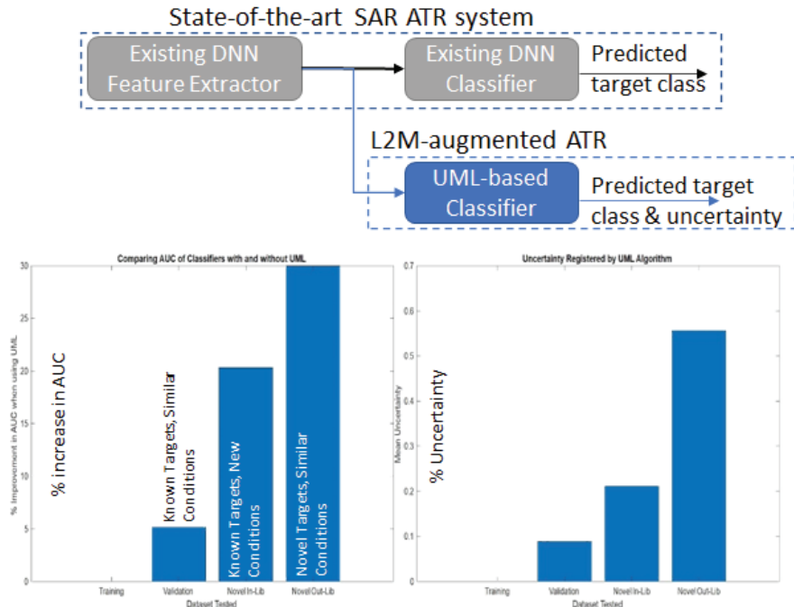
Figure 11. UML Improves Performance of a State-of-the-Art SAR-Based ATR Algorithm in Novel (Out-of-Nominal) Conditions
