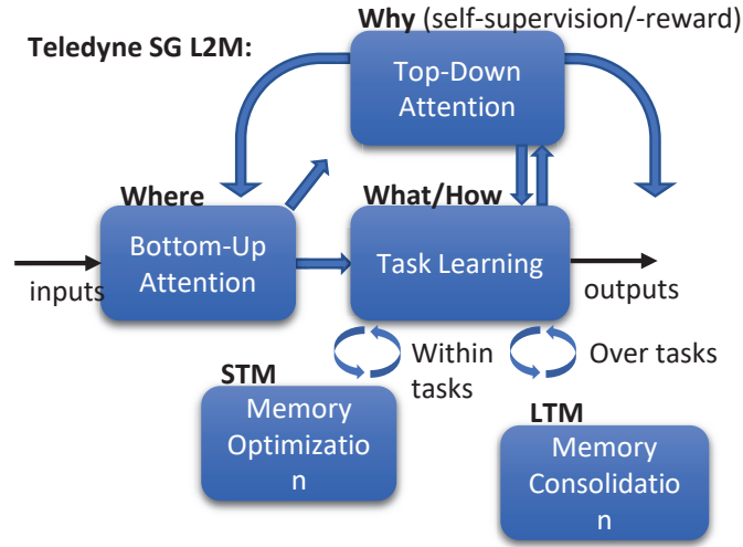
Figure 8. Functional Blocks of the Teledyne SG Integrated System
