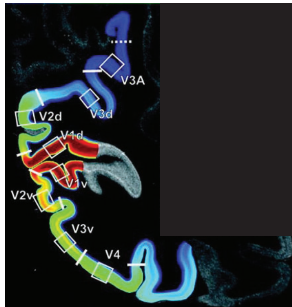
Figure 6. Gradient of Muscarinic Receptor Distribution in Visual Brain Areas
