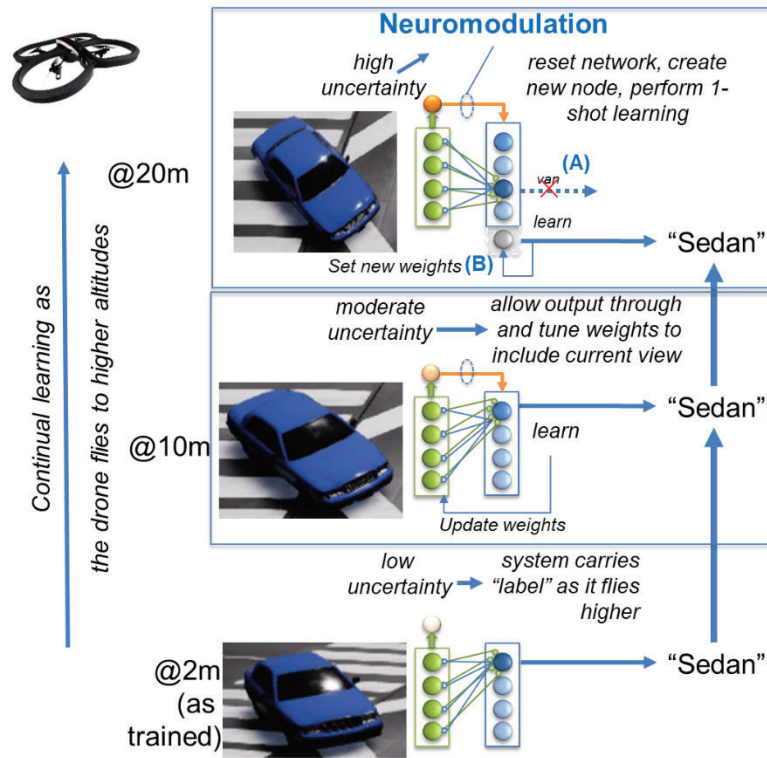
Figure 17. Self-Supervised Learning of a New Object
