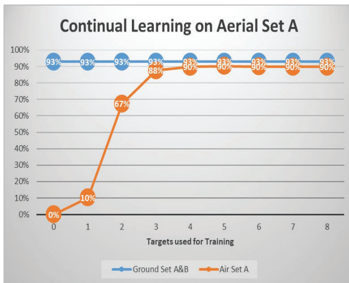
Figure 20. Proof of Concept 1 Results
