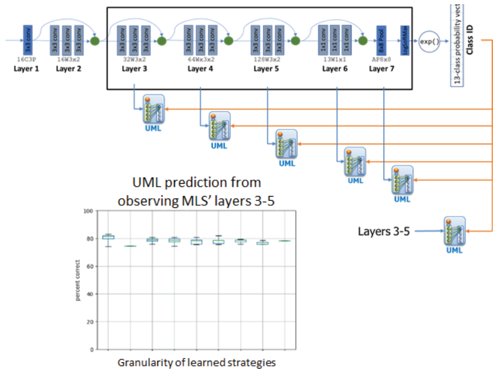
Figure 12. UML Applied to Predict Performance of an Existing Machine Learning Algorithm
