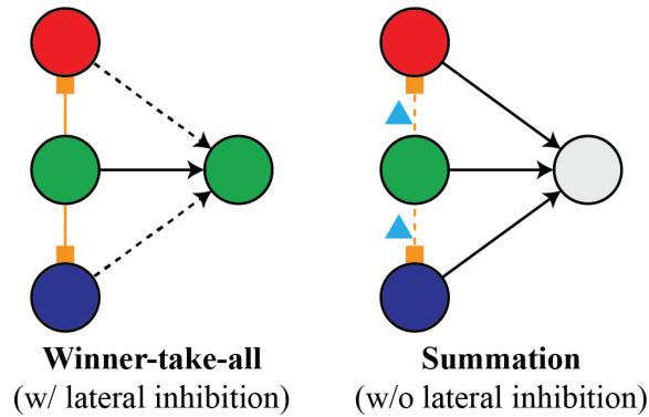
Figure 9. Neuromodulation Enables Neural Circuits to Quickly and Temporarily Change Their Dynamics
