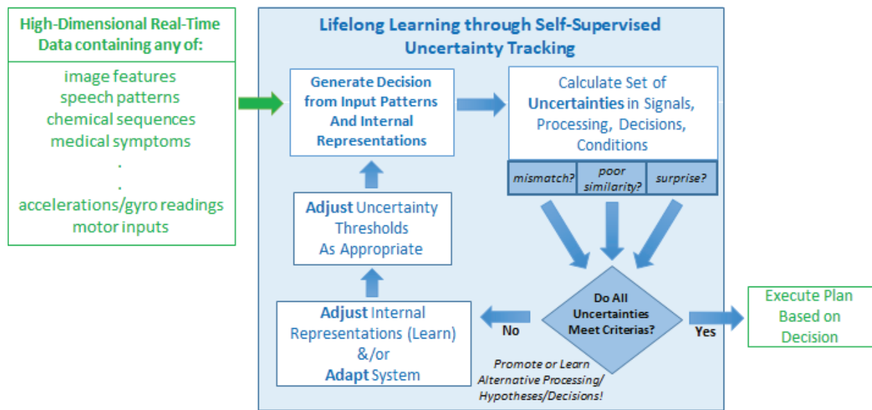
Figure 15. Generalized Algorithm for the Uncertainty-Modulated Architecture
