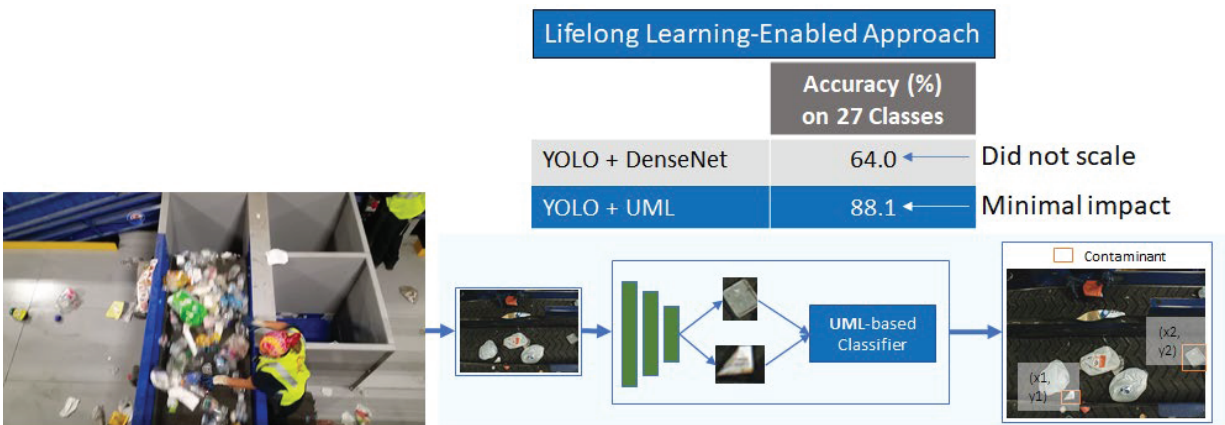
Figure 13. UML Applied to Classify Objects in Complex Environments Outperforms State-of-the-Art Object Classifiers
