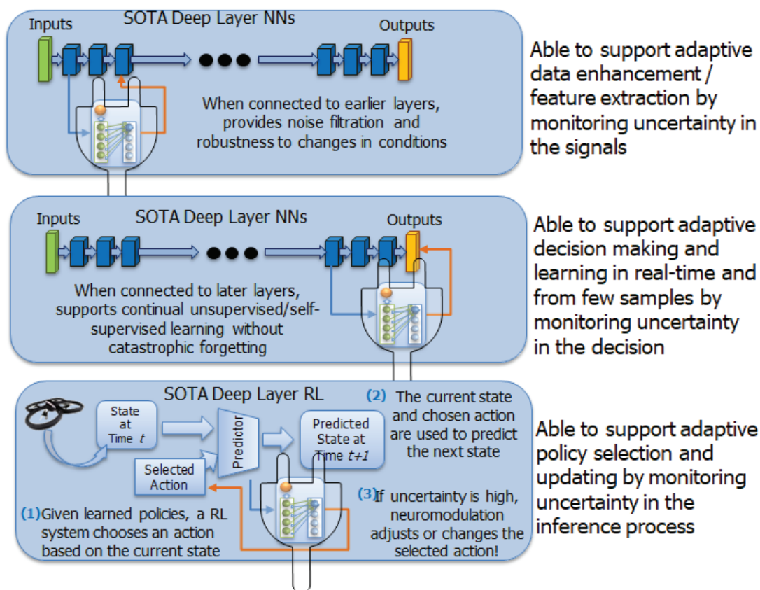
Figure 36. UML is a Pluggable Component that can Support Lifelong Learning Capabilities in State-of-the-Art Machine Learning Systems
