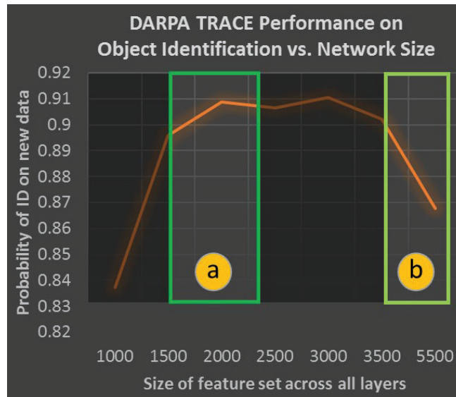
Figure 2. Deep Learning Scaling Limit
