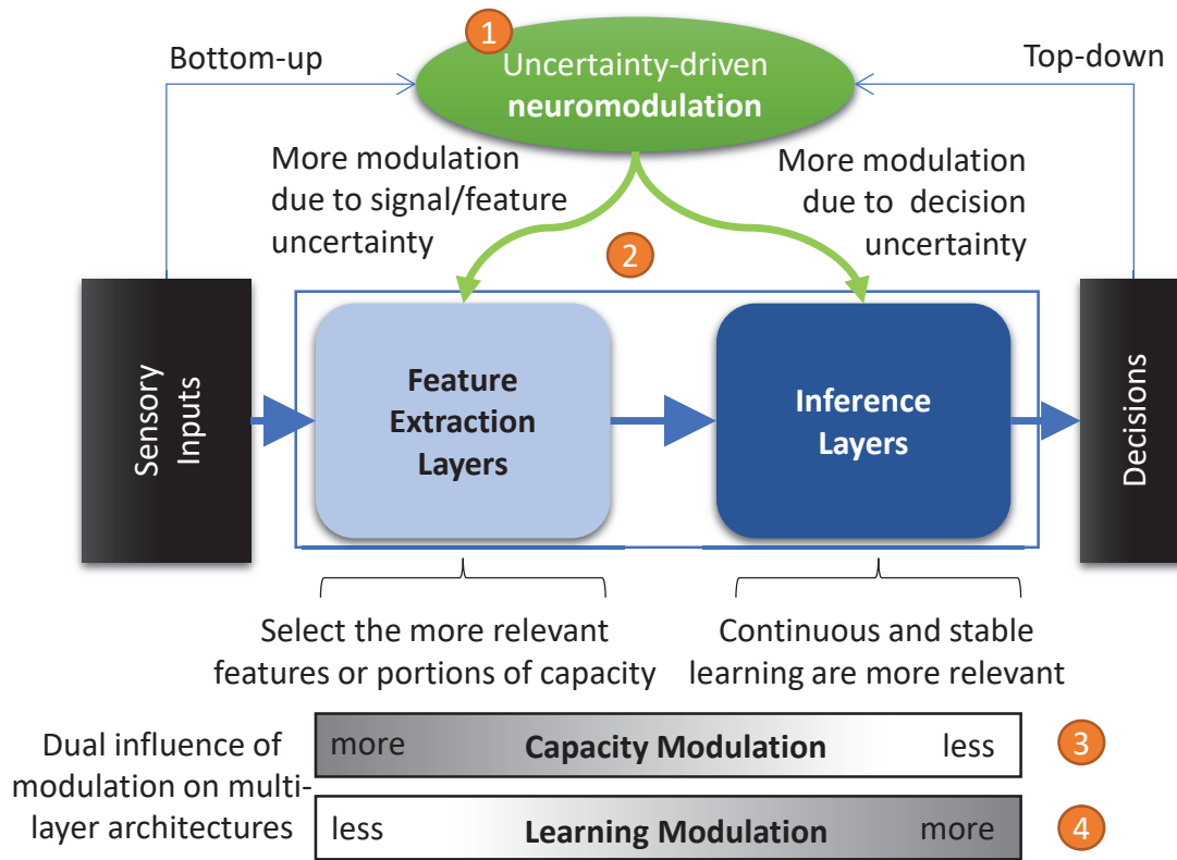
Figure 1. Architectures for Selective Plasticity in Hierarchical Machine Learning Systems
