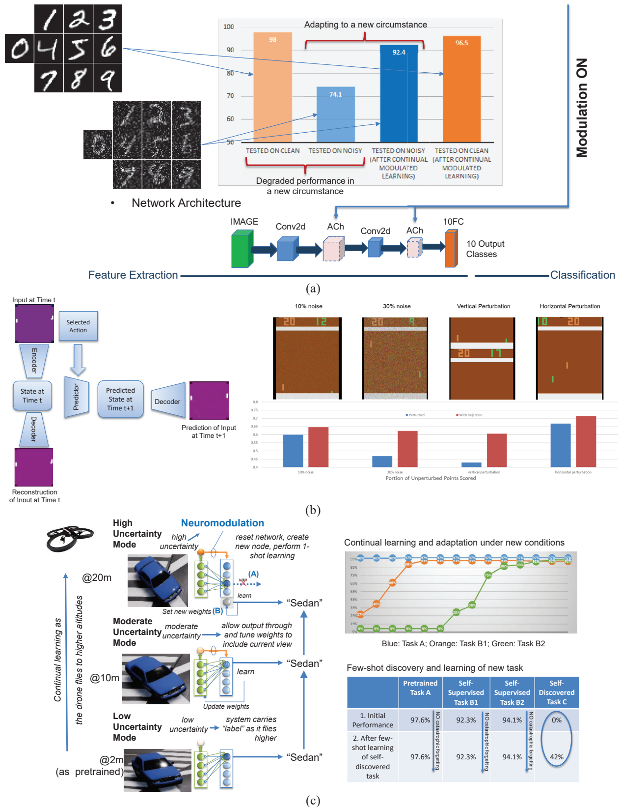
Figure 10. Application of UML to a Variety of Machine Learning Problems
