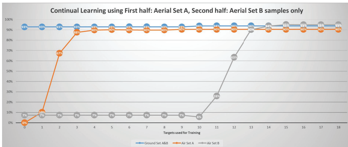
Figure 21. Proof of Concept 2 Results
