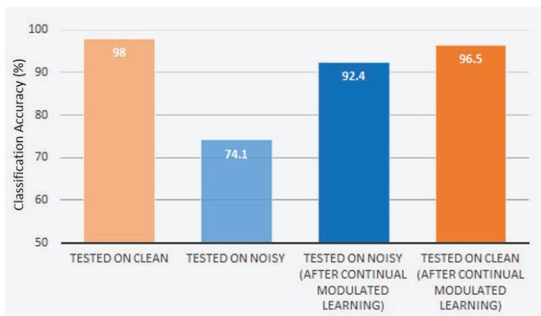
Figure 34. Continual Modulated Learning with Noisy Imagery
