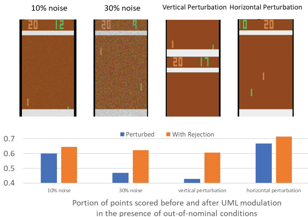
Figure 35. Noise Rejection in Reinforcement Learning
