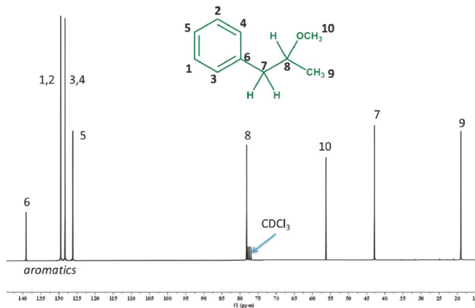
Figure 4. Carbon ( ^{13}\text{C} ) NMR spectrum of (2-methoxy)propyl benzene in \text{CDCl}_3 .
