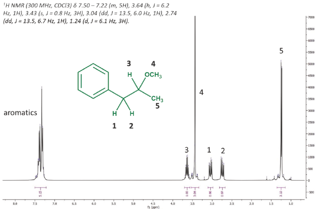
Figure 3. Proton ( ^1\text{H} ) NMR spectrum of (2-methoxy)propyl benzene in \text{CDCl}_3 .
