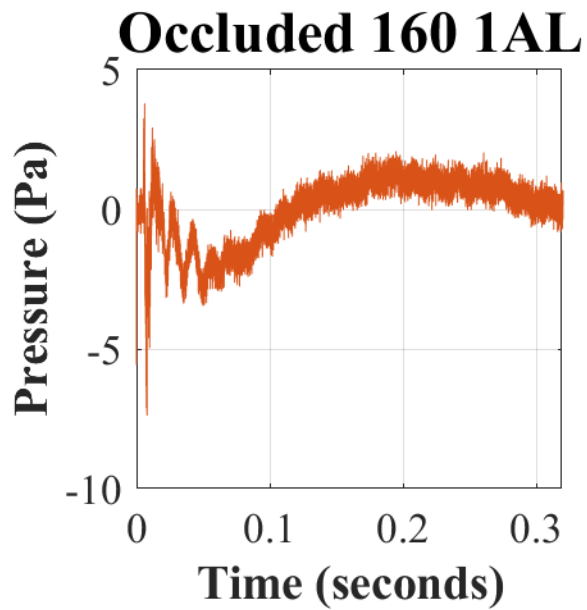
Appendix G. Recorded occluded (closed-ear) waveforms (in pascals [Pa]) over time (in seconds [s]) in response to 160 dBp with the ComTac™ III (MAX).
