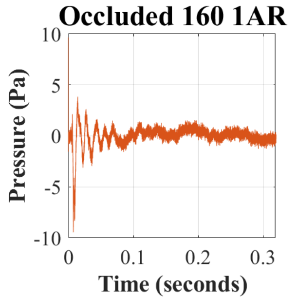
Appendix G. Recorded occluded (closed-ear) waveforms (in pascals [Pa]) over time (in seconds [s]) in response to 160 dBp with the ComTac™ III (MAX).
