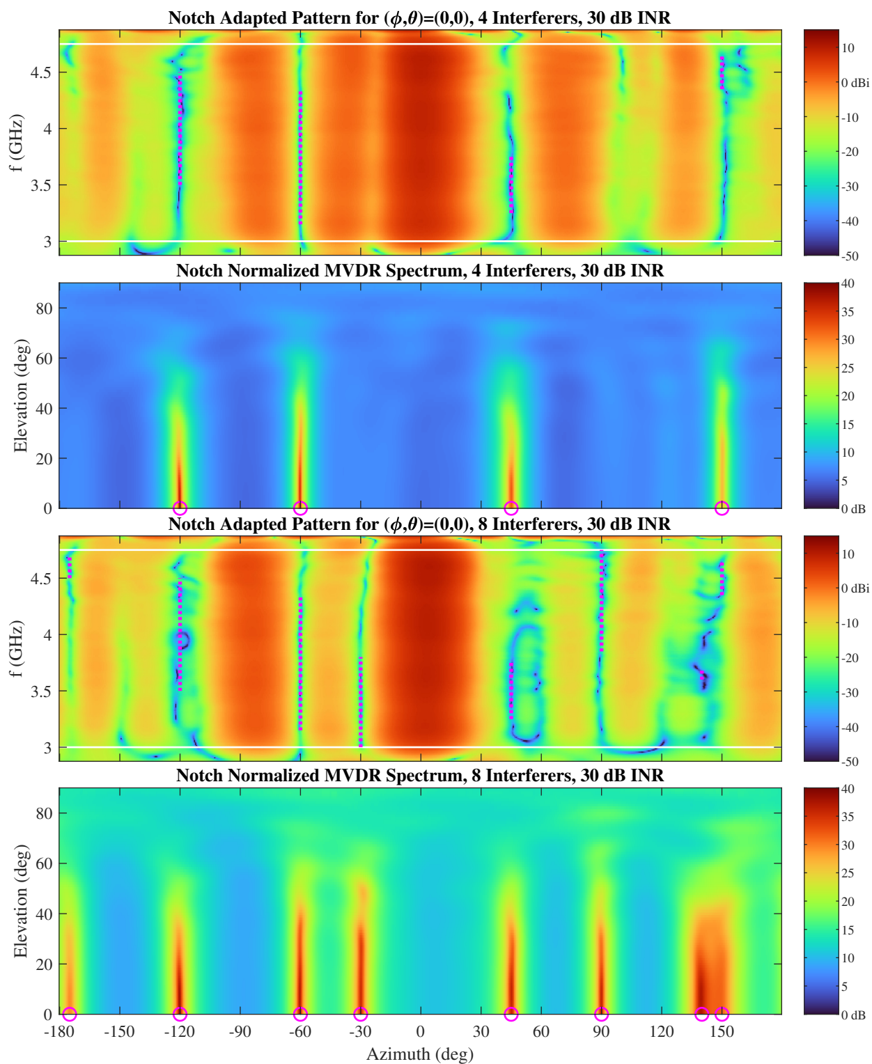
Fig. 46—Adaptive array patterns and normalized MVDR spectra for the notch array in the presense of noise and multiple interference sources. In the top two plots, four interference sources are present, versus eight in the bottom two plots.
