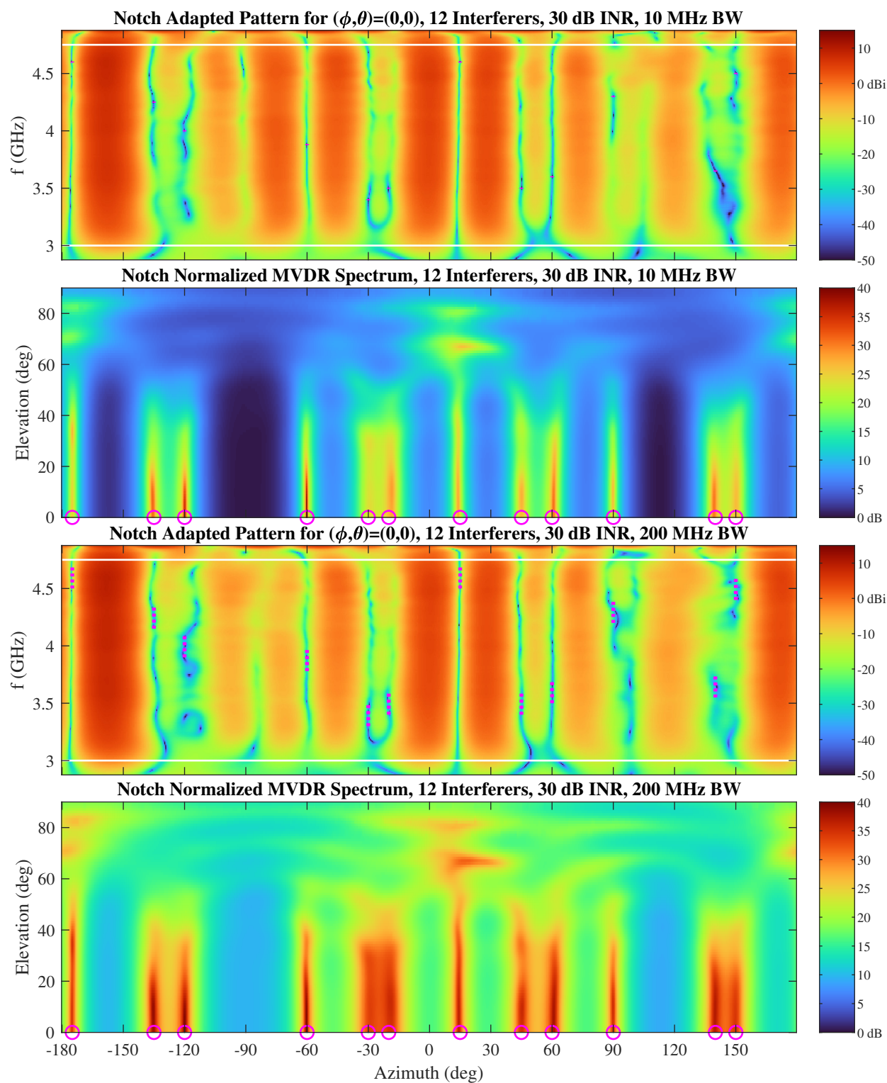
Fig. 48—Adaptive array patterns and normalized MVDR spectra for the notch array in the presense of noise and 12 interference sources. In the top two plots, the interference bandwidth is 10 MHz, versus 200 MHz in the bottom two plots.
