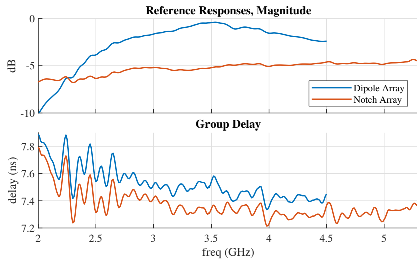
Fig. 28—The reference (mode 0) frequency responses for the two arrays
