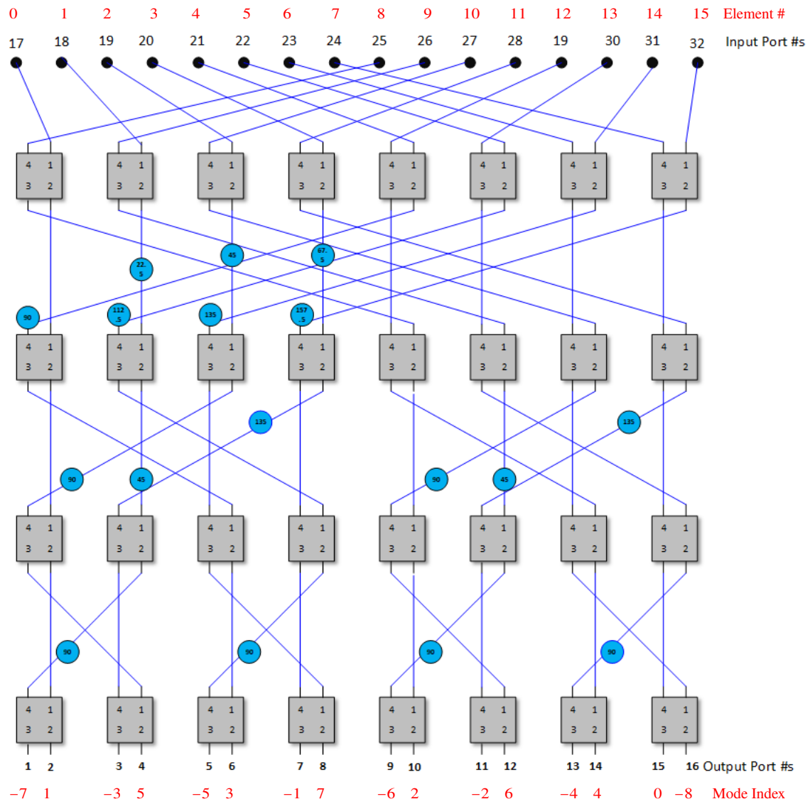
Fig. 19—16 × 16 Butler matrix layout. The boxes are 90° hybrids and the circles are phase shifters. The red labels at top and bottom give the element index and mode index, respectively, that correspond to the port numbers (in black).
