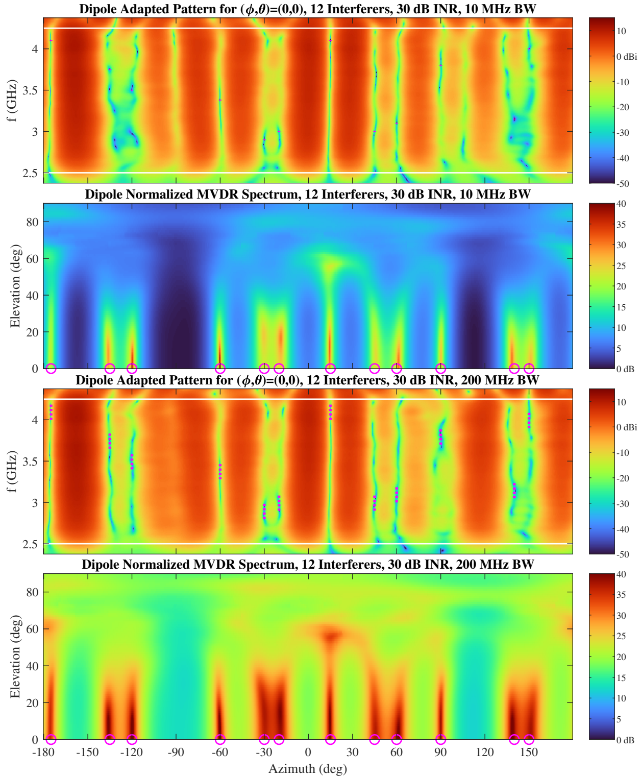
Fig. 47—Adaptive array patterns and normalized MVDR spectra for the dipole array in the presense of noise and 12 interference sources. In the top two plots, the interference bandwidth is 10 MHz, versus 200 MHz in the bottom two plots.
