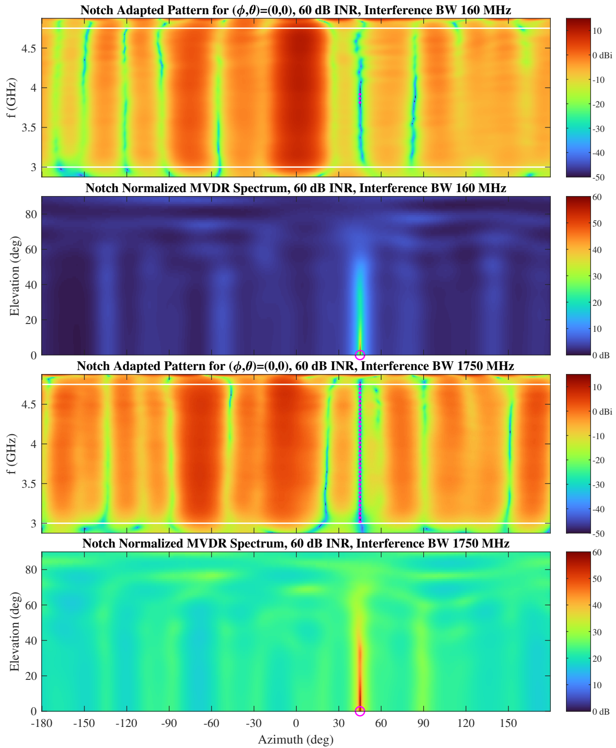
Fig. 44—Adaptive array patterns and normalized MVDR spectra for the notch array in the presense of noise and a single strong interference source. In the top two plots, the interference has a modest bandwidth, while in the bottom two plots, the interference occupies the entire equalized band.
