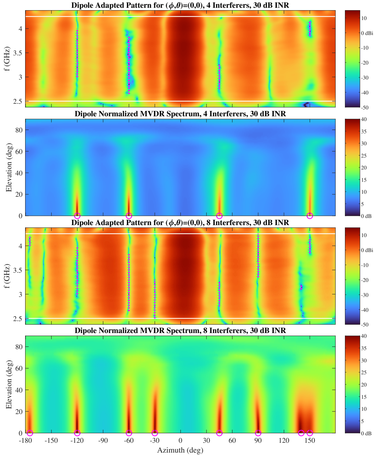
Fig. 45—Adaptive array patterns and normalized MVDR spectra for the dipole array in the presense of noise and multiple interference sources. In the top two plots, four interference sources are present, versus eight in the bottom two plots.
