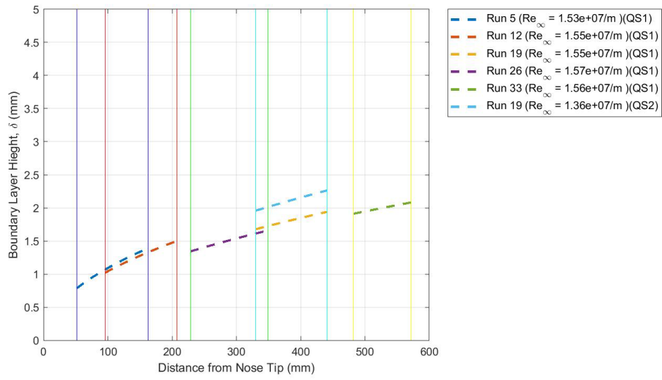
Figure 57: Laminar Boundary Layer Thickness for Uncooled Experiments at P_{DT} = 300 psi, T_w/T_0 = 0.59 ( T_w/T_c = 4.35 \pm 0.15 )
