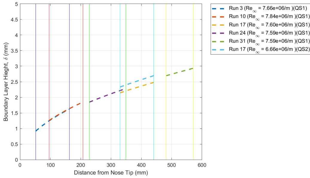
Figure 55: Laminar Boundary Layer Thickness for Uncooled Experiments at P_{DT} = 150 psi, T_w/T_0 = 0.59 ( T_w/T_c = 4.35 \pm 0.15 )
