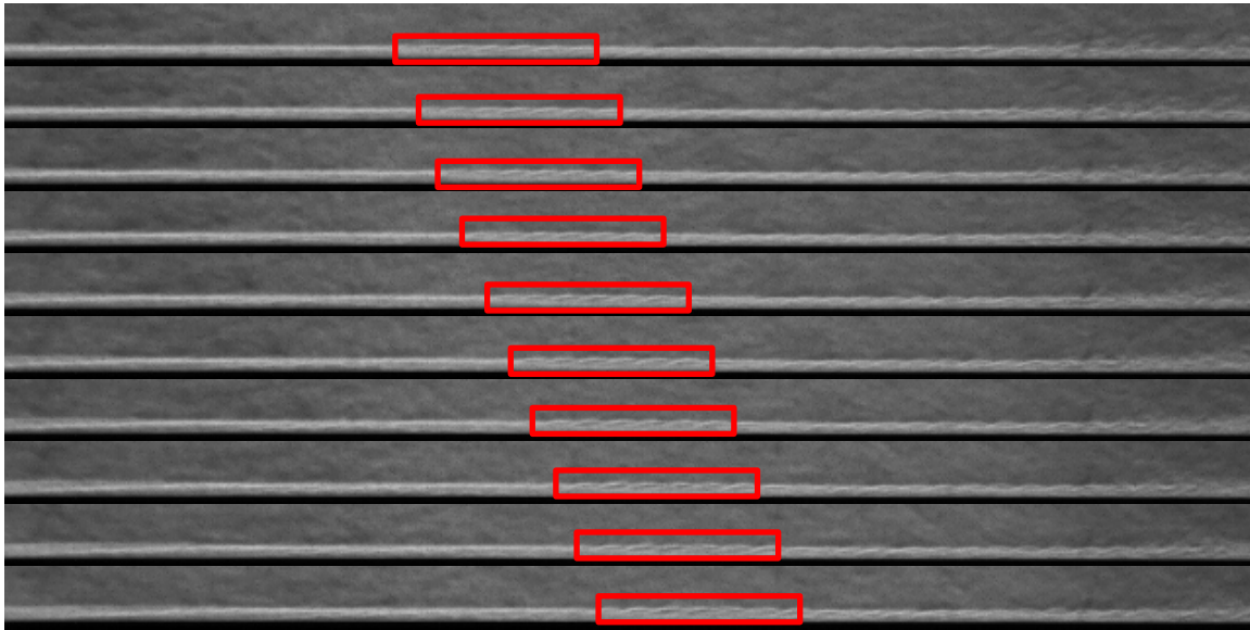
Figure 42: Mack's Second Mode Instabilities (Red Boxes) Flowing (From Left-to-Right) into Turbulence Transition Onset for Uncooled Run 27 ( x=229\text{-}349\text{ mm} ), P_{DT} = 400\text{ psia}
