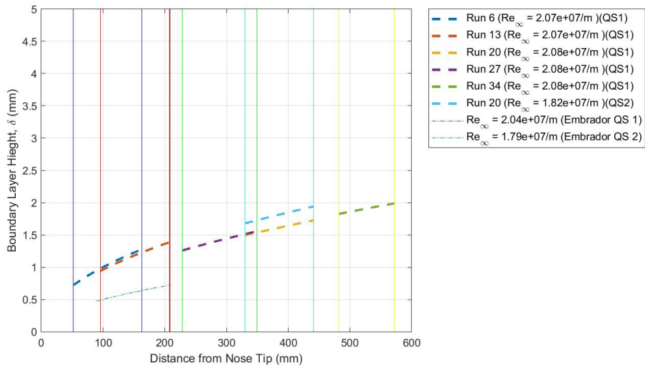
Figure 58: Laminar Boundary Layer Thickness for Uncooled Experiments at P_{DT} = 400 psi, T_w/T_0 = 0.59 ( T_w/T_c = 4.35 \pm 0.15 )
