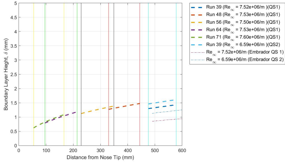
Figure 62: Laminar Boundary Layer Thickness for Cooled Experiments at P_{DT} = 150 psi, T_w/T_0 = .19 ( T_w/T_c = 1.40 \pm 0.05 )
