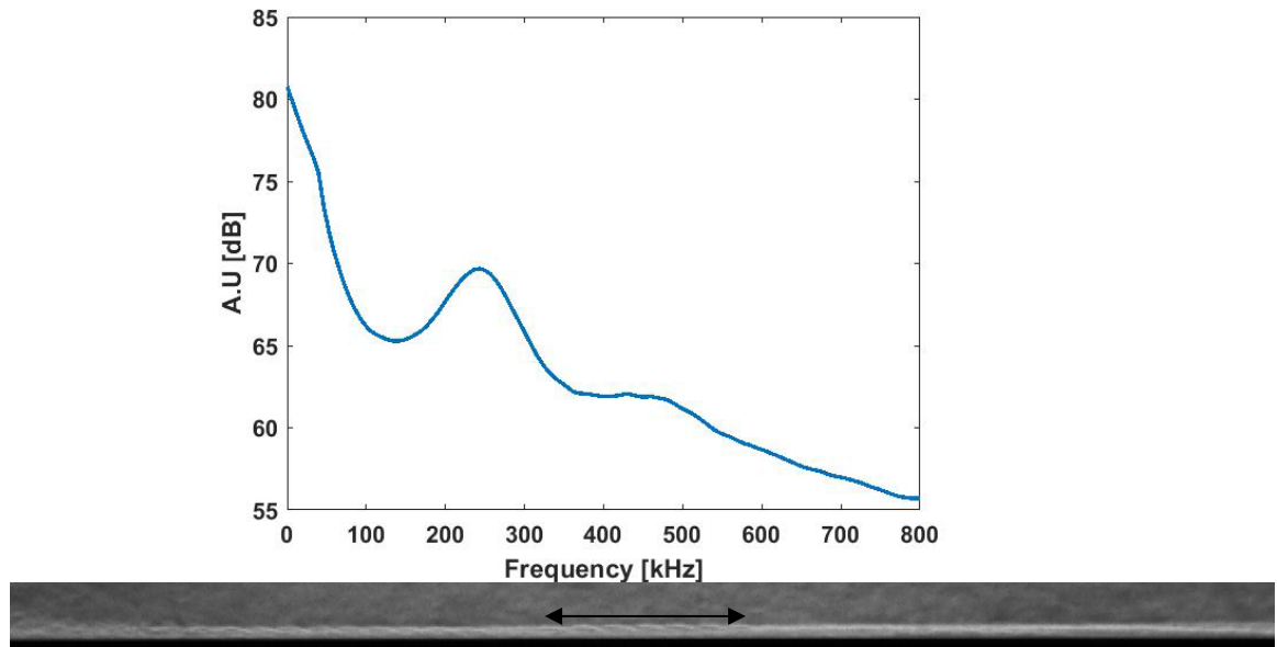
c) PSD plot for Uncooled Run 27 ( x=229-349 mm) QS1 Second Mode, P_{DT} = 400 psia, peak frequency = 243 kHz
