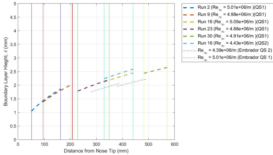
Figure 54: Laminar Boundary Layer Thickness for Uncooled Experiments at P_{DT} = 100 psi, T_w/T_0 = .59 ( T_w/T_e = 4.35 \pm 0.15 )
