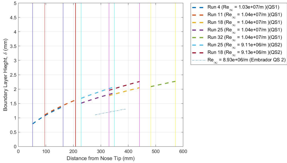
Figure 56: Laminar Boundary Layer Thickness for Uncooled Experiments at P_{DT} = 200 psi, T_w/T_0 = 0.59 ( T_w/T_c = 4.35 \pm 0.15 )
