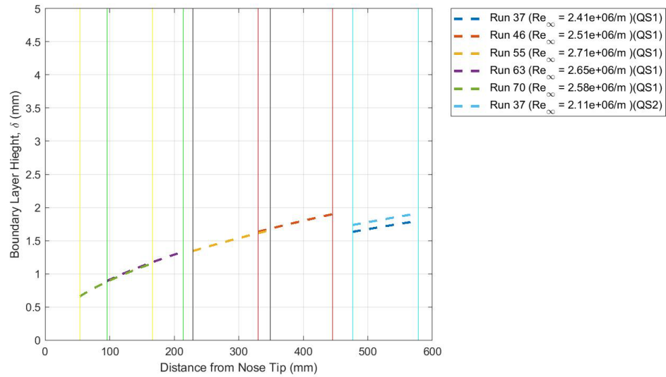
Figure 60: Laminar Boundary Layer Thickness for Uncooled Experiments at P_{DT} = 50 psi, T_w/T_0 = 0.19 ( T_w/T_c = 1.40 \pm 0.05 )
