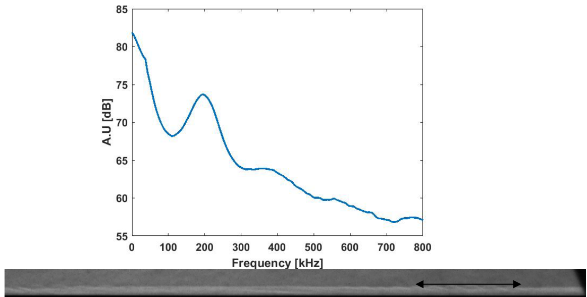
d) PSD plot for Uncooled Run 18 ( x=330-441 mm) QS2 Second Mode, P_{DT} = 200 psia, peak frequency = 195 kHz
