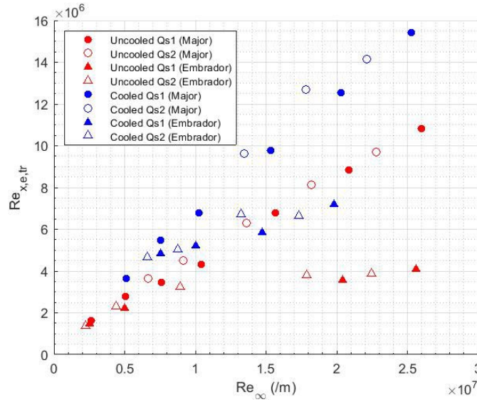
Figure 38: Transition Reynolds Number at the Boundary Layer Edge with Varying Freestream Unit Reynolds Number, Cooled ( T_w/T_0 = .19 ) and Uncooled ( T_w/T_0 = .59 ) Experiments for Both Sharp-Tipped (Embrador) and Blunt-Tipped (Major) Results
