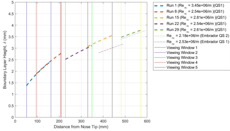
Figure 53: Laminar Boundary Layer Thickness for Uncooled Experiments at P_{DT} = 50 psi, T_w/T_0 = .59 ( T_w/T_e = 4.35 \pm 0.15 )
