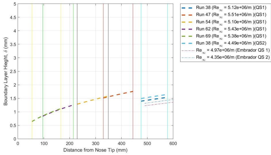
Figure 61: Laminar Boundary Layer Thickness for Cooled Experiments at P_{DT} = 100 psi, T_w/T_0 = .19 ( T_w/T_c = 1.40 \pm 0.05 )
