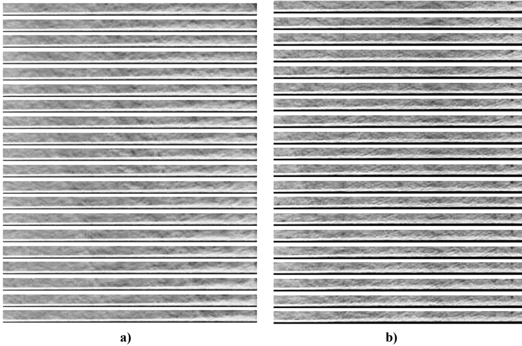
Figure 36: Qualitative Comparison Between Turbulence Intermittency Discontinuity, 20 Sequential Schlieren Images, P_{DT} = 300 psi Cooled (Target: T_w/T_e = 1.40 \pm 0.05 ) QS1 at a) Run 41 ( x=476-578 mm) and b) Run 50 ( x=330-445 mm)
