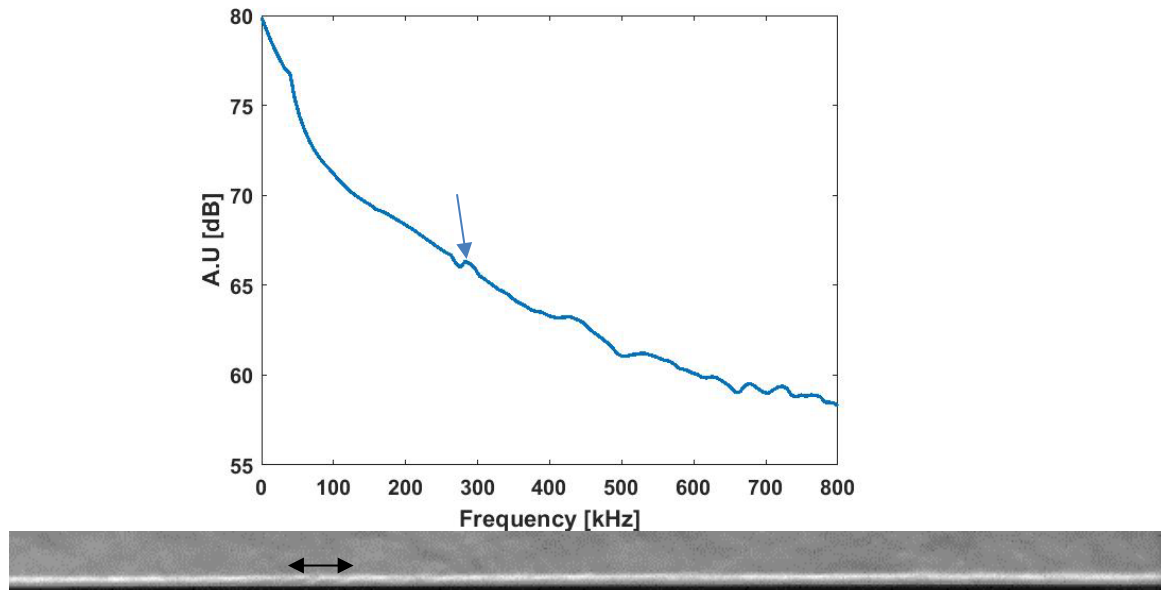
g) PSD plot for Cooled Run 40 ( x=476-578 mm) QS1 Second Mode, P_{DT} = 200 psia, peak frequency = 289 kHz
