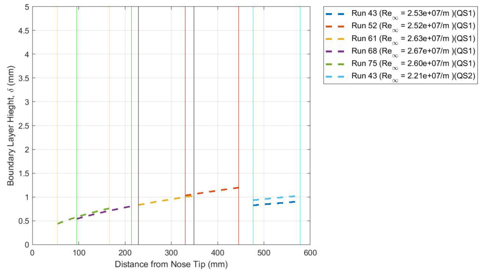
Figure 66: Laminar Boundary Layer Thickness for Cooled Experiments at P_{DT} = 500 psi, T_w/T_0 = .19 ( T_w/T_c = 1.40 \pm 0.05 )
