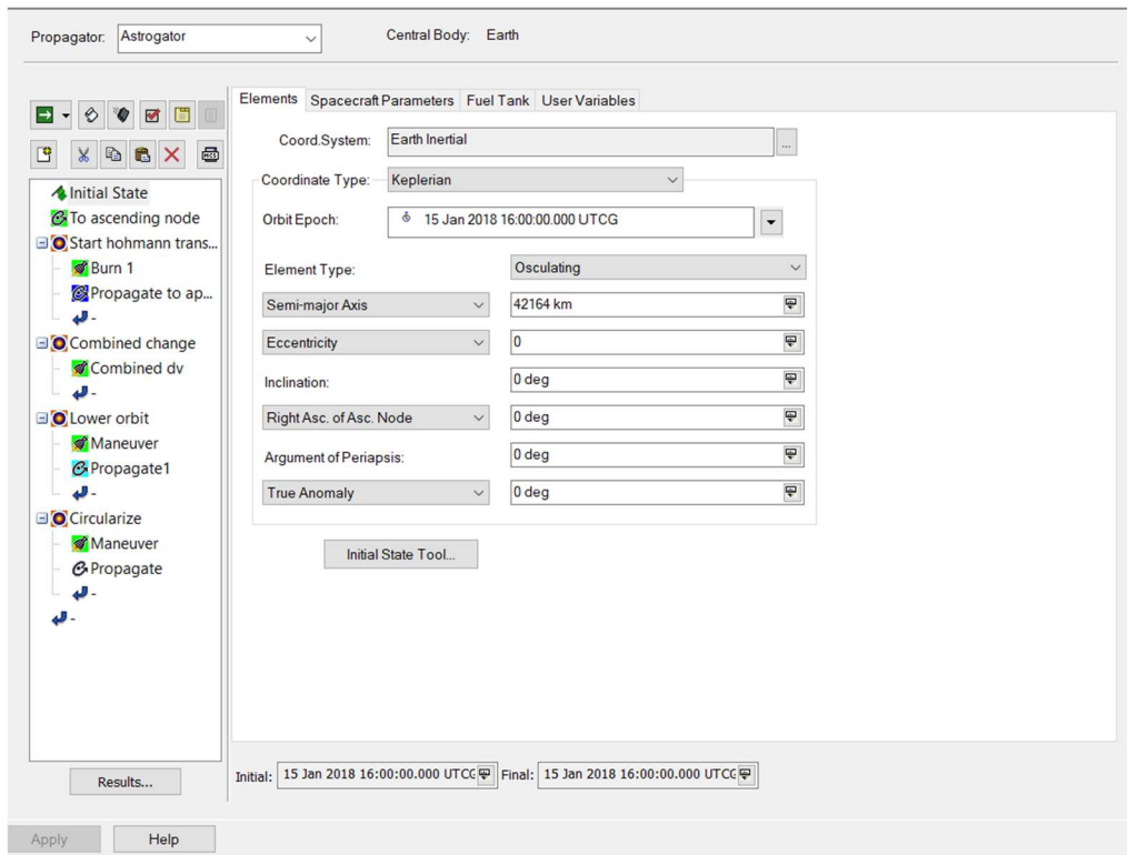
Figure 21: Targeting profile of inclination change using Hohmann transfer to a greater radius of GEO. Modified strategy from STK tutorial.
