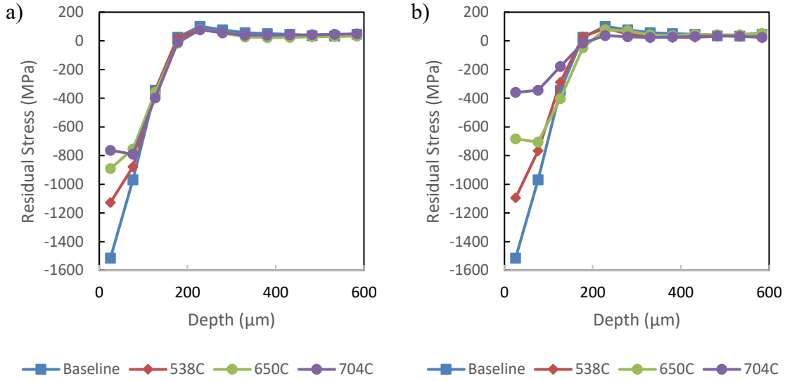
Figure 22 Residual stress profile after a) 1 hour and b) 100 hours
