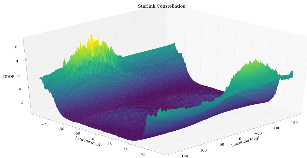
Figure 4.4. GDOP vs. Latitude/Longitude for Starlink Constellation
