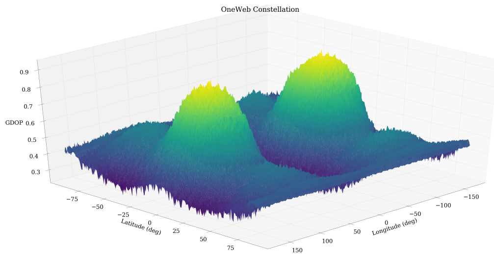
Figure 4.3. GDOP vs. Latitude/Longitude for OneWeb Constellation
