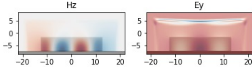
Figure 24: Relative normalized field strength of H_z and E_y based on the H_z Gaussian excitation at 1.3 GHz. The material properties used are \epsilon = 3 and \mu = 36.05 . The expected TE 01 excitation is achieved and shown by the dark red region in middle of the E_y field.
