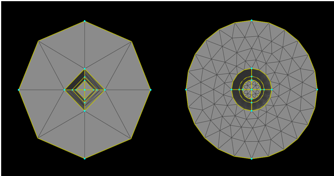
(a) Mesh structure with a 2.1 mm mesh sizing. (b) Mesh structure with a 0.25 mm mesh sizing. Would not support a Transverse Electric wave in this coax. This would support a TEM wave in the Magnetic (TEM) wave in this coax.
