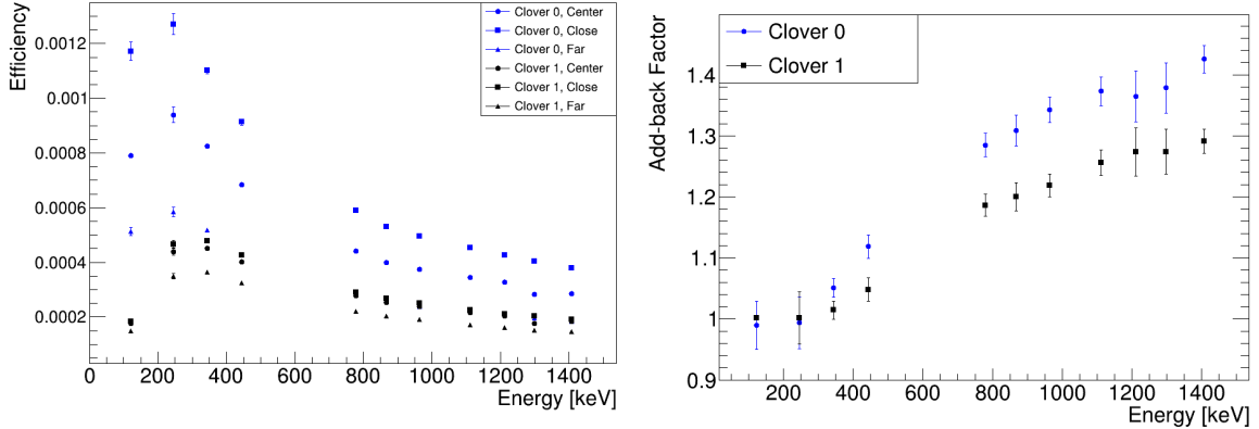
(a) Gamma efficiency for Clover 0 (at 90^\circ ) and Clover 1 (at 54^\circ ) measured with a 0.916 \mu\text{Ci } ^{152}\text{Eu} at the target location and 1" closer and away from Clover 0. The results are the total of each leaf in the clover, but does not include add-back.
