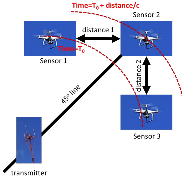
Figure 6. Scenario where TDOA cannot be used to find the target location
