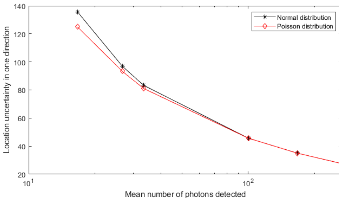
Figure D-9. Uncertainty in location caused by the uncertainty in using photon detector sensors to find the emitter location as a function of the mean number of photons the detector would measure
