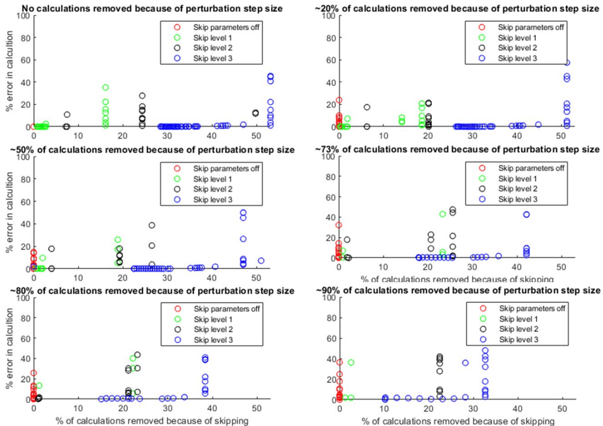
Figure C-2. Accuracy in the TLE estimation drops as the algorithm speeds up calculation time by not performing as many calculations
