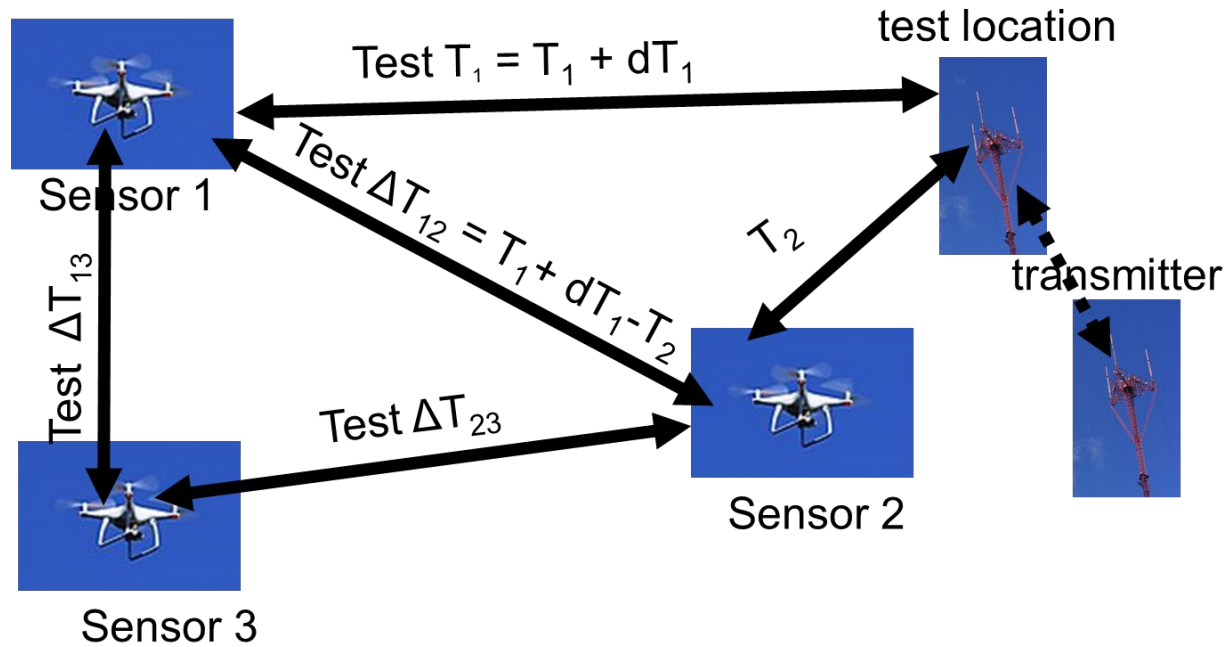
Figure 3. Example showing how to determine the error in finding the emitter location if a perturbation is added to the time of arrival SIGINT system as measured by Sensor 1
