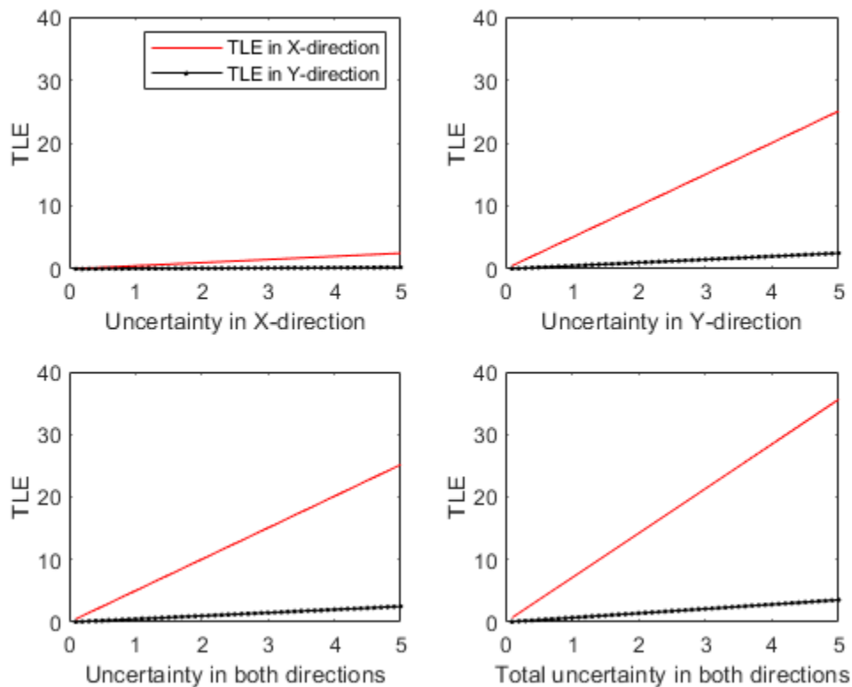
Figure D-6. Various results from the test for the scenario shown in Figure D-5
