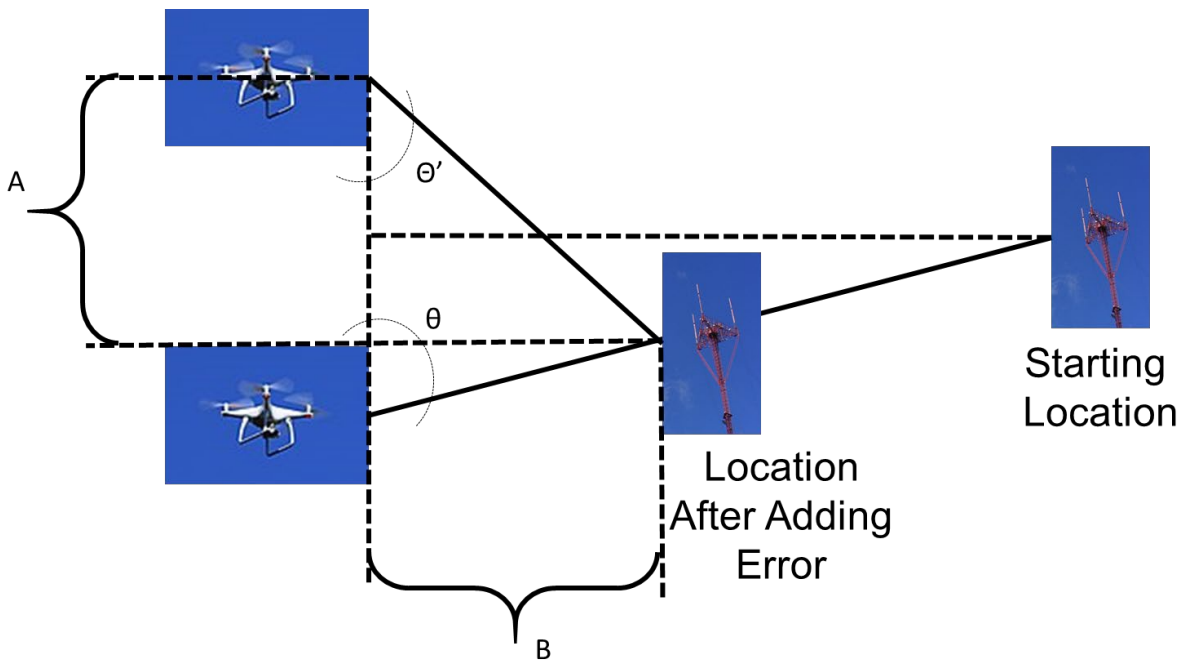
Figure D-8. Error in the measured emitter location after adding an error to the angle measured by one sensor
