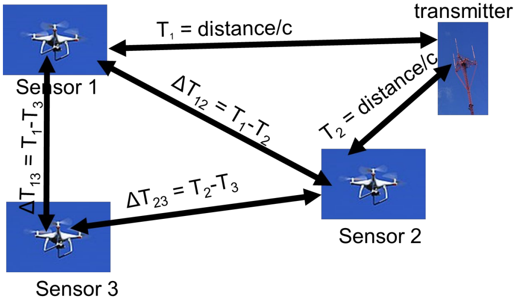
Figure 1. Geometry showing how to find the time difference for each sensor if the location of the emitter is known and the sensor is a SIGINT system using TDOA
