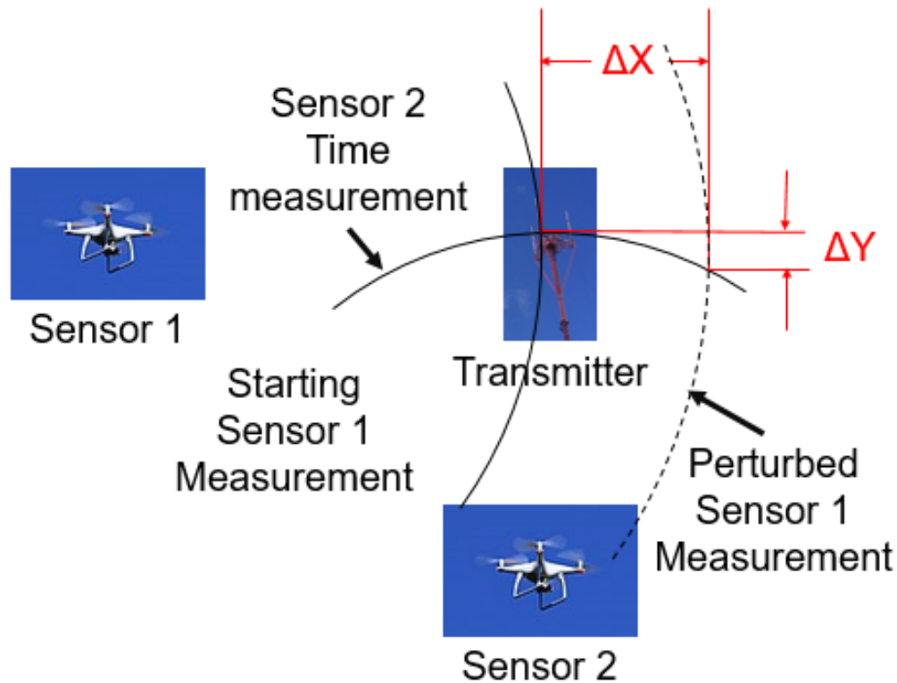
Figure D-3. Perturbation in time measurement for one sensor can add a TLE in both directions
