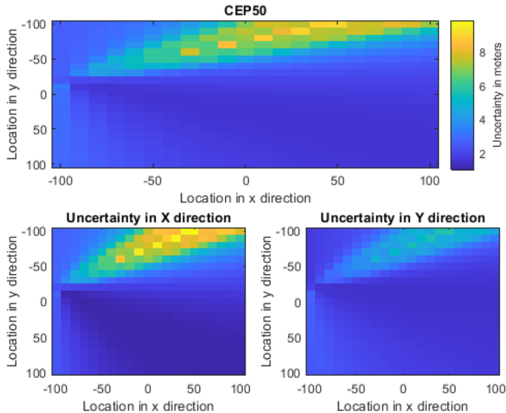
Figure 8. TLE in the X- and Y-directions along with CEP50 for the sample experiment at several locations
