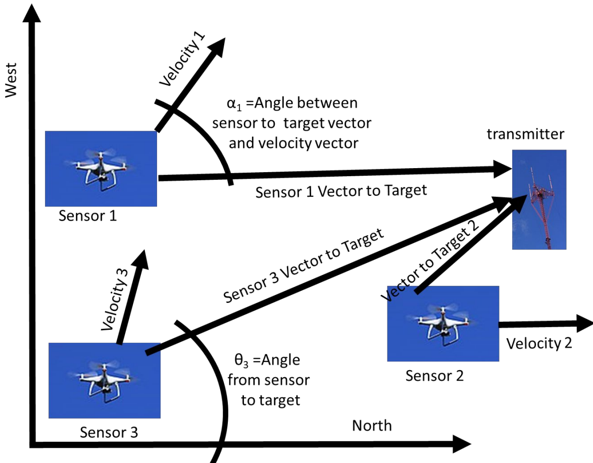
Figure 2. Geometry showing how to find the angles needed to model EO/IR, FDOA SIGINT, and AOA SIGINT when the location of the emitter is known
