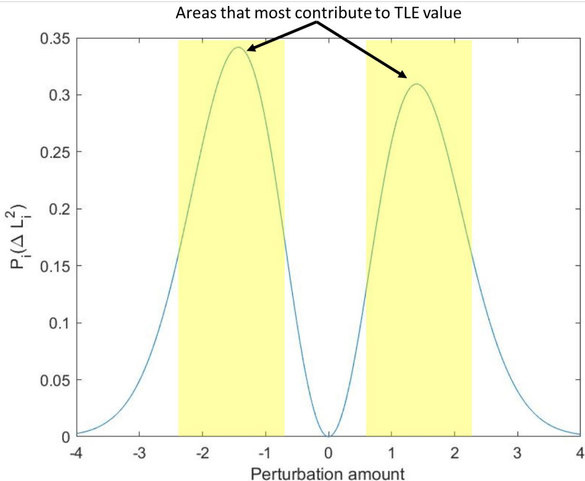
Figure C-1. Perturbation values that contribute most to the final TLE value
