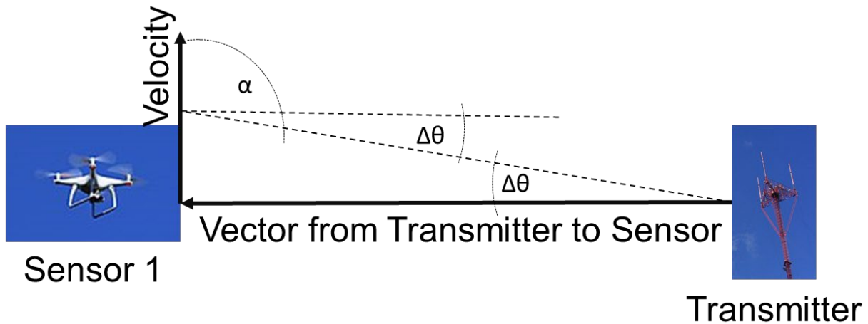
Figure D-2. Geometry when adding an uncertainty in azimuth angle to the test FDOA setup
