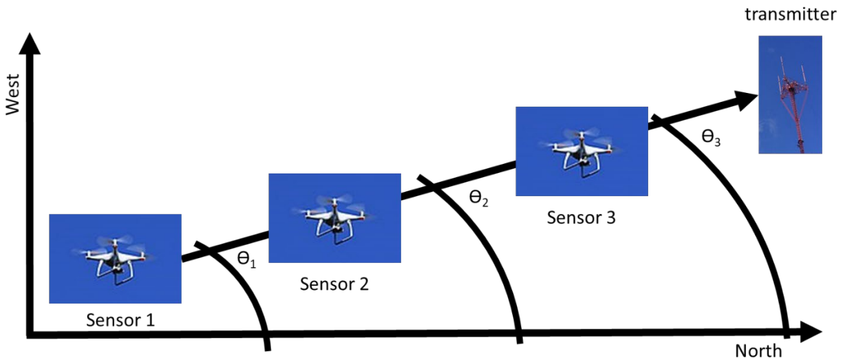
Figure 5. Configuration in which a SIGINT AOA cannot be used to find an RF emitter
