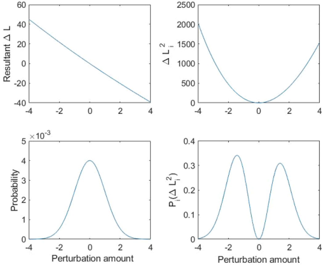
Figure 4. Example values used to find the uncertainty of the target of interest's location in a single direction caused by an uncertainty in knowing the value of a single variable
