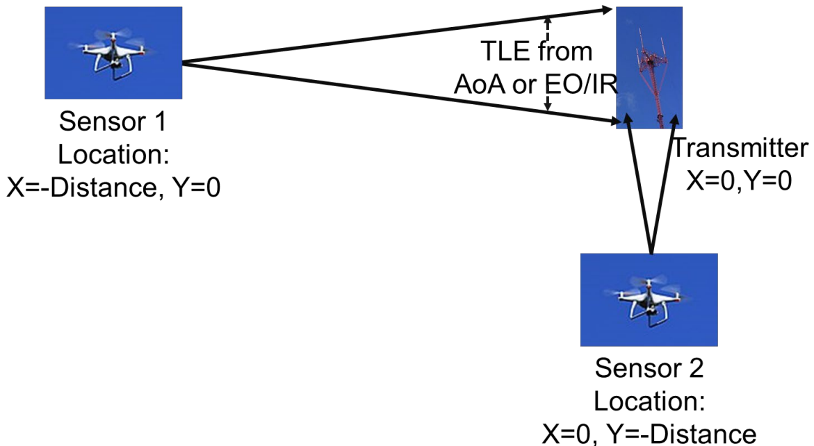
Figure D-1. Experimental setup where the uncertainty in one direction is only caused by a measurement uncertainty of a single sensor
