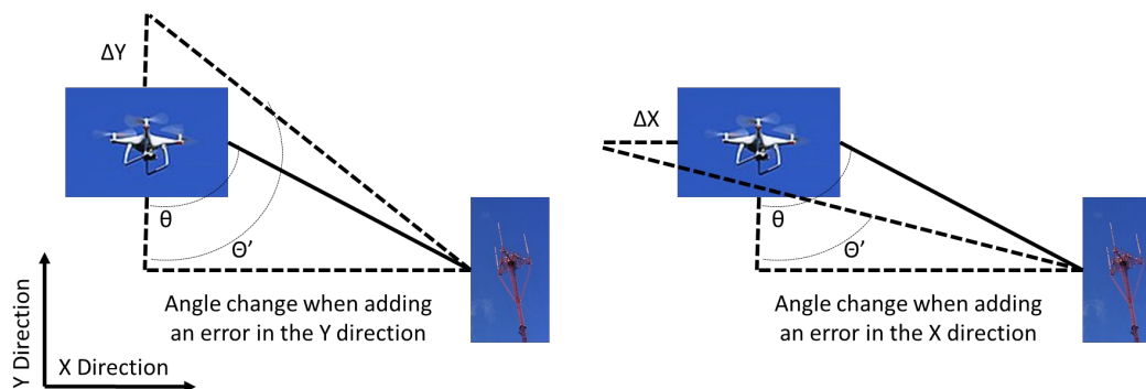
Figure D-7. Angle changes as errors are added in the X- and Y-directions to the sensor location
