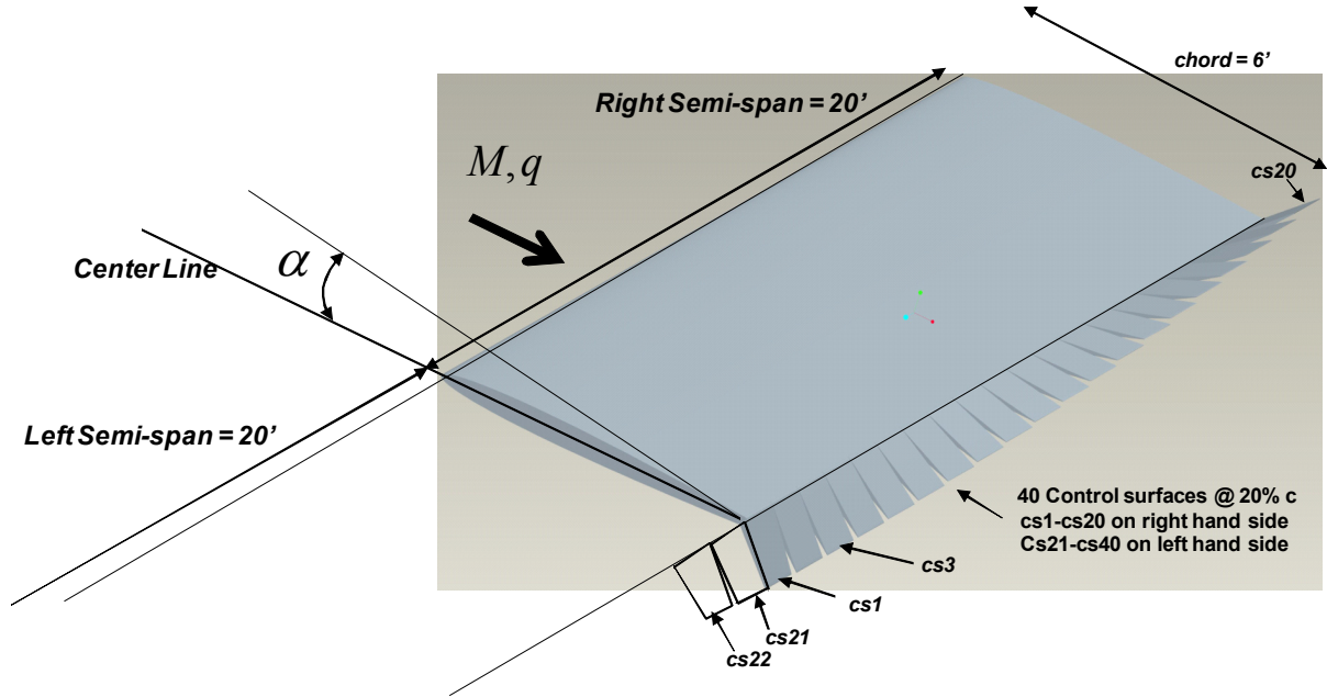
Figure 3. Golang Wing Aerodynamic Configuration
