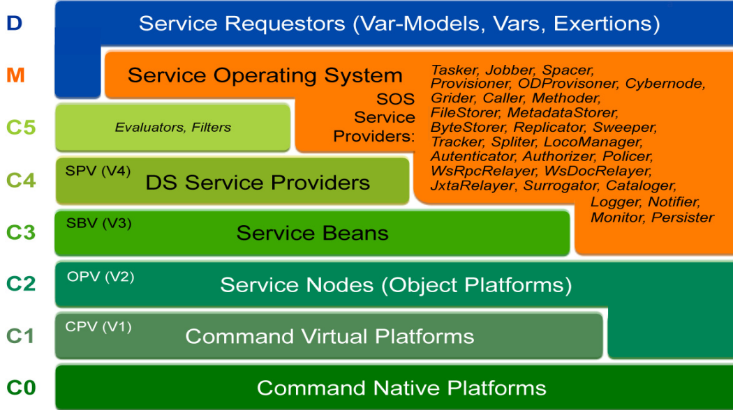
Figure 1. The SORCER layered architecture, where C0C5 (carrier)—the metaprocessor with its service cloud at C4 and C3, platform cloud at C2 and C1, M (management)—SORCER operating system, D (domain)—service requestors; where V1V4 stands virtualization of the corresponding layer
