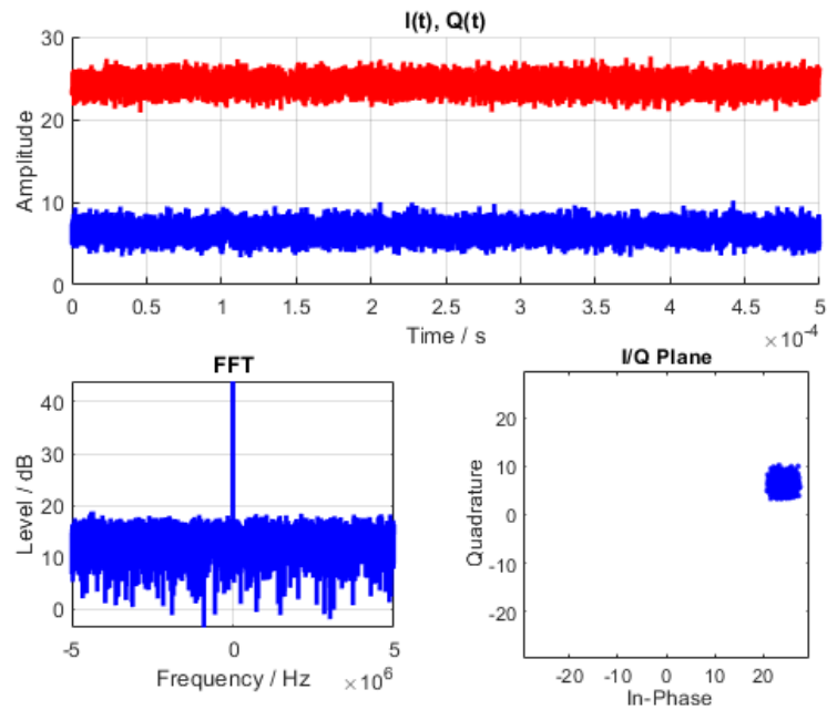
Figure 4.1. Producing pulsed radar embedded communications .wv file for physical signal generation.
