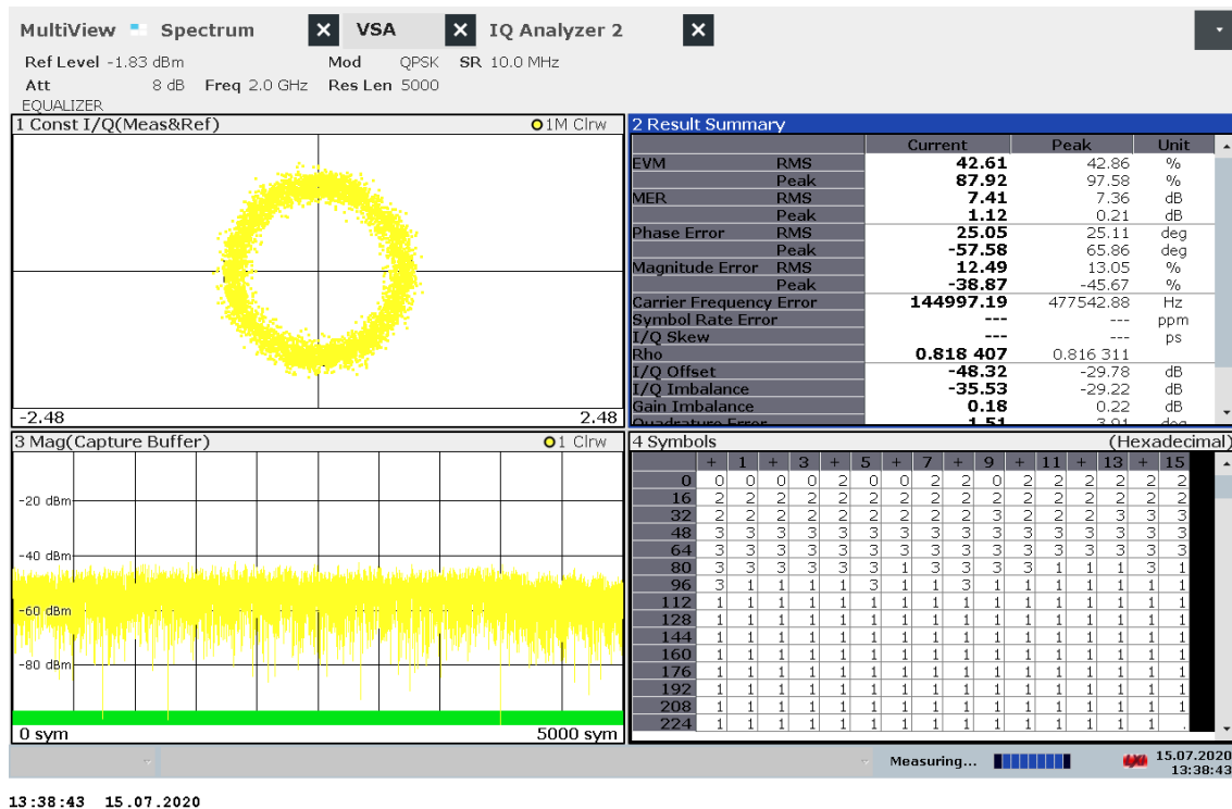
Figure 4.12. Multiview screenshot of the receiving SpecAn on LFM radar embedded communications
