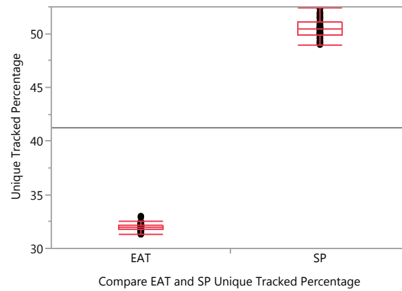
Figure 10 Unique-Track Percentage Box Plot: The plot presents the difference in data sets where the EAT performs better.
