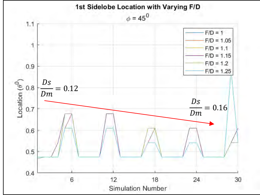
Figure 51. First sidelobe location with varying F/D ratios over the search area for the offset fed Cassegrain; \phi = 45^0 .
