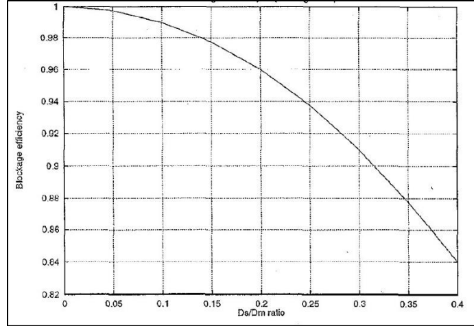
Figure 14. Relationship between D_s/D_m and the blockage efficiency for the axially fed Cassegrain antenna [3].
