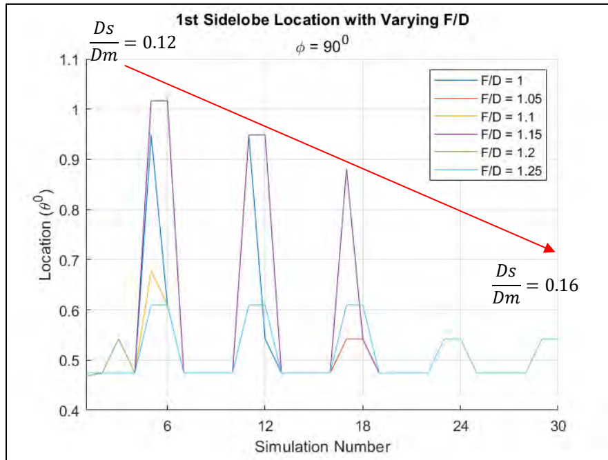
Figure 52. First sidelobe location with varying F/D ratios over the search area for the offset fed Cassegrain; \phi = 90^0 .
