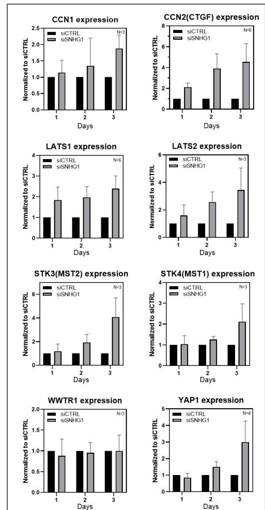
Figure 4: Expression of hippo pathway gene mRNA following SNHG1 knockdown in PC3 cells. Mean \pm SD.
