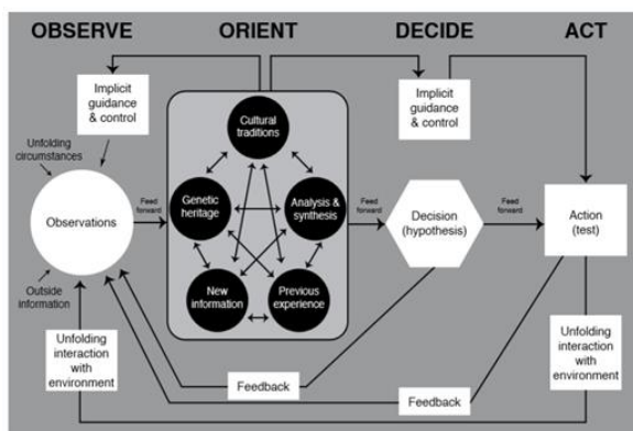
Figure 7: OODA Loop
