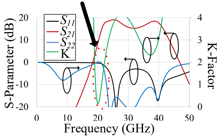
Figure 5.2: S-parameter EM PEX Simulations with V_{DD} = 6 V, Highlighting the Mismatch of the Broadband GaN Class J PA from the first GaN tapeout that Shows a Big Dip in Stability at ~20 GHz, Similar to what was Observed in Measurement
