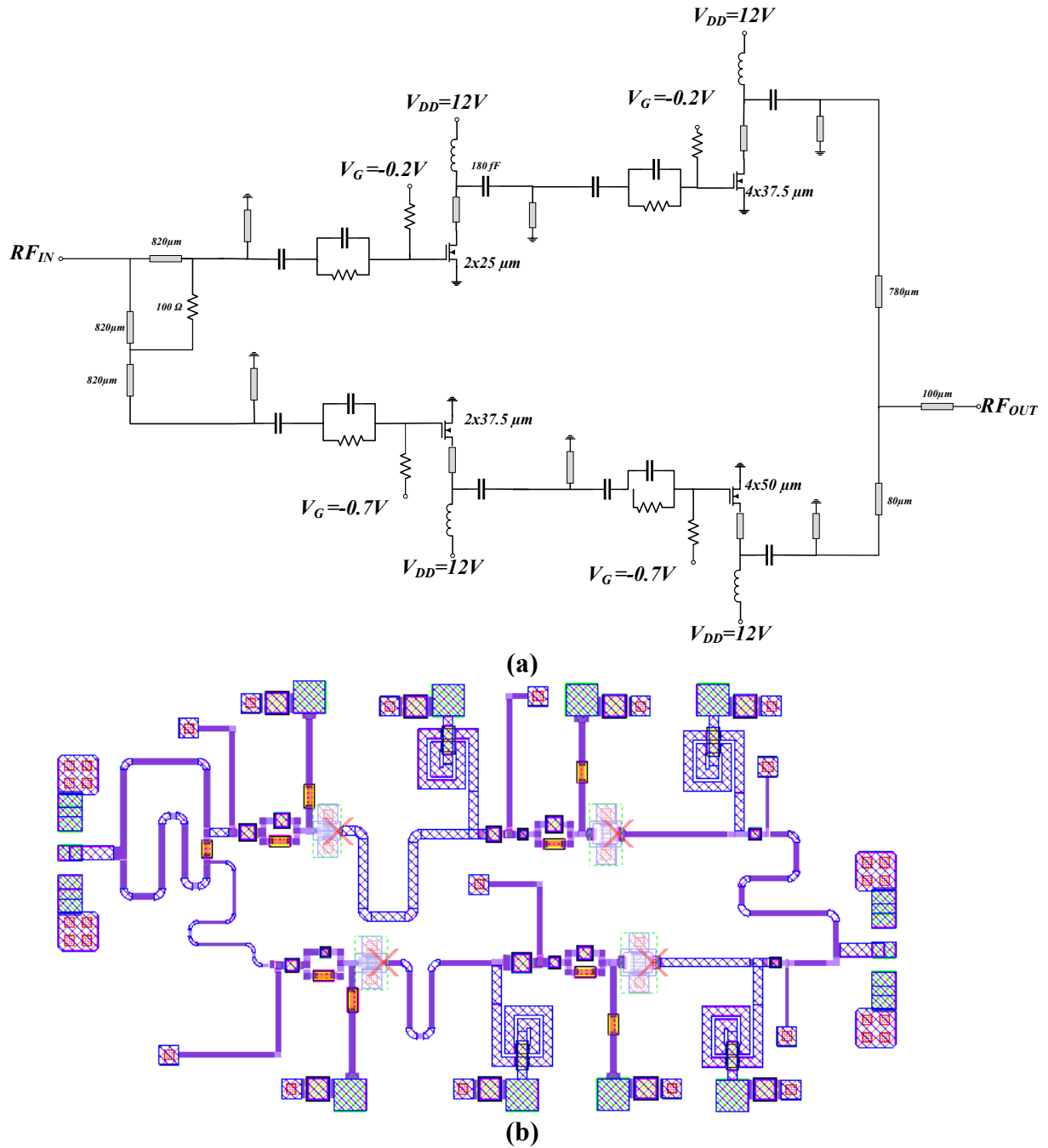
Figure 4.26: Schematic (a) and (b) layout of the two-stage 39 GHz Doherty PA
