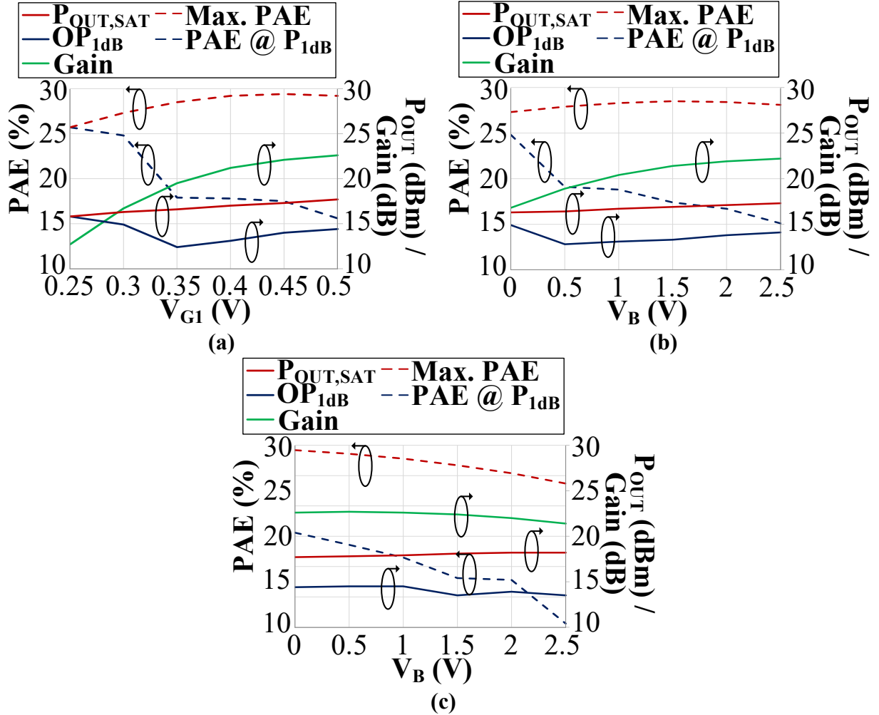
Figure 4.35: Post-layout PEX Simulations of the Two-stage CMOS PA where PAE@ P_{1dB} , max. PAE, gain, OP_{1dB} and P_{OUT,SAT} as a Function of (a) V_{G1} of the bottom CS Device on the Second Stage of the PA (with V_B = 0 V); (b) body bias V_B of the Second Stage with V_{G1} = 0.3 V; and (c) body bias V_B of the Second Stage with V_{G1} = 0.5 V
