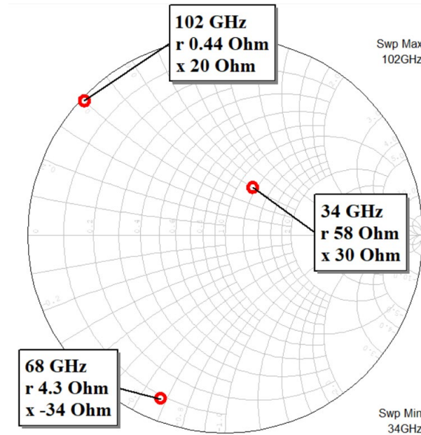
Figure 4.22: Load of the Second Stage Device of the Broadband Two-stage Class J GaN PA where f_o = 34 GHz, 2f_o = 68 GHz, and 3f_o = 102 GHz.
