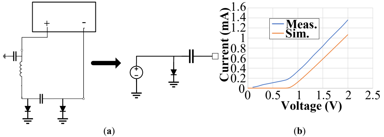
Figure 4.79: Schematic to Run the I-V Curve for the Tiedown Model (a) and (b) the I-V Curve of the Tiedown Model and the Measured I-V Curve from Biasing the V_{CC} Pad to the RF_{OUT} Pad
