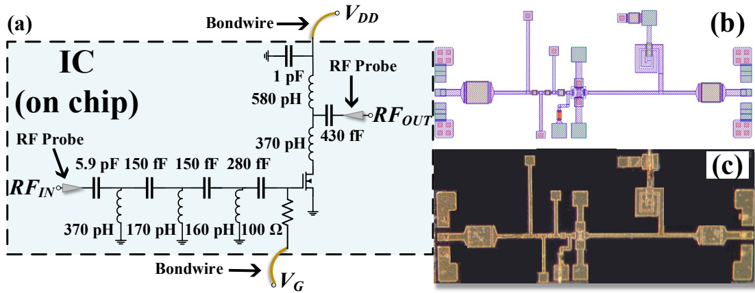
Figure 4.2: Schematic (a); (b) Layout; and (c) Micrograph of the 2.1 \times 0.88 \text{ mm}^2 Broadband mm-Wave GaN PA Designed in this Work
