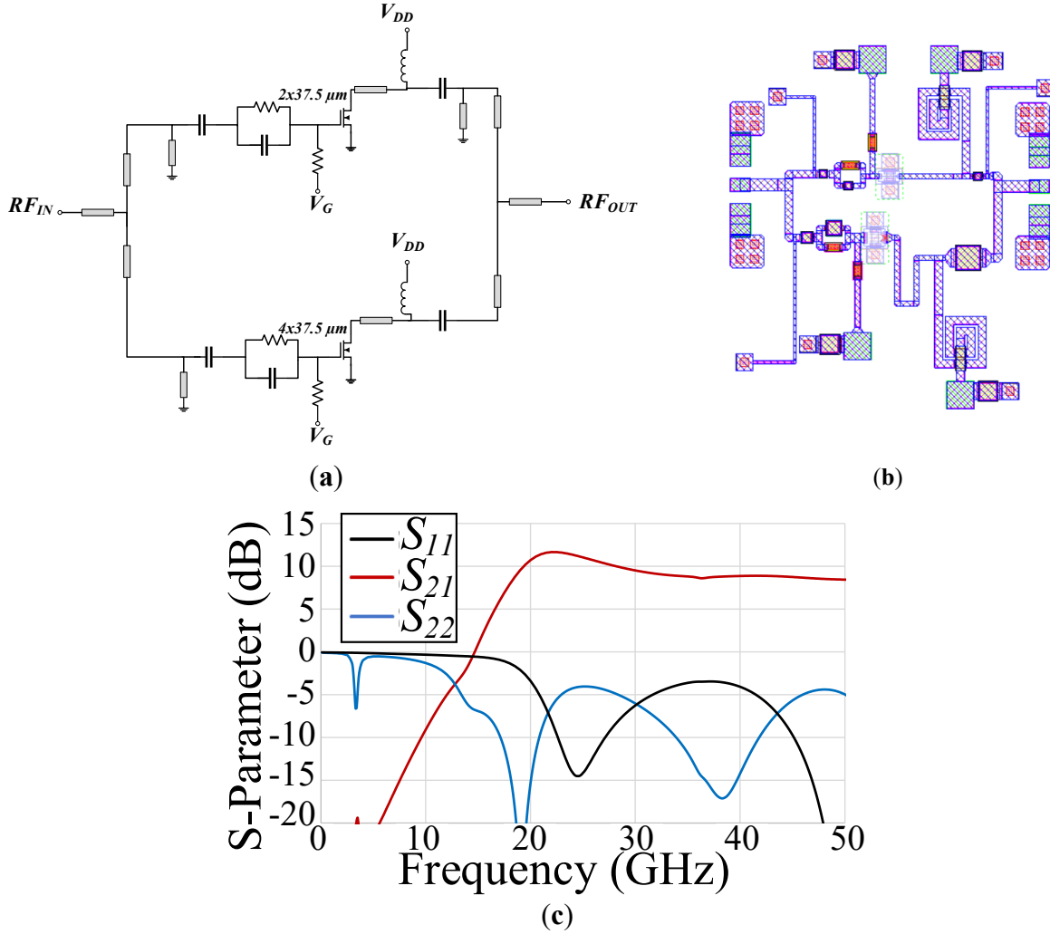
Figure 4.20: Simplified Schematics (a) and (b) the Layout of the One-stage Asymmetrically Combined GaN PA (1.1 x 1.3 mm 2 with pads); and (c) its S-parameter EM PEX Simulation Results
