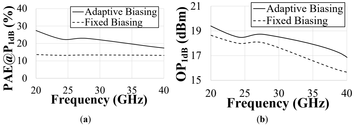
Figure 4.74: PEX Simulations of (a) PAE@P_{1dB} , and (b) OP_{1dB} vs. Frequency with the Adaptive Biasing Circuit Turned On and off of the Broadband Differential SiGe PA with RC Feedback and Neutralization Capacitors
