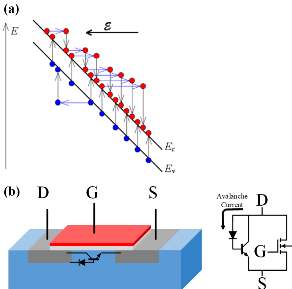
Figure 2.4: Basic Energy Band Diagram of a Semiconductor to Illustrate the Chain Reaction of Electron-hole Pairs Generation Under a High External Electric Field \mathcal{E} that is causing an Avalanche Breakdown (a); and (b) a Simplified Diagram of the Avalanche Breakdown in a n-MOSFET, where the Avalanche Current Flows through the Base-Collector Junction of the Parasitics npn BJT [8]
