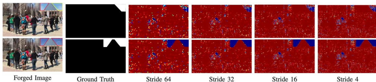
Figure 56. The Forged Scanned Images and Corresponding Reliability Maps with Different Strides
