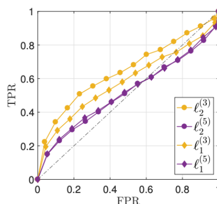
Figure 71. ROC Curve Related to the Inpainting-based Anonymization Method
