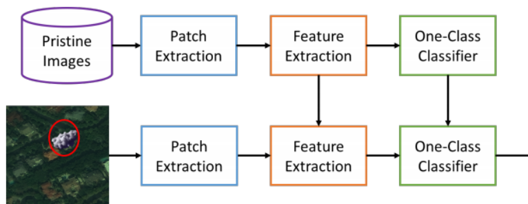
Figure 38. Pipeline of the Proposed Method. At Training Time, the Feature Extractor and One-Class SVM Learn Their Models from Pristine Images Only. At Testing Time, Forged Areas Are Detected as Anomaly With Respect to the Learned Model.
