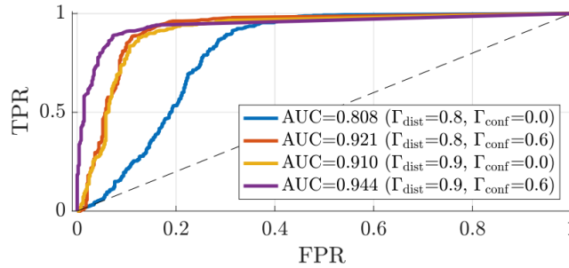
Figure 69. Area Under the Curve (AUC) for Tampering Detection Using Different Parameter Settings
