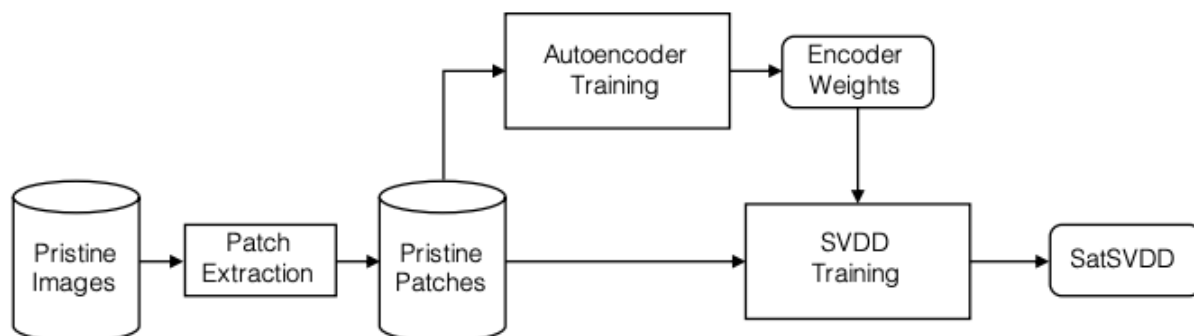
Figure 33. Overview of the Whole Training Process of Sat-SVDD
