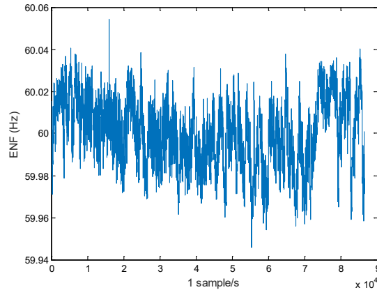
Figure 77. Ground Truth ENF Signal Computed on 10th July 2020 from Denver
