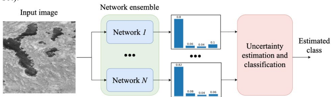
Figure 46. Pipeline of the proposed attribution method
