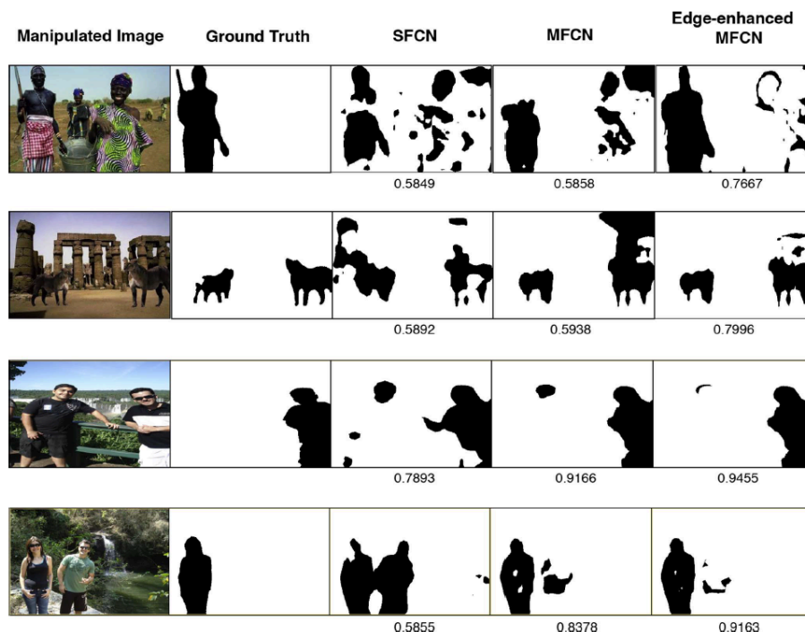
Figure 63. System Output Mask Examples of SFCN, MFCN, and Edge-enhanced MFCN on the CASIA v1.0 and Carvalho Datasets. We Refer to the MFCN without Edge-enhanced Inference Simply as MFCN. Each Row in the Figure Shows a Manipulated or Spliced Image, the Ground Truth Mask, the SFCN Output, the MFCN Output, and The Edge-enhanced MFCN Output. The Number Below Each Output Example is the Corresponding F1 Score
