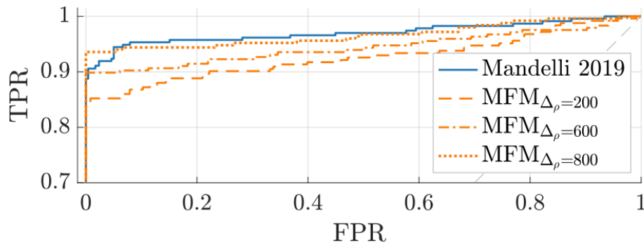
Figure 74. ROC Curves for Video PRNU Attribution
