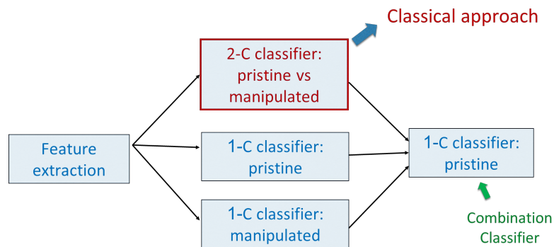
Figure 11. Architecture of the One-and-a-Half Class (1.5C) Classifier
