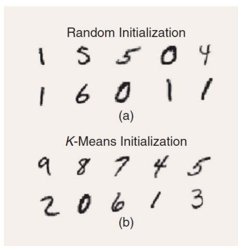
Figure 19. The Comparison of MNIST Unsupervised Classification Results of the LeNet-5 Architecture with the (a) Random and (b) K-Means Initializations, where the Images that are Closest to Centroids of Ten Output Nodes are Shown
