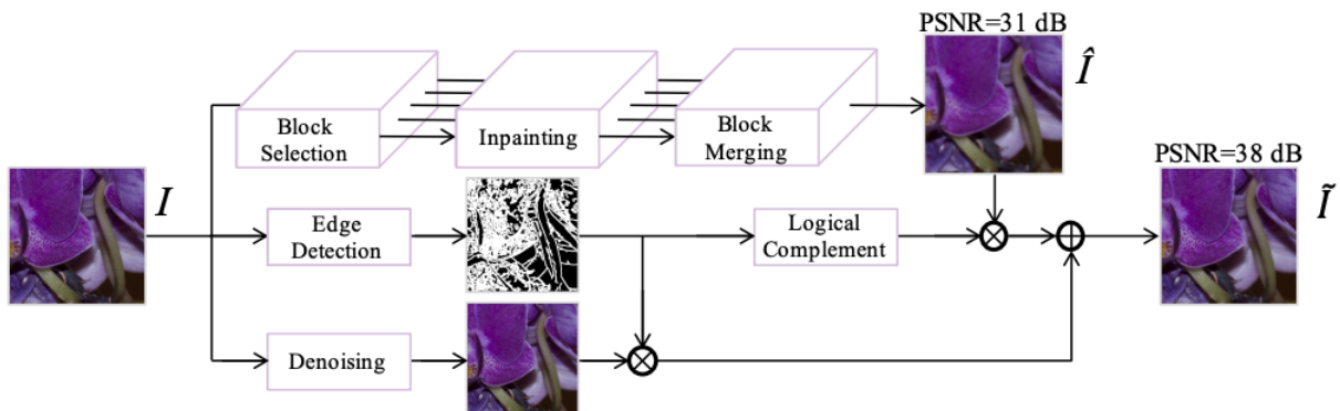
Figure 25. Main Pipeline of the Inpainting-based Method
