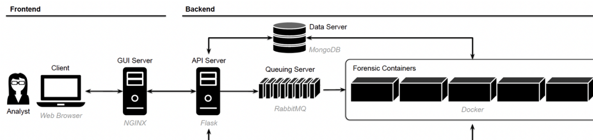
Figure 51. The architecture of SILA. We adopted a client-server model, with frontend components focused on usability, and backend components focused on scalability and extensibility. Other solutions can be added to the system if they are made available as Forensic Containers. Labels in italic on the bottom of the components detail the technology used to implement them. Arrows express the data flow between components.
