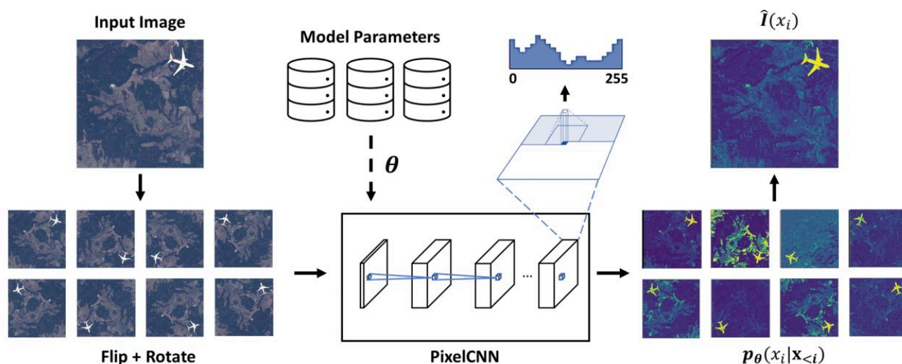
Figure 37. Proposed Ensemble: Multiple Models Process the Flipped and Rotated Input Images. The Prediction of Every Network Is Averaged Obtaining a Final Robust and Accurate Likelihood Estimate for Each Pixel of the Image. The 8 Images of p_{\theta}(x_i | x_{<i}) are Plotted as -\log p_{\theta}(x_i | x_{<i}) for Visualization Purposes.
