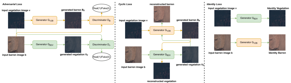
Figure 43. CycleGAN
