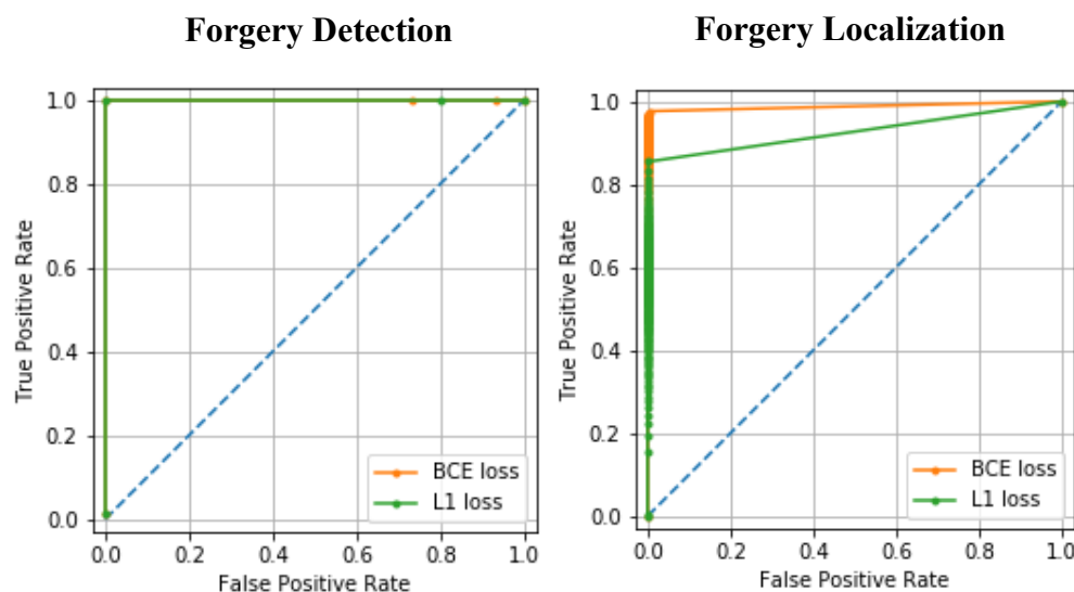
Figure 83. ROC Curves for Detection and Localization of Spliced Forgeries
