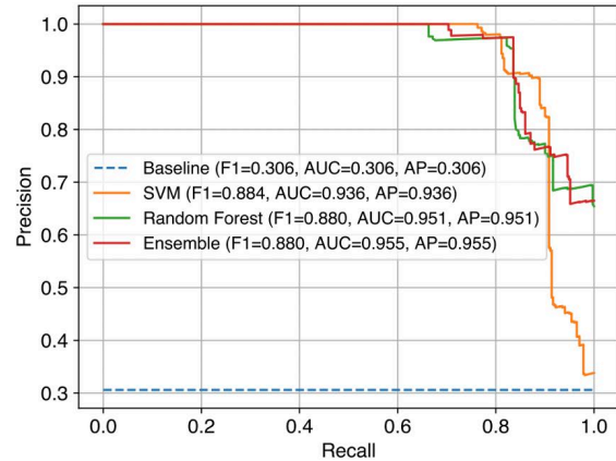
PR curves, F1 score, AUC score, and AP score on the test set for all the trained models using 50% of the available training data (339 videos).
