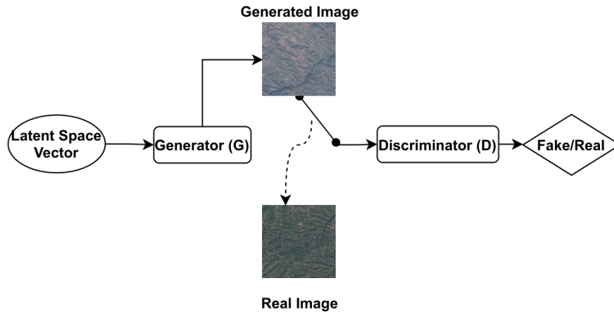
Figure 41. Basic GAN
