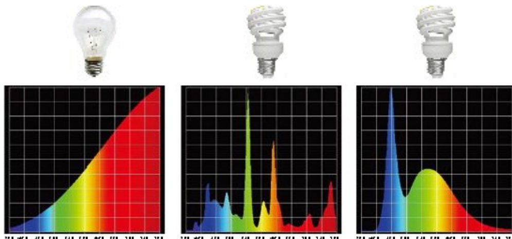
Figure 26. Spectra of Various Light Sources
