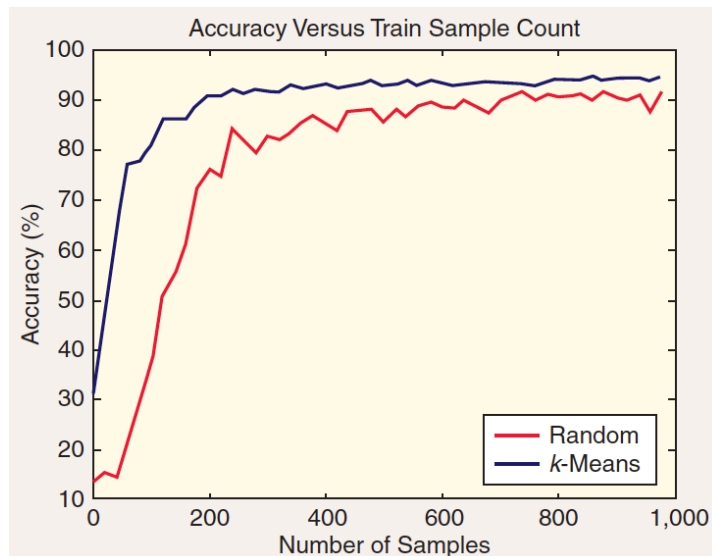
Figure 64. The Comparison of MNIST Weakly Supervised Classification Results of the LeNet-5 Architecture with the Random and K-Means Initializations, where the Correct Classification Rate is Plotted as a Function of Training Sample Numbers
