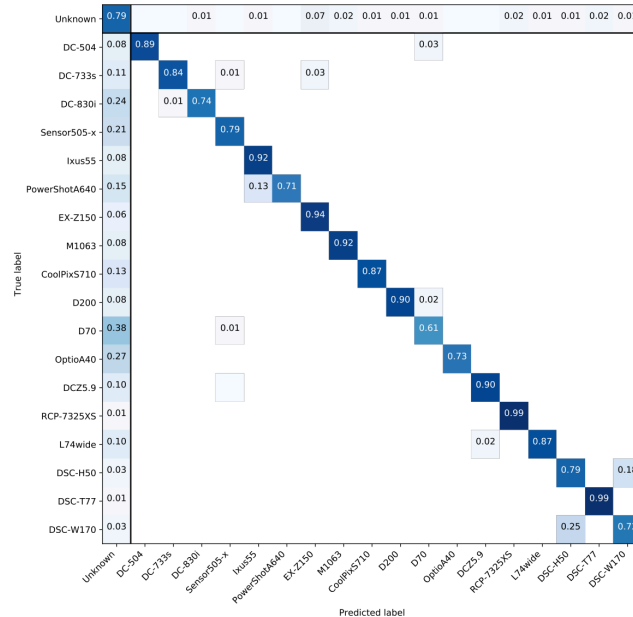
Figure 70. Open-set Camera Model Identification Confusion Matrix
