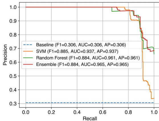
PR curves, F1 score, AUC score, and AP score on the test set for all the trained models using 25% of the available training data (169 videos).
