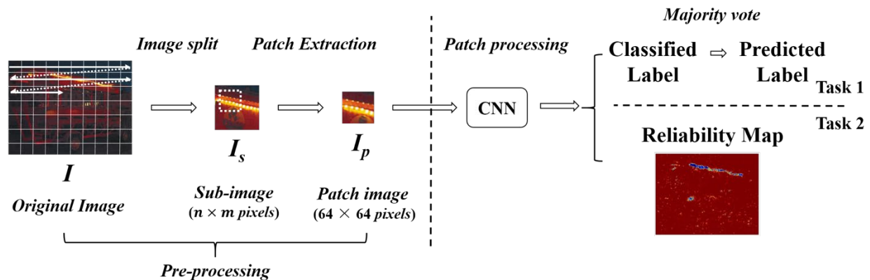
Figure 6. The proposed system for scanner model identification
