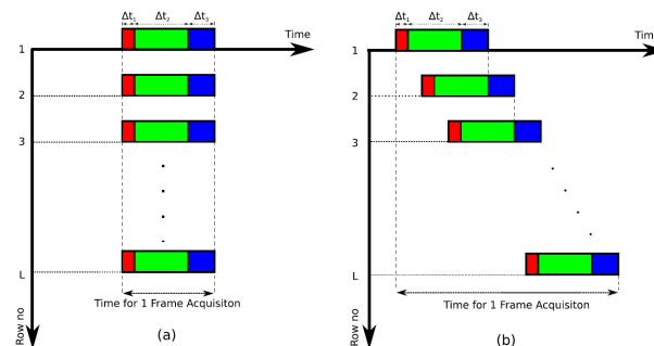
Figure 27. Demonstration of (a) Global Shutter Sampling Mechanism – Each Row of a Frame Is Exposed at the Same Time Instance (b) Rolling Shutter Sampling Mechanism
