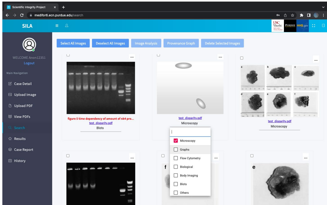
Figure 107. Manual correction of image labels
