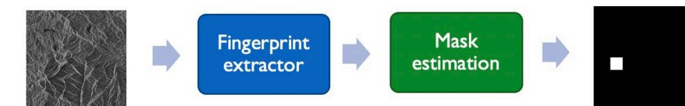
Figure 44. SAR Forensic Pipeline
