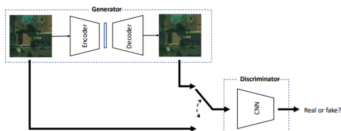
Figure 39. Architecture of the Used GAN
