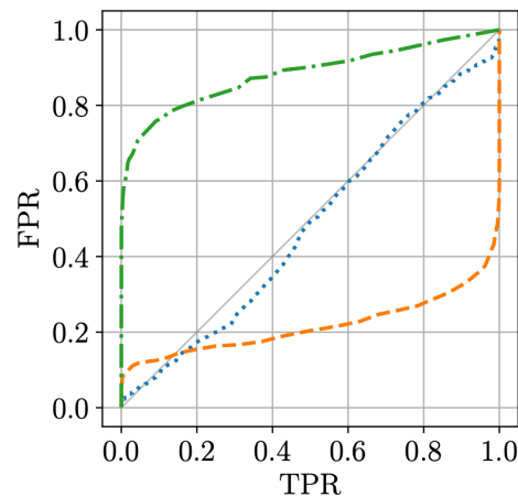
Figure 72. Results Achieved Through the Use of the Anonymization CNN
