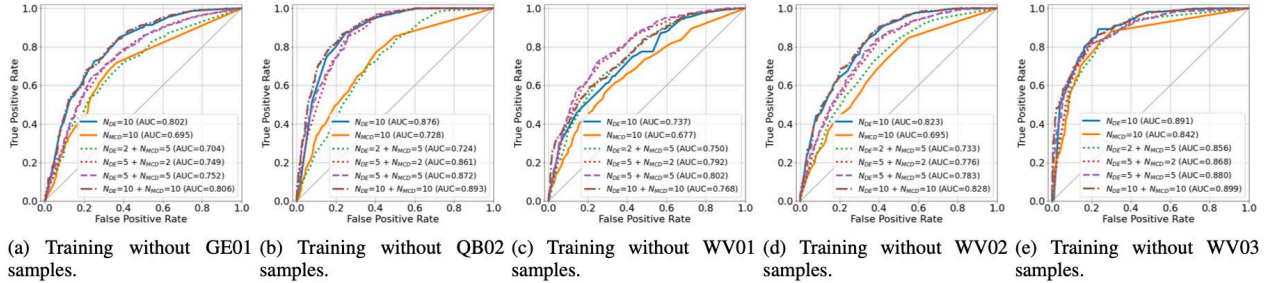
Figure 94. Open-set results for the leave-one-class experiments. N_{DE} and N_{MCD} denote N values for DE and MCD whenever they are combined
