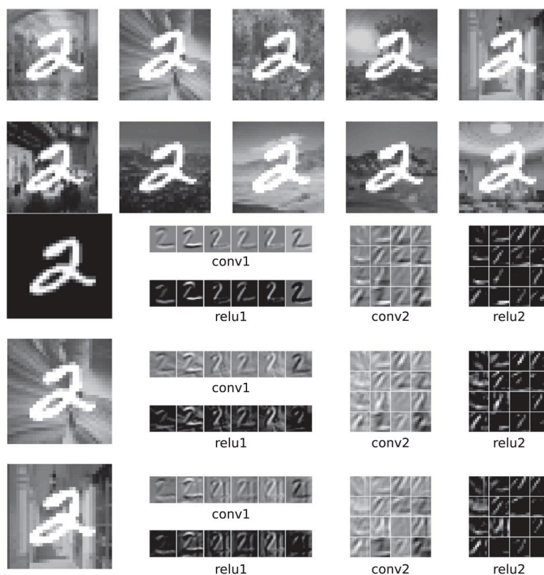
Figure 67. The MNIST Dataset with 10 Different Background Scenes (Top 2 Rows). Filter Response of 1st and 2nd Layer of LeNet-5
