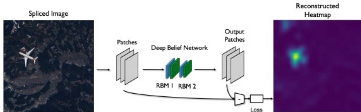
Figure 36. Method Overview for Generating the Heatmap and the Detection Score
