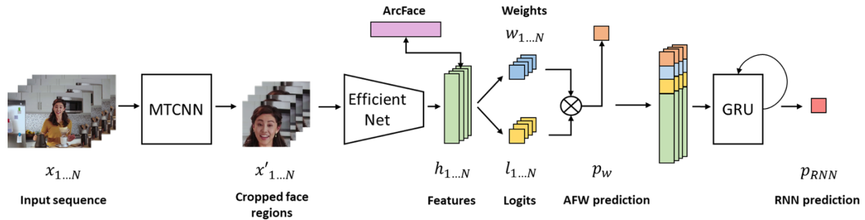
Figure 2. Block Diagram of the Proposed Deepfake Detection Method
