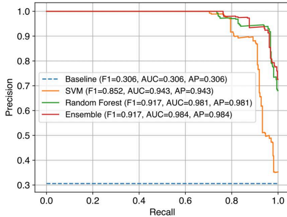
PR curves, F1 score, AUC score, and AP score on the test set for all the trained models using 10% of the available training data (68 videos).
