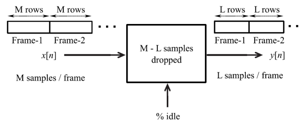
Figure 28. Inherent Reduction in Captured Luminance Samples in a Video Due to the Implementation of Idle Period at the End of Each Frame by Camera
