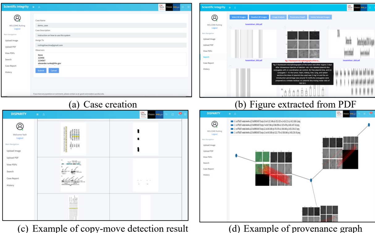
Figure 96. Screenshots of the Scientific Integrity System
