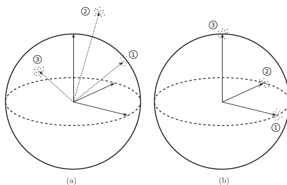
Figure 24. Illustration of Functions of Convolutional Layer C5 and Fully Connected Layer F6 in LeNet-5 Architecture
