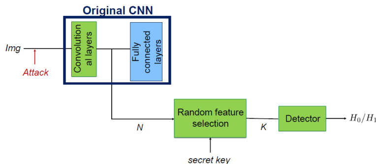
Figure 13. Scheme of the RDFS Detector
