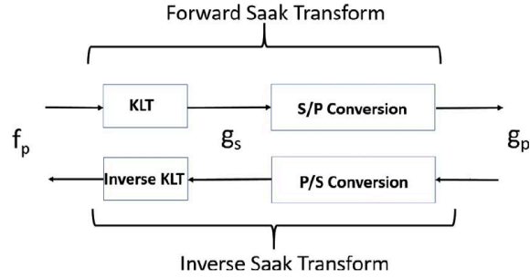
Figure 21. The Block Diagram of Forward and Inverse Saak Transforms
