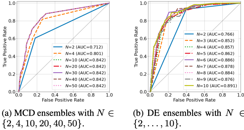
Figure 93. ROC curves obtained using MCD or DE ensembles with different N values
