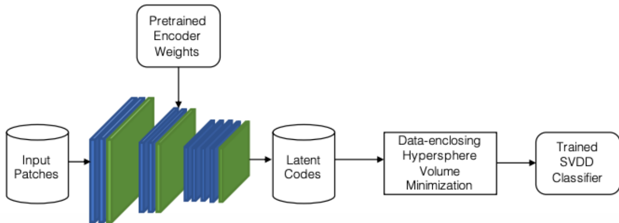
Figure 34. Overview of the Sat-SVDD Training Step
