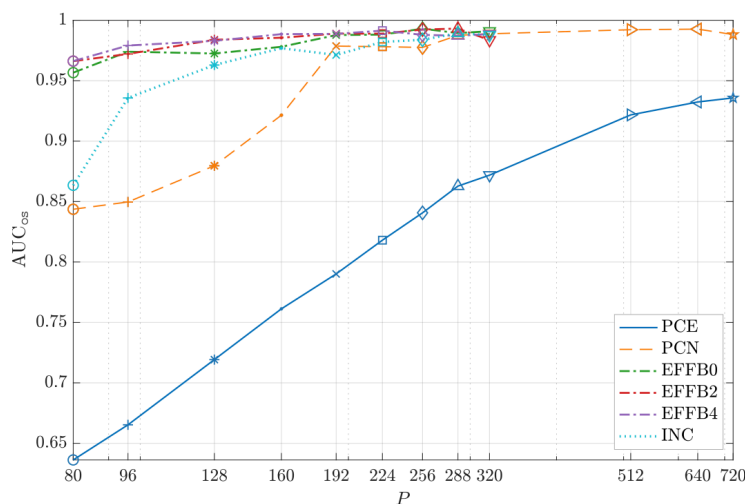
Figure 73. PRNU Attribution AUC vs. Patch Size for Different CNNs and the Standard PCE Test
