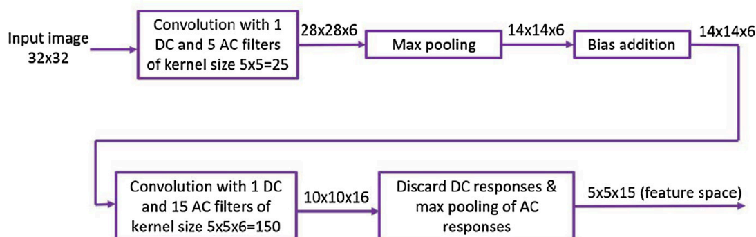
Figure 15. Summary of the FF Design of the First Two Convolutional Layers of the LeNet-5
