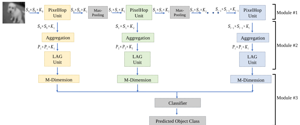
Figure 20. Block Diagram of the PixelHop Method
