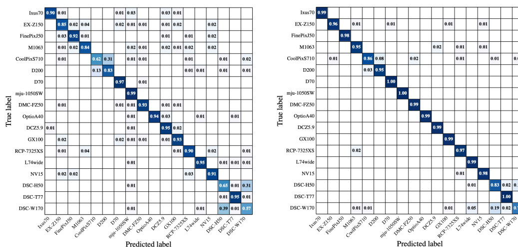
Figure 68. Camera Model Identification Results [1, 2] (left) and the Improvement Obtained with [3] (right)
