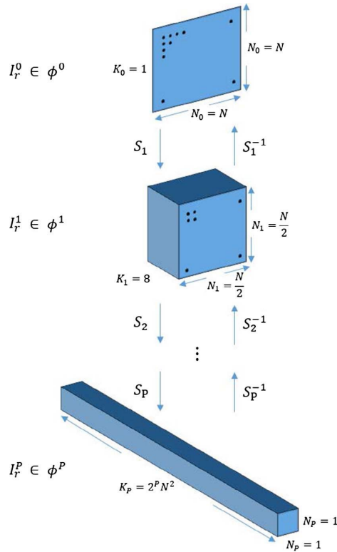
Figure 22. The Conversion Between an Input Image and Its Spatial-Spectral Representations via Forward and Inverse Multi-Stage Saak Transforms
