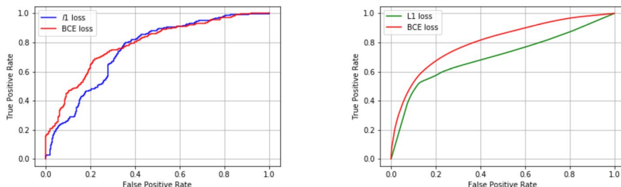
Figure 57 AUC of Standard (l1) vs Proposed (BCE) Loss
