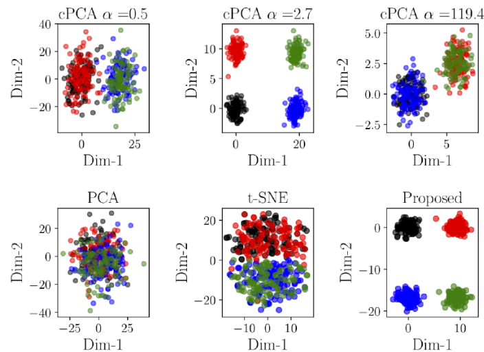
Figure 61. Performance on a Synthetic Dataset, where Different Colors are Used for the Four Different Classes
