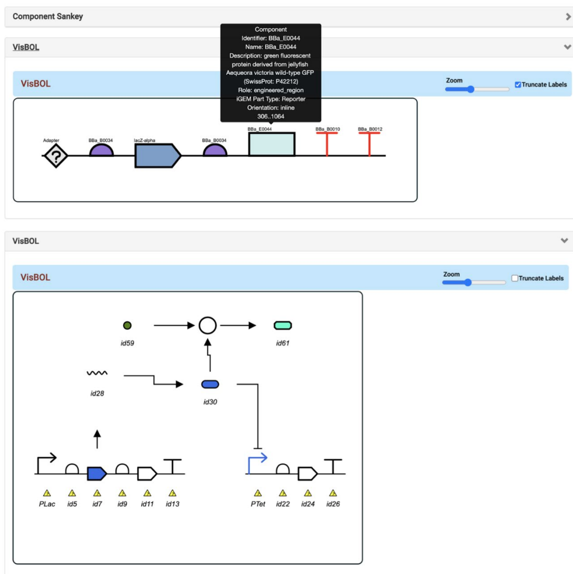
Figure 118. Further updates in genetic circuit design structure and function as part of SynBioHub's plugin architecture.
