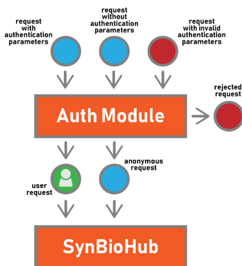
Figure 112. New authentication module for SynBioHub. All requests to access SynBioHub will come through this module. This will support more fine grain user and group permissions. It will also allow anonymous access to support share links.
