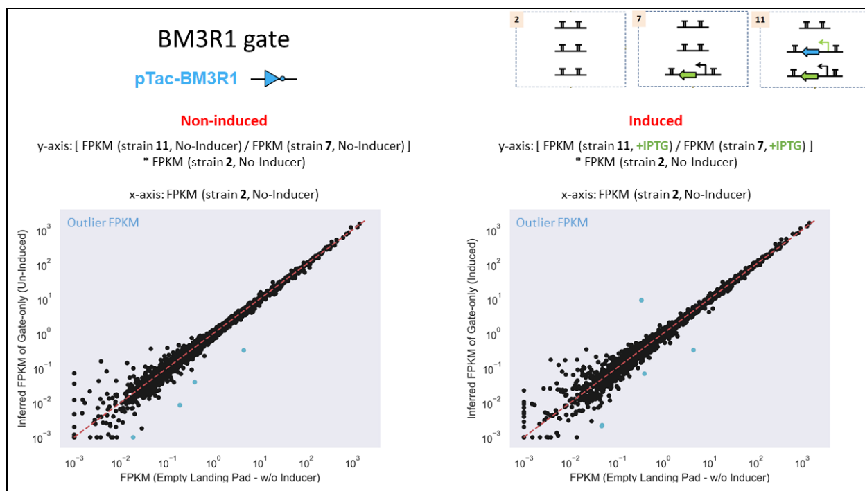
Figure 30. Exclusive impact of BM3R1 gate under induced and non-induced conditions. The quantification formula is shown. Schematics of strains used in the formula are shown in top right. Each box represents a strain with three landing pads in the genome (from bottom to top: sensor landing pad, repressor landing pad, YFP landing pad). The x-axis is the measured genomic FPKM data from the control strain 2 (empty landing pads), and y-axis data is the predicted genomic FPKM of the repressor. Outlier genes with significant deviation from x=y are marked with blue color.
