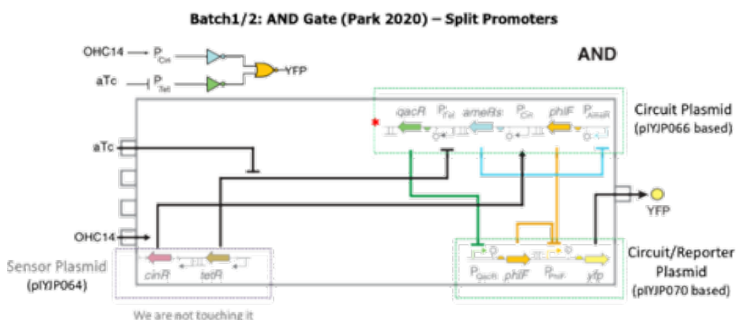
Figure 99. The schematic of the AND logic Gate (from Park et al., 2020) will receive MoClo-adapted parts before the rapid, modular assembly of genome-integration plasmids. The two circuit plasmids (pIYJP066 and pIYJP070) have been designed to carry level-1 and level-2 fragments flanked with the appropriate MoClo scars. The circuit pIYJP066 (red asterisk) adaptation requires a new gate design from scratch since it is not present in the CIDAR MoClo library.
