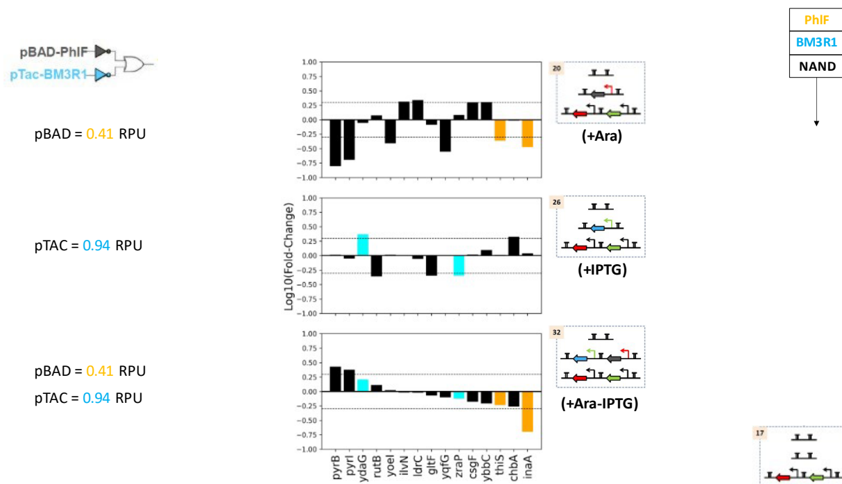
Figure 36. List of regulated genes in PhIF-BM3R1 NAND circuit. Orange and light blue colors represent exclusive target genes for PhIF and BM3R1, respectively. The strains used to identify the targets genes are shown as dashed box next to each plot, and the reference strain is shown in bottom right corner. The strength of promoters expressing each repressor is also shown in RPU.
