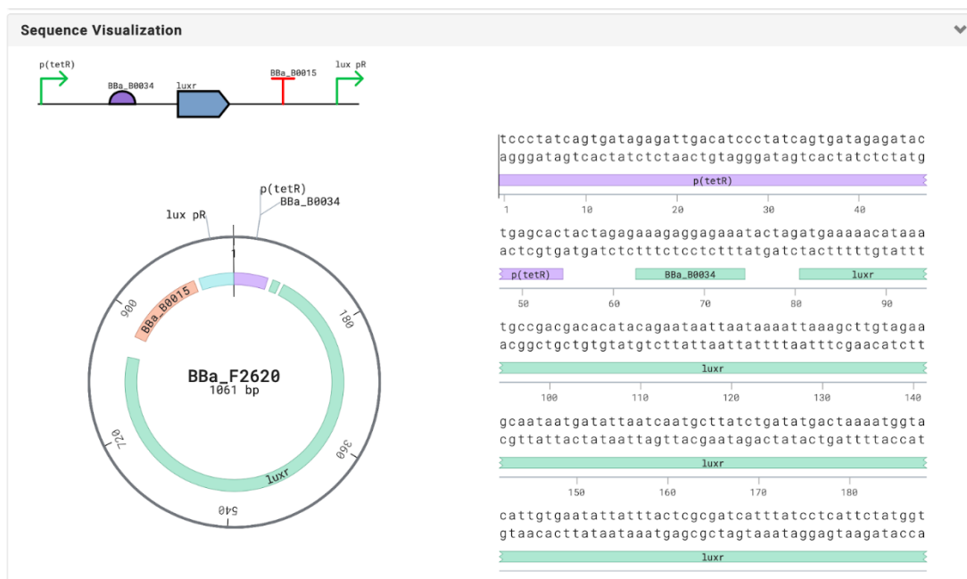
Figure 115. Sequence visualization using SynBioHub's plugin architecture.
