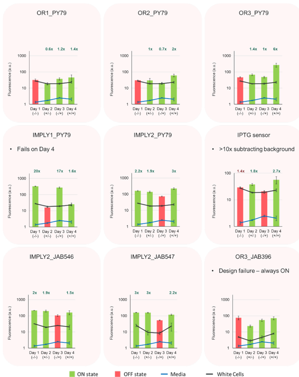
Figure 57. Plate reader fluorescence from obstacle course run at Strateos at 35C.
