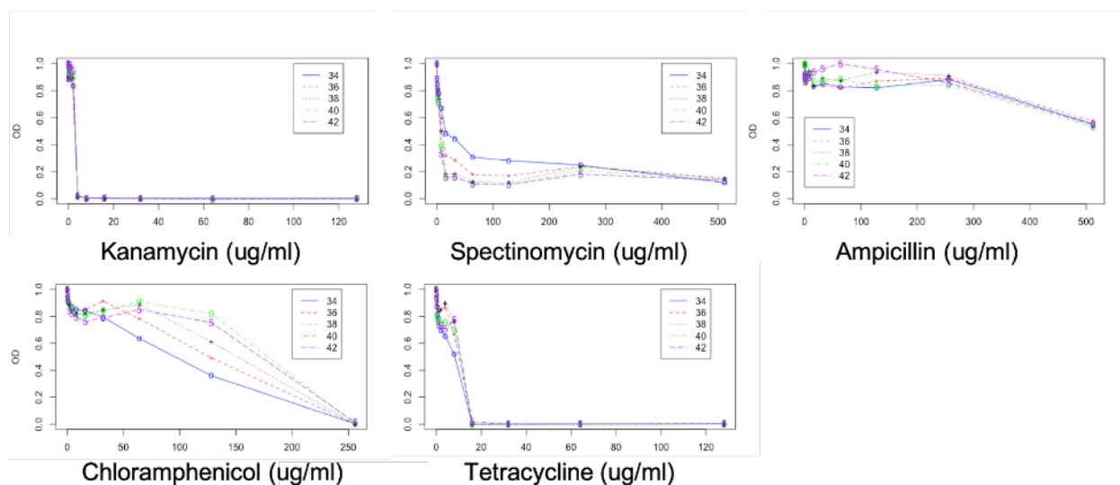
Figure 78. MIC results for Pseudomonas protegens PF5. Kanamycin, and tetracycline are ideal choices for selection of modified protegens. Protegens showed some tolerance to spectinomycin at higher concentrations that slightly decreased with time. MIC50 for chloramphenicol greatly increased with time, suggesting an increased tolerance with exposure. Protegens was resistant to Ampicillin, which is common for Pseudomonads .
