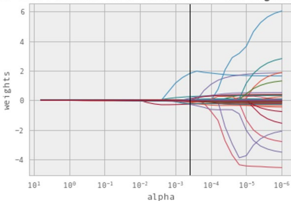
Figure 82. Lasso computer Rosetta terms and alpha value. Top: The Lasso computed Rosetta terms that are major contributors to ProStab stability score. Bottom: The computed alpha value which thresholds the scores that get minimized to zero during significance evaluation.
