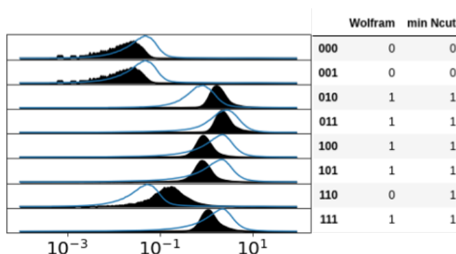
Figure 92. A circuit marked as successful in the Cello publication (Nielsen et al., 2016), but where the best-normalized cut score was lower than the specified truth table. By the normalized cut metric, the circuit would be marked as a "failure." The column denoted "Wolfram" is the truth table of the desired circuit behavior in the table. The column marked "min Ncut" is the truth table with the minimum normalized cut score of all possible 3-input truth tables.
