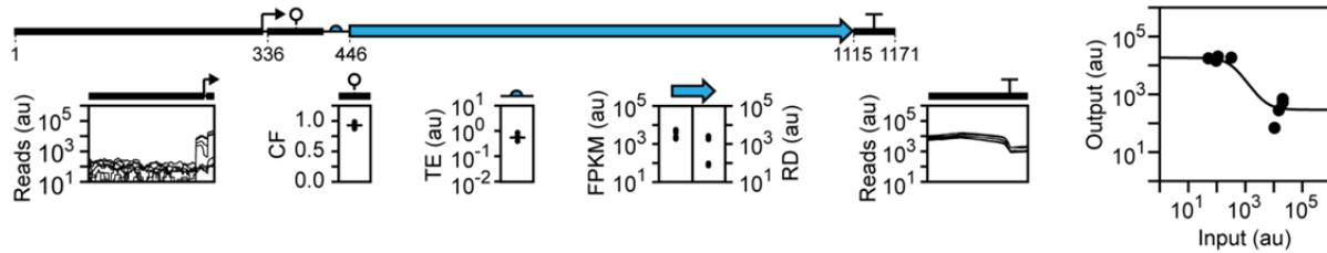
Figure 4. Full characterization of a gate's biological parts using RNA-seq and Ribo-seq. From left to right: 1- promoter activity and transcription start site are shown using RNA-seq, 2- ribozyme cleavage fraction are quantified using RNA-seq, 3- translation efficiency of RBS is quantified using Ribo-seq, 4- FPKM and ribosome density of each protein is calculated using RNA-seq and Ribo-seq, respectively, 5- terminator strength and transcription termination site are shown using RNA-seq, 6- input-output response of each gate is quantified using RNA-seq.
