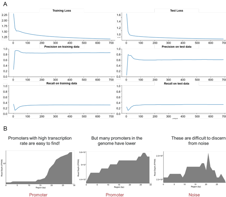
Figure 11. Results of genetic part identification model (A) Results of the ML model on both training and test data sets. (B) Transcription profiles of 30bp regions – first two are promoters and third isn't.
