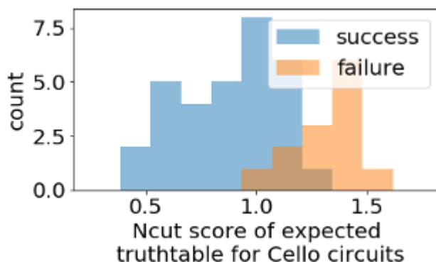
Figure 93. Histogram of normalized cut scores for 44 circuits scored from the Cello publication (Nielsen et al. 2016). "Success" or "failure" denotes whether a circuit was reported in the publication as a faithful implementation of the truth table specified during design.
