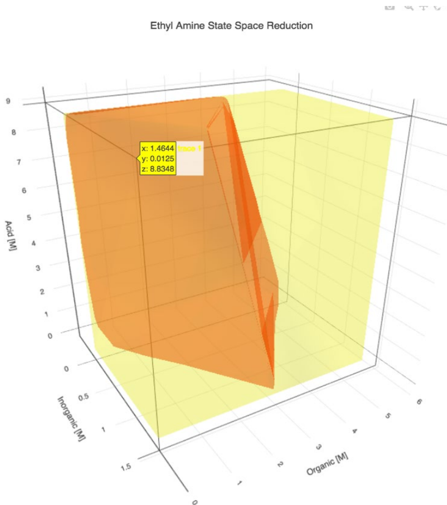
Figure 83. Convex hull limiting the statespace of the ethyl amine predictions
