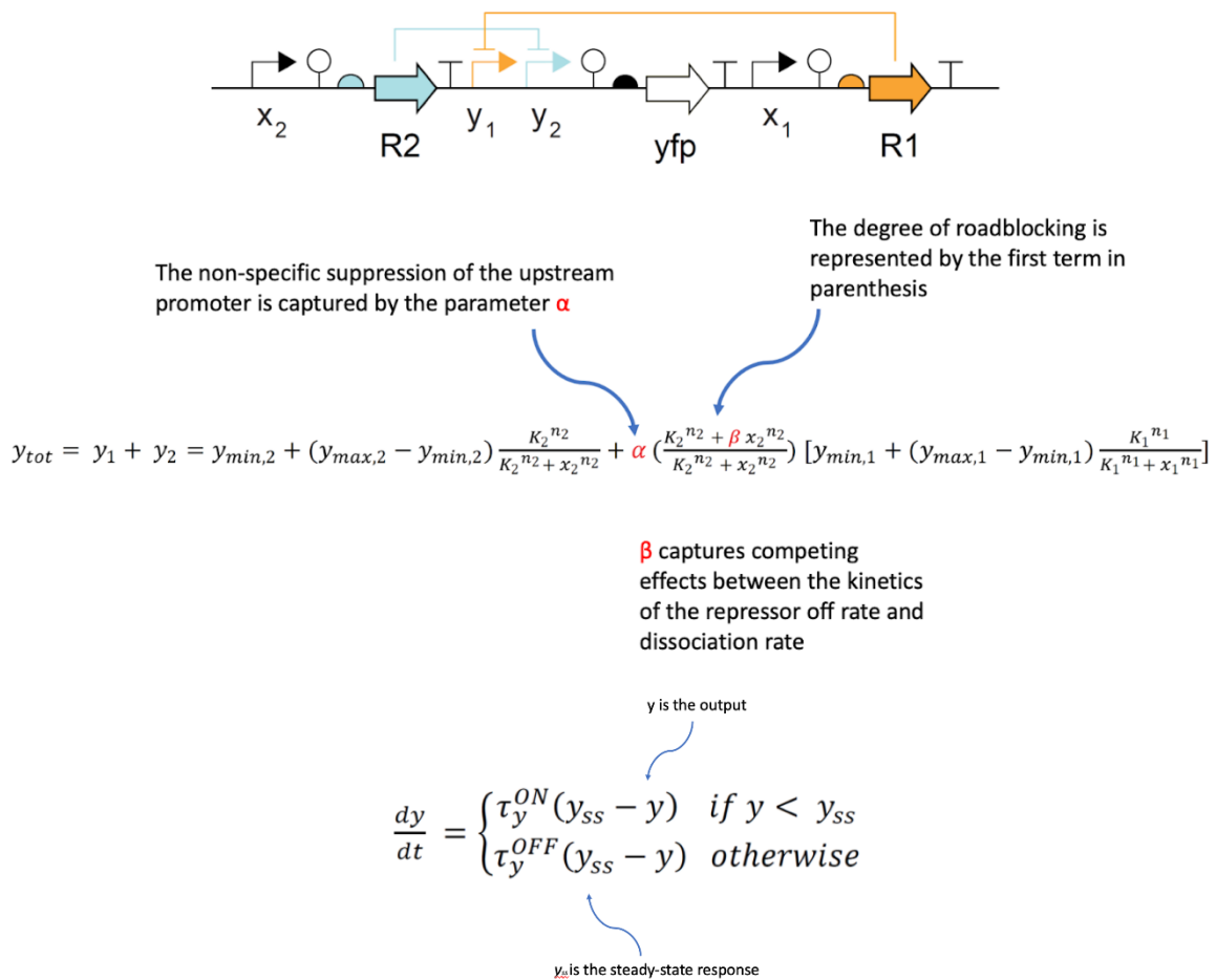
Figure 123. Improved dynamic model formulation. The new steady-state model includes parameters to express the effect of roadblocking. The dynamics are now governed by measured rates of change to turn on and off.
