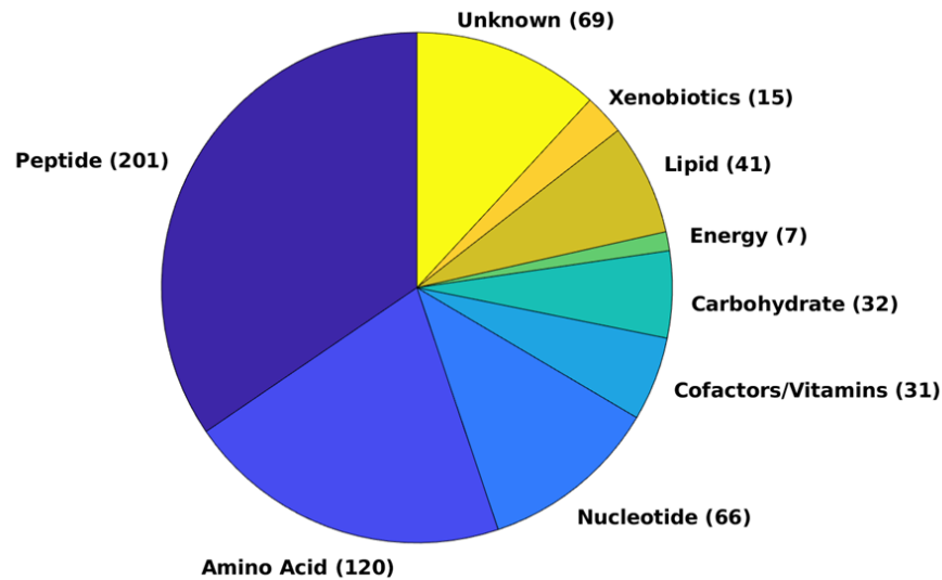
Figure 40. Breakdown of the metabolites detected in our metabolomics study.
