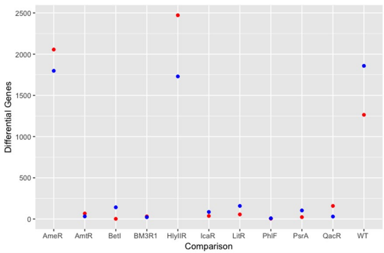
Figure 74. Differential expression of NOT gates to sensors. Red - no induction, blue - induction. HlyIIR and AmeR are least like the sensors, with differential levels similar to that of the wildtype. Most of the other gates were very similar to the sensors.
