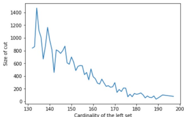
Figure 108. Graph shows the number of cuts vs. cardinality of one of the sets using the modified Karger's algorithm. Out of 264 total operation types, cardinality 177 means that the left set will contain 67% of all operation types, and the right retains 33%.
