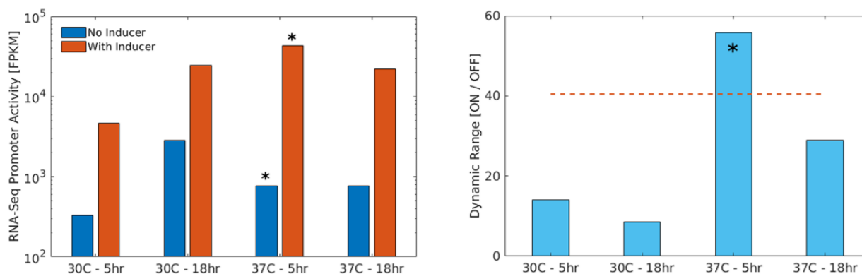
Figure 26. Effect of growth conditions on the activity of pTACmin promoter. Left plot shows the ON and OFF activities and right plot shows the dynamic ranges. The growth conditions are shown under x-axis. The horizontal dashed line is Cello value at standard condition (37 °C and 5 hours), and asterisk symbol shows RNA-seq value at standard condition.
