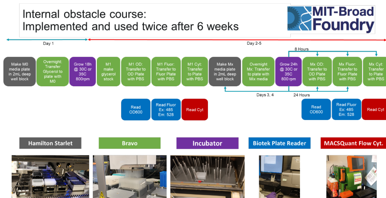
Figure 53. Schematic of 4-day obstacle course as implemented at the Broad institute.
