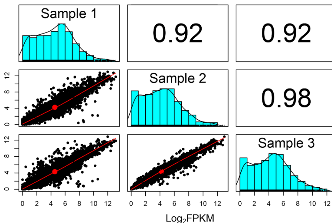
Figure 76 Pearson's correlations for B. subtilis (upper right numbers) between log2 FPKM of 5 hour time points on each of the three different days. Samples 2 and 3 have much more similar patterns compared to 1-2 and 1-3. Additionally, these two comparisons have a lower correlation than the 5-8 hour E. coli comparisons, suggesting greater variability in the growth/biological conditions for B. subtilis . Scatterplots are gene-gene Log 2 FPKM comparisons, with a red linear regression line. Blue plots are histograms for frequencies of gene FPKMs.
