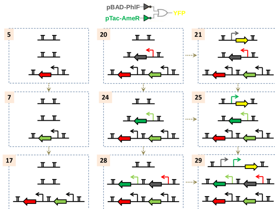
Figure 45. Decomposition of a NAND circuit into its building block components.
