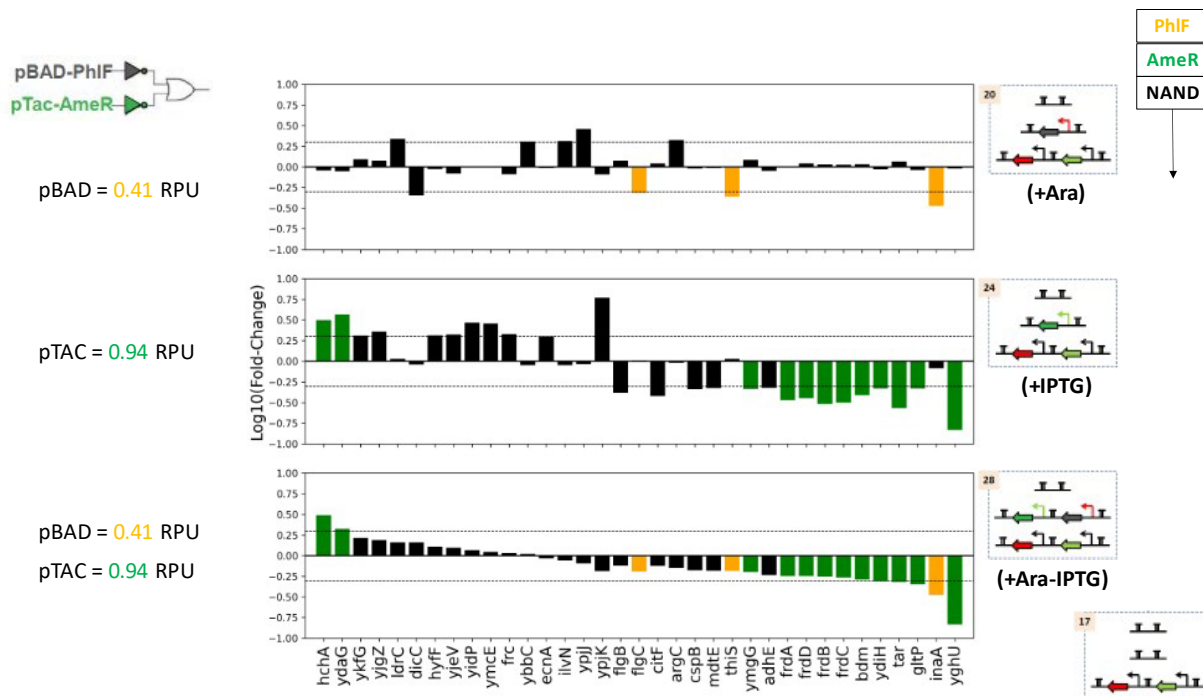
Figure 34. List of regulated genes in PhIF-AmeR NAND circuit. Orange and green colors represent exclusive target genes for PhIF and AmeR, respectively. The strains used to identify the targets genes are shown as dashed box next to each plot, and the reference strain is shown in bottom right corner. The strength of promoters expressing each repressor is also shown in RPU.
