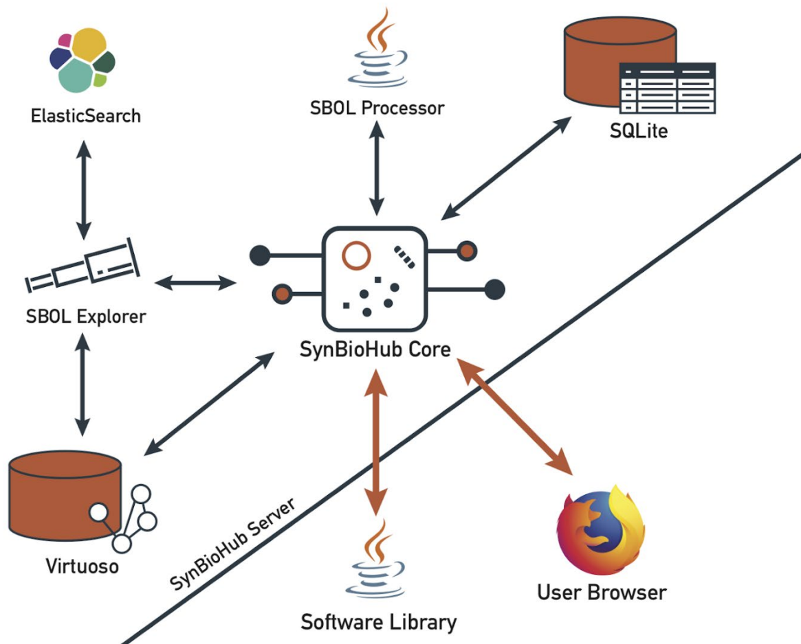
Figure 116. SynBioHub new backend and front-end architecture.
