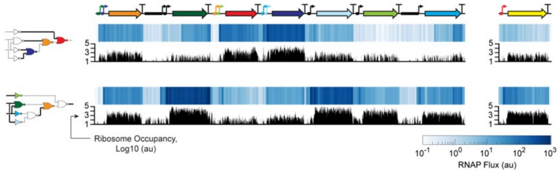
Figure 2. Transcription and translation profiles across a genetic circuit.
