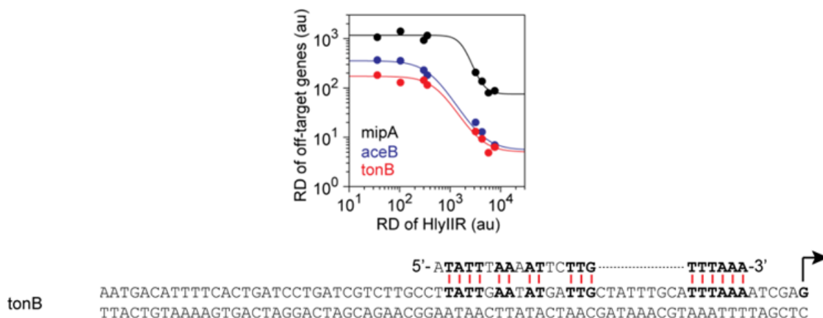
Figure 9. Off-target activity of HlyIIR repressor. RNA-seq showed that HlyIIR has off-target activity toward genes on the genome. Top plot shows the repression curves of three off-target gene on the genome. Bottom plot shows the potential binding site of HlyIIR on tonB promoter on the genome.
