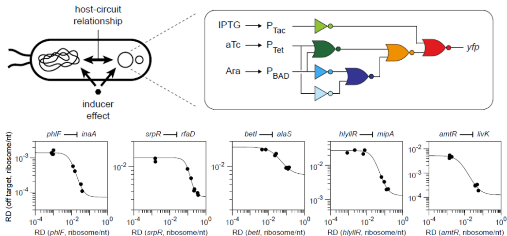
Figure 37. Off-target activity of all repressors in the circuit. Examples of non-specific interactions between circuit's repressor proteins and the native genes on E. coli genome. Genes are correlated according to a Hill function, suggesting a regression mode of gene regulation.
