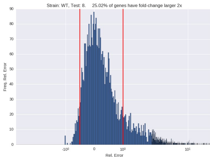
Figure 49. Accuracy of whole genome simulator for wild type E. coli at stationary phase. The distribution of relative errors for predicted expression of all native genes in WT strain when both IPTG and arabinose are present and growth is at stationary phase. Red lines depict the 2-fold error thresholds.
