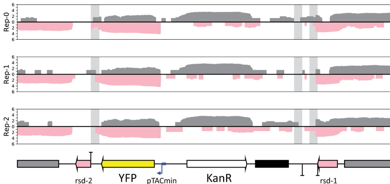
Figure 22. Transcription profile of genome-integrated promoters in uninduced conditions Transcription profiles of the genome-integrated YFP reporter across 4 biological replicates are shown under standard condition (37 °C and log-phase) without IPTG induction. One of the replicates was lost due to robot handling issue. The DNA annotation is shown at the bottom. Gray and pink regions in the transcription profiles represent sense and antisense transcription, respectively. The grey columns are the location of terminators that were used to insulate the synthetic gates from the neighboring genomic regions by splitting the native gene rsd . The location of promoter of interest (pTACmin) is also shown.
