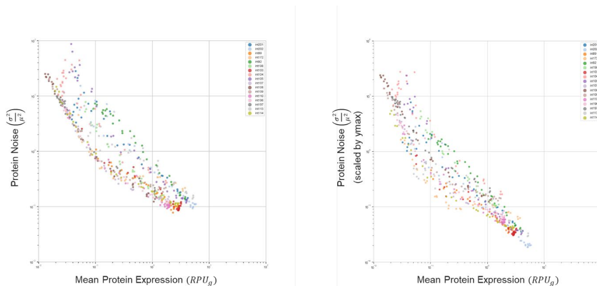
Figure 20. Noise levels across different genomic gates in E. coli left (a) Noise (as variance over mean squared) within a cell population as a function of the mean expression level for 17 strains containing a genomic gate each, represented by different colors. (right) same data scaled in noise by the output promoter's maximum strength
