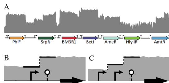
Figure 10. Transcription profiles showing curated RNA sequencing data (A) a synthetic DNA segment containing circuit elements and expected profiles around a single promoter (B) or tandem promoters (C)
