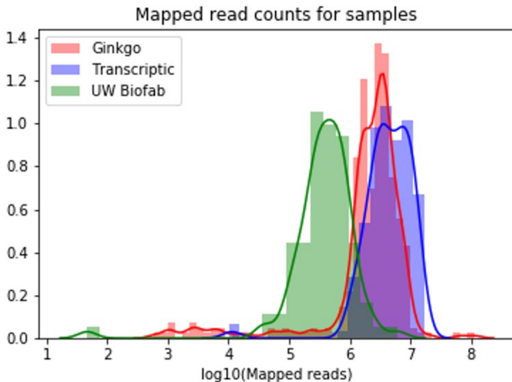
Figure 67. The number of mapped reads for each lab is log10 scaled and shows many samples pass the QC threshold of 1 million mapped reads. Ginkgo and Transcriptic had a majority of samples above the threshold while UW Biofab only had 10 samples remaining for downstream testing.
