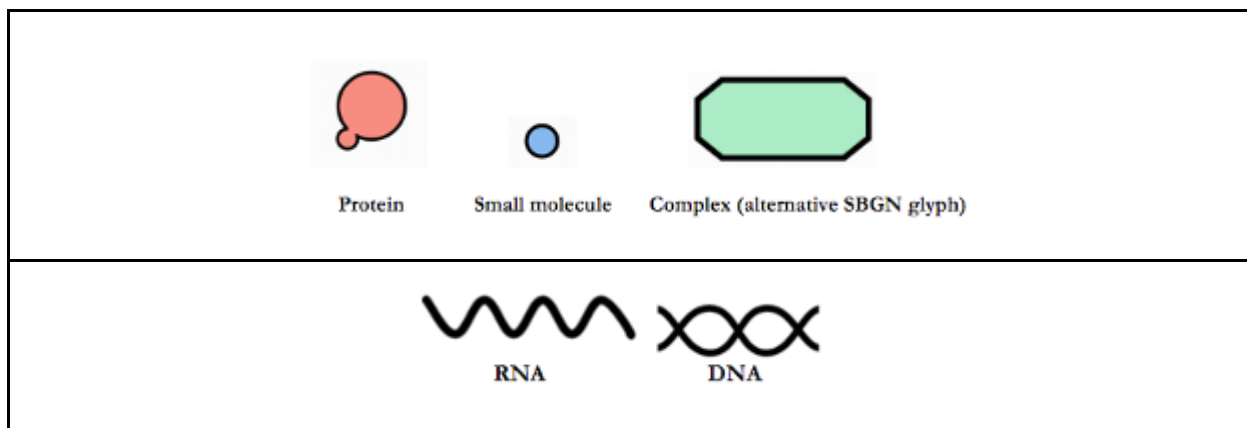
Figure 109. New glyphs added to VisBOL
