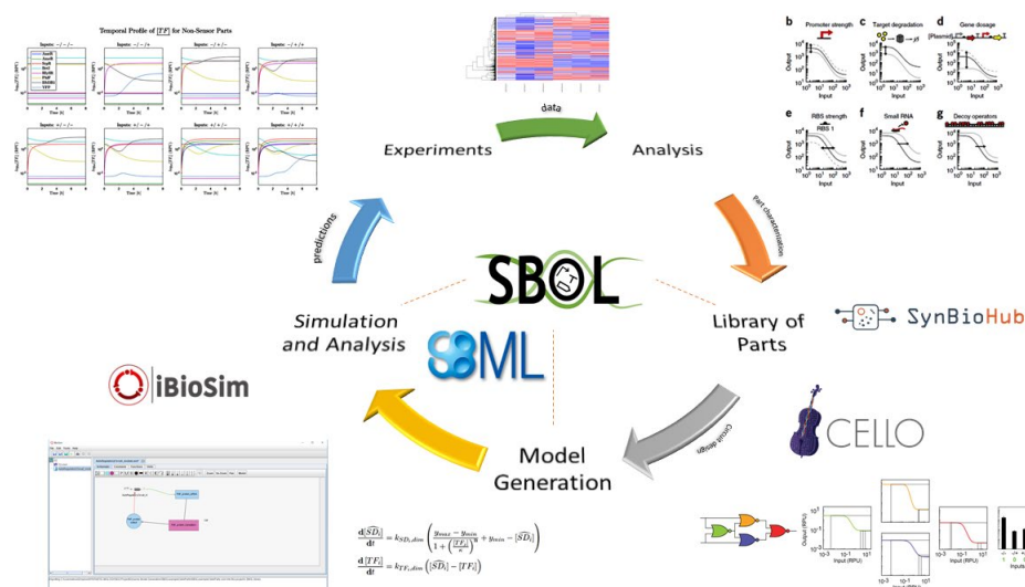
Figure 120. Updated proposed workflow for the integration of experimental data with data modeling/simulation using a new dynamic model for genetic circuits created by Hamid Doosthosseini, integrated to iBioSim to produce RNAseq and Protein concentration predictions to be compared with experimental data and to help de-bug genetic circuits.
