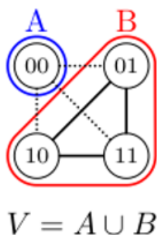
Figure 91. The specification of the normalized cut score. A graph with nodes representing the different states of the circuit is first fully connected then partitioned to match other truth tables. The edge weights correspond to the Wasserstein distances between cytometry distributions. A lower score indicates a more faithful implementation of a particular truth table.
