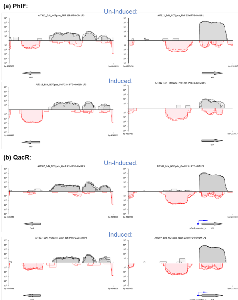
Figure 61. RNA sequencing profiles of engineered E. coli Nissle. Left panels show the gate region where the repressor is expressed under induction, right panels show output region where YFP is expressed by a repressible promoter. (A) PhlF and (b) QacR gate.
