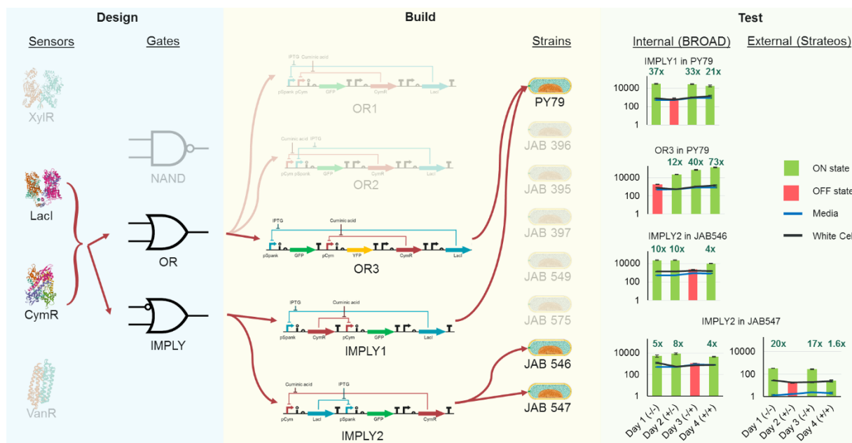
Figure 58. Creating 4 functional constructs in new hosts. Pressure test accomplishments after 4 months
