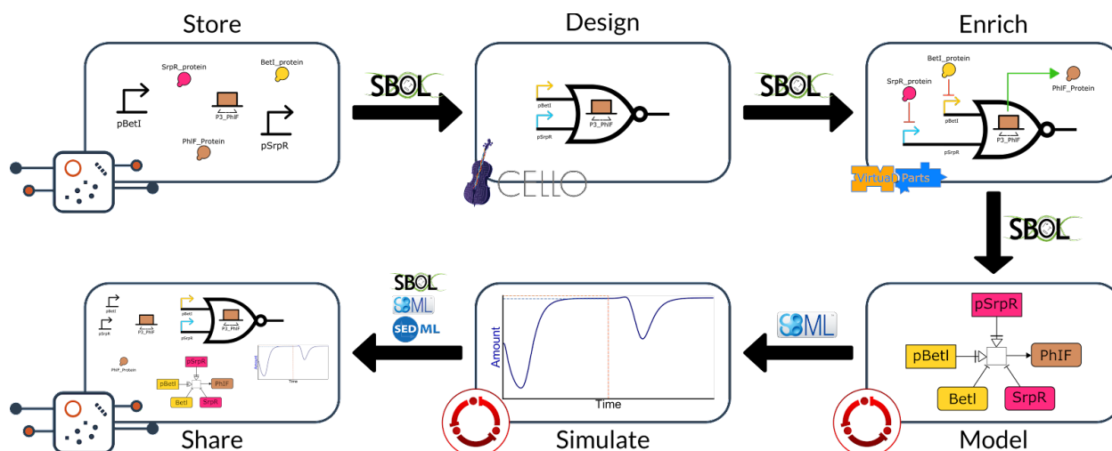
Figure 124. Design build test learn workflow for genetic circuit failure percent characterization and modeling. This workflow shows how a user can start with parts and designs in SynBioHub and end up with prediction models for the same designs, also using SynBioHub.
