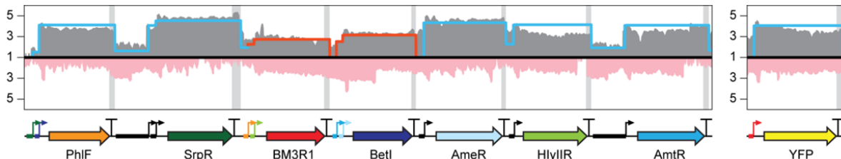
Figure 3. Validation of Cello using RNA-seq profile.
