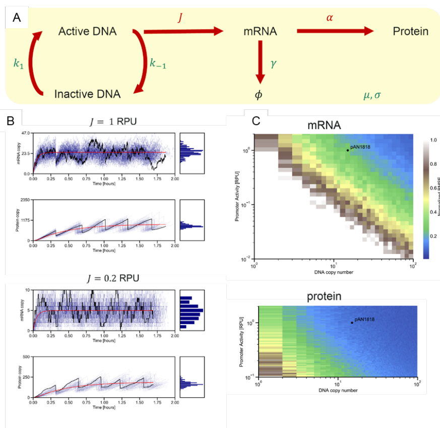
Figure 17. Stochastic simulation results (A) Schematic of two-state model describing transcriptional bursting (B) results of stochastic simulation for two promoters of different strength on a low copy plasmid. (C) root mean squared error of an entire population of cells for a range of DNA copy and promoter activity levels.
