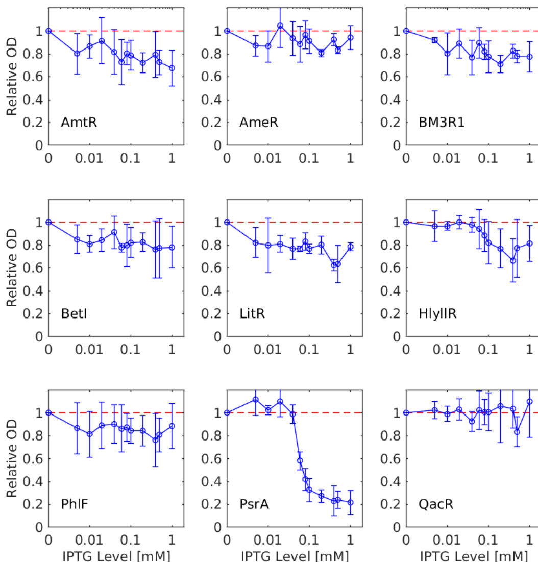
Figure 29. Toxicity of 9 genomically-integrated gates under different IPTG induction. PsrA is a gate that becomes highly toxic after high dose of IPTG.
