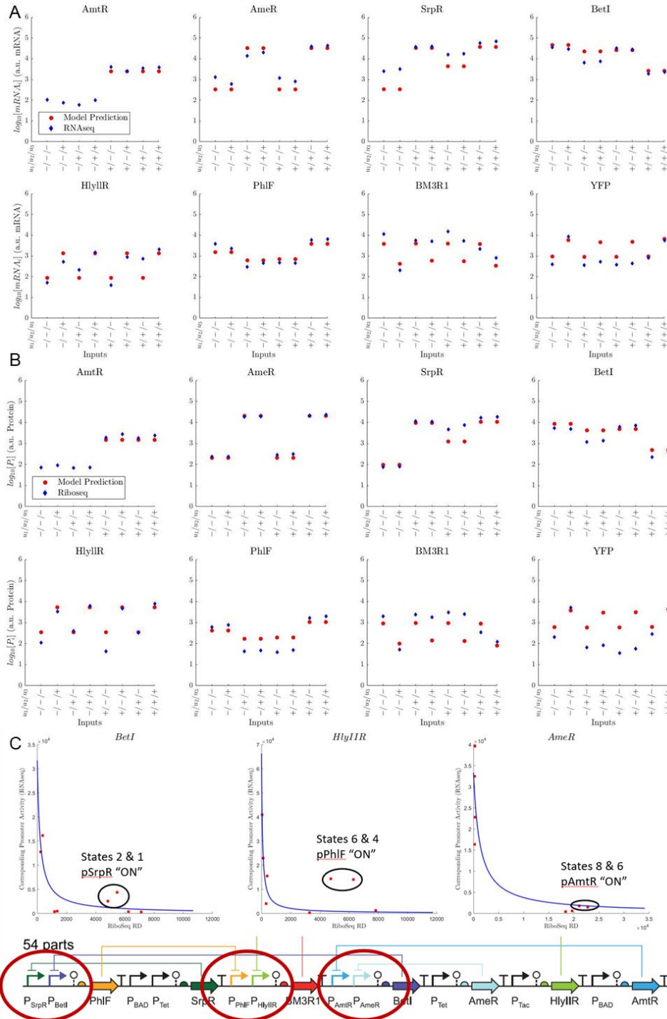
Figure 16. Predicted expression levels using the genetic circuit simulator (A) Prediction vs. Measured RNA-seq (B) Prediction vs. Measured protein expression (C) Tandem promoter effect
