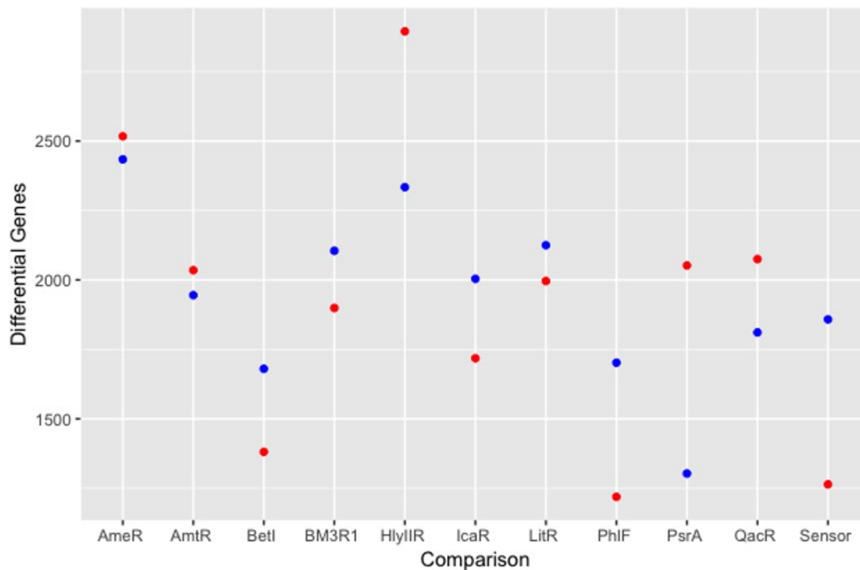
Figure 73. Differential expression of NOT gates to wildtype. Red - no induction, blue - induction. HlylIR had the highest differential expression followed by AmeR; the two gates least similar to the other gates. Most gates had slightly higher differential compared to the sensors alone.
