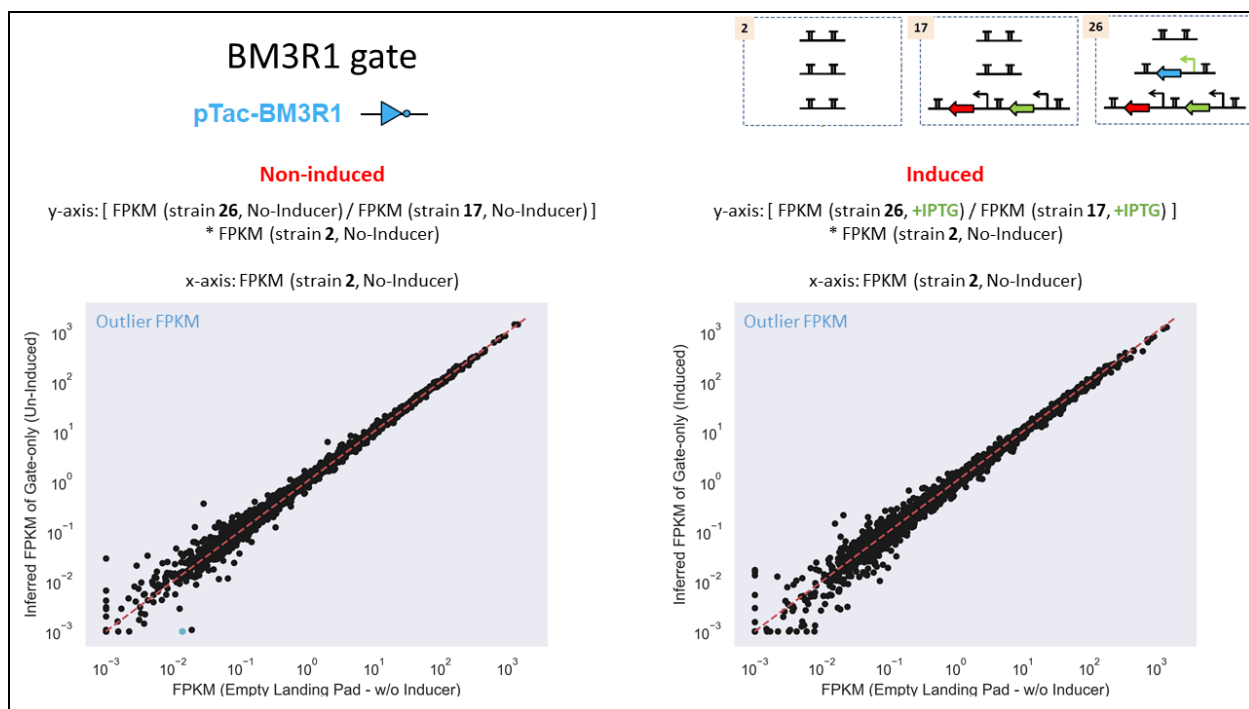
Figure 32. Exclusive impact of BM3R1 gate under induced and non-induced conditions.
