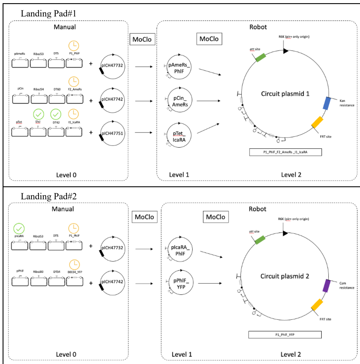
Figure 104. The two construction plans for the AND circuit presented in Figure 101. It considers two independent plasmid assemblies associated with their corresponding landing pad (#1 and #2). Modular parts are assembled manually or automatically using a liquid handling robot depending on the construction level of the MoClo assembly strategy.
