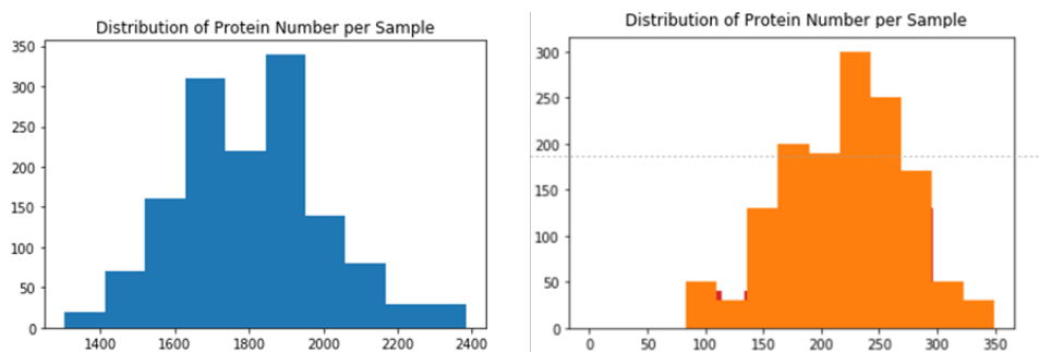
Figure 12. Results of high throughput proteomics experiments (A) Distribution of proteins with non-zero abundance value across samples in the proteomics data for NAND iterate and (B) same distribution for proteins that passed QC i.e. had confidence score > 10
