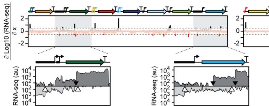
Figure 6. RNA-seq can identify cryptic promoters in both sense and antisense strands.
