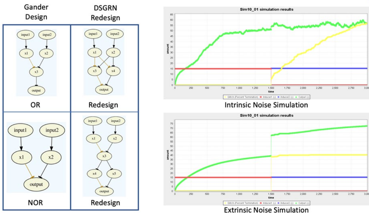
Figure 125. Extrinsic and intrinsic noise model genetic circuits failure predictions for two different DSGRN design layouts using iBioSim.
