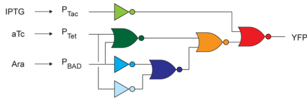
Figure 1. Circuit diagram of the genetic circuit used in this work.
