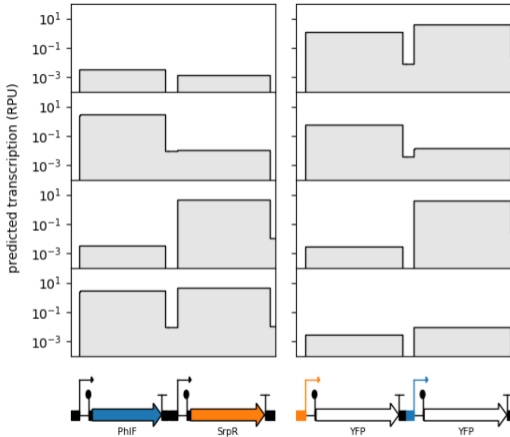
Figure 98. Cello2 generated a sample RNA-seq profile. The profile is for a NAND circuit. Each row of plots represents a particular input state. Each column represents a specific plasmid.
