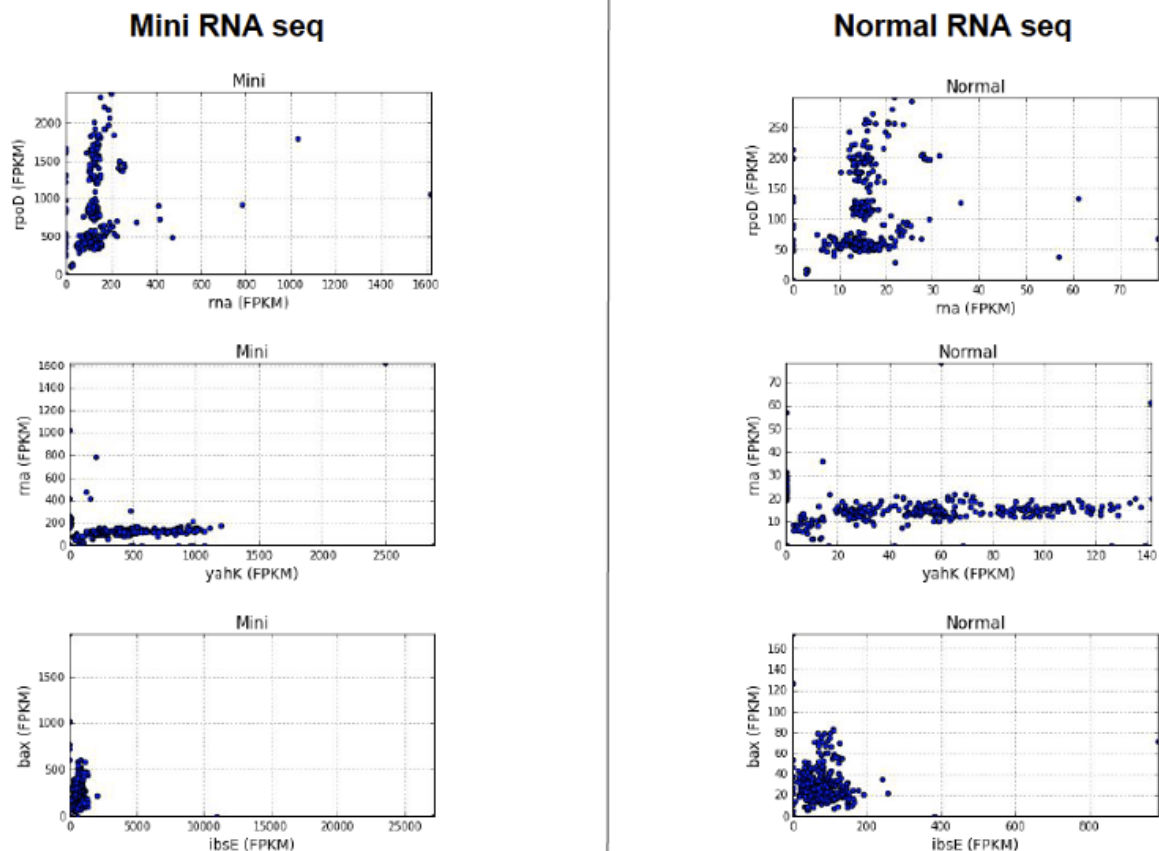
Figure 64. Genes comparison of mini and normal preparation kit using FPKM values
