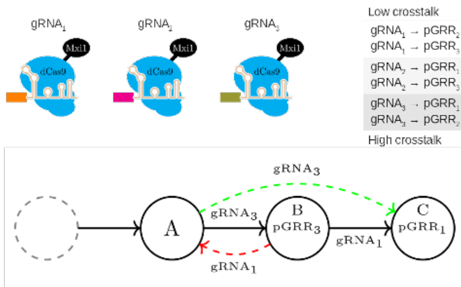
Figure 95. Example assignment of guide RNAs according to knowledge of crosstalk effects. The path from A to C is assumed to be least likely to hurt circuit function, and so it is assigned the guide RNA with the worst crosstalk behavior. The path from B to A is assumed to be the most likely to hurt circuit function, and so it is assigned the guide RNA with the best crosstalk behavior.
