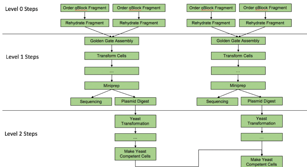
Figure 106. Visualization of an Operations Graph within Puppeteer. Each operation (green box) stores input parts, output parts, and a set of previous operations and subsequent operations.
