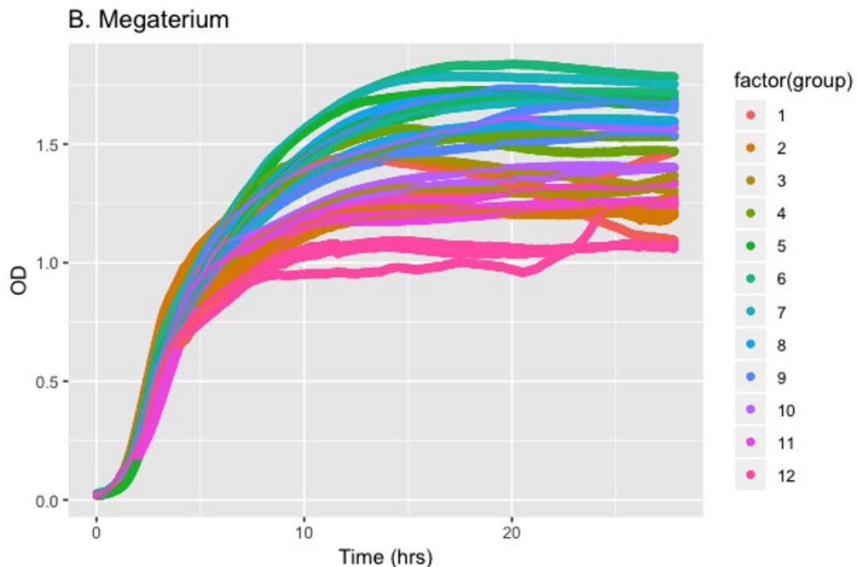
Figure 81 Mixed media growth in B megaterium. Group 1 is 100% LB, group 12 is 100% M9CA with intermittent groups representing 10% shift from LB to M9CA (2 is an exception as it is 5% due to having 1 extra column). Media composition between LB and M9CA had minimal effect on the growth rate, while having a much bigger effect on carrying capacity and time in log-phased growth. This is ideal for selecting times to compare media as the growth rates will be similar (as long as a time is selected while in log-phased growth).
