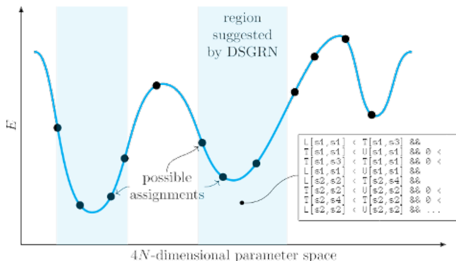
Figure 94. DSGRN suggests regions of parameter space for Cello to investigate. A region of parameter space corresponds to a set of inequalities on Hill-function parameters that would implement the given truth table.
