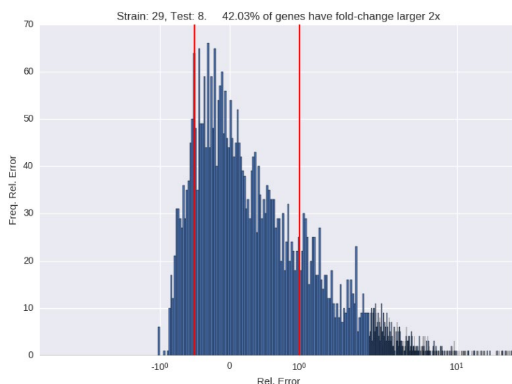
Figure 48. Accuracy of whole genome simulator for a NAND circuit at stationary phase. The distribution of relative errors for predicted expression of all native genes in strain 29 when both IPTG and arabinose are present and growth is at stationary phase. Red lines depict the 2-fold error thresholds.
