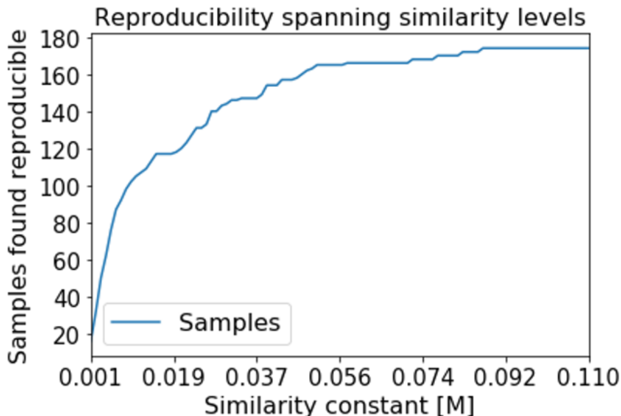
Figure 86. Scanning the precision constant from 0.001 to 0.11 we observe how samples begin forming groups. This can be expanded upon by using the percent reproducibility per group to get an idea of how precise a reproducible result is, but this idea needs more data to assess.
