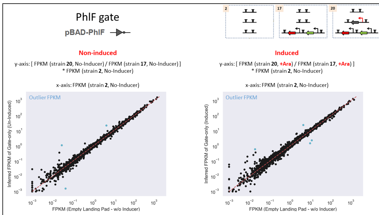
Figure 33. Exclusive impact of PhlF gate under induced and non-induced conditions.
