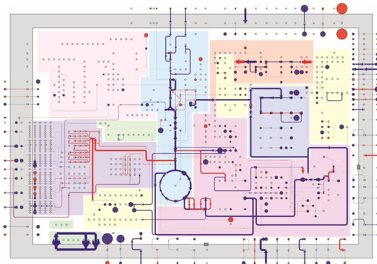
Figure 42. The metabolic network of E. coli .
