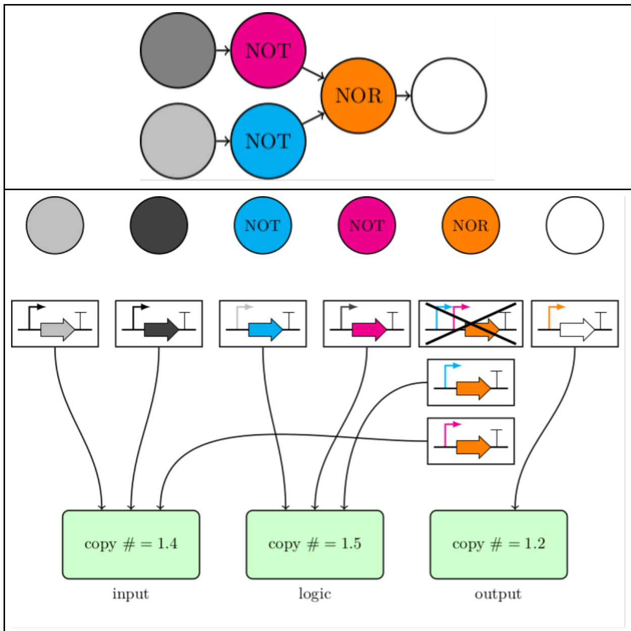
Figure 96. Tandem promoter splitting. The NOR gate transcriptional unit with tandem promoters is split into two, and one unit is reassigned to a different location.
