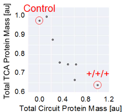
Figure 39. Impact of the circuit on TCA cycle enzyme levels.
