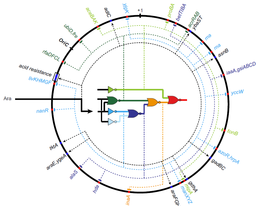
Figure 38. A complete map of circuit's non-specific impacts on E. coli genome. Dashed lines with arrow heads mean activation, while dashed lines with stopping-line head represent repression.
