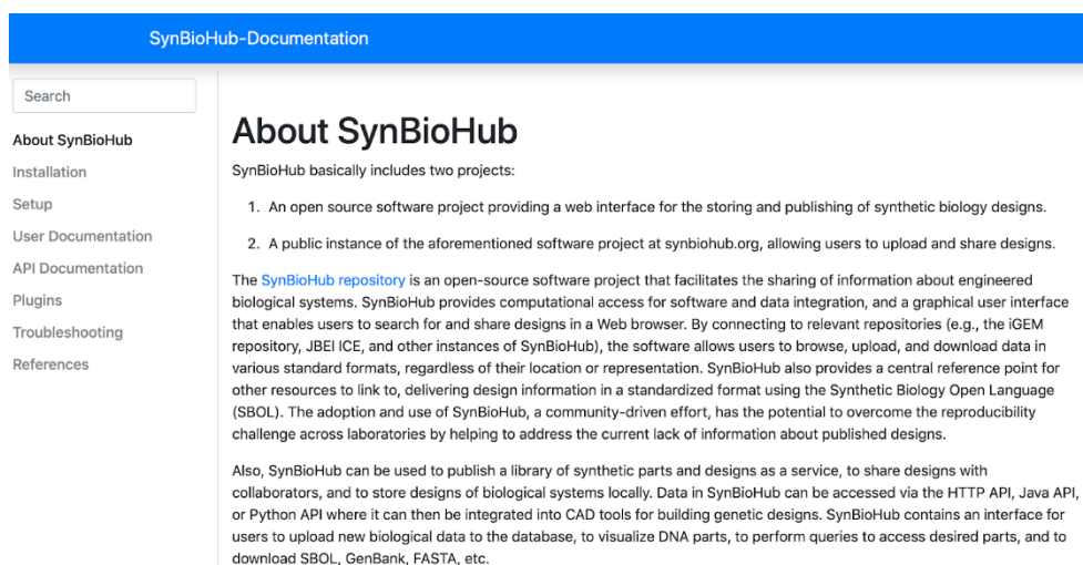
Figure 114. SynBioHub's new documentation found at https://synbiohub.github.io
