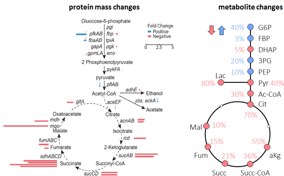
Figure 41. Metabolomics data confirms the Ribo-seq results. As the expression of enzymes in TCA decreases, the concentration of metabolites involved in their enzymatic reaction also decreases. Plot are generated by comparing +/+ state with the control.
