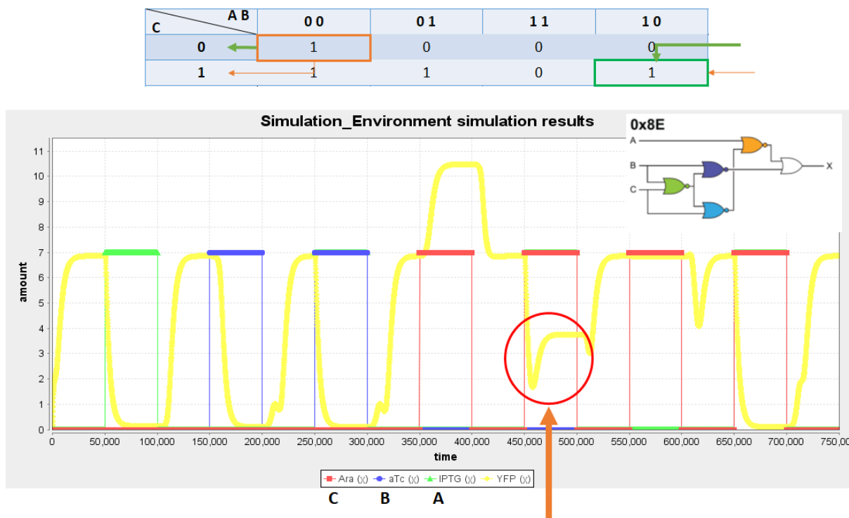
Figure 121. Example of a function hazard in a genetic circuit design. In this circuit, when A (IPTG) and C (Ara) go high simultaneously, this creates a race through the logic. Namely, if the change on C is felt first, the circuit remains outputting a high value, but if the change on A is felt first, there will be a glitch to a low value on the way to the final high state. This glitch is observed in the dynamic simulation generated by our model generation procedure. This race is known as a function hazard, and these are inherent to the Boolean function being implemented. There is no logic implementation that can eliminate this function hazard. The only solution is to restrict the order of input changes (for example, require C to be set high before A).
