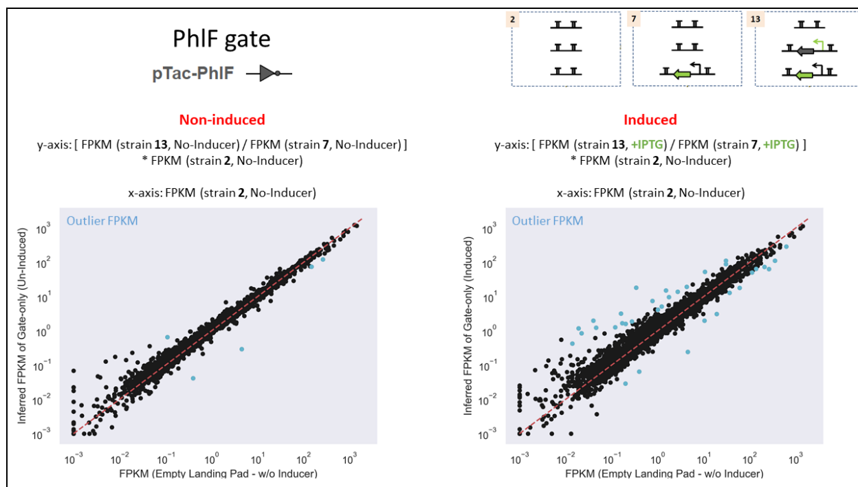
Figure 31. Exclusive impact of PhIF gate under induced and non-induced conditions. The quantification formula is shown. Schematics of strains used in the formula are shown in top right. Each box represents a strain with three landing pads in the genome (from bottom to top: sensor landing pad, repressor landing pad, YFP landing pad). The x-axis is the measured genomic FPKM data from the control strain 2 (empty landing pads), and y-axis data is the predicted genomic FPKM of the repressor. A long list of outlier genes with significant deviation from x=y are marked with blue color in the induced-state of PhIF.
