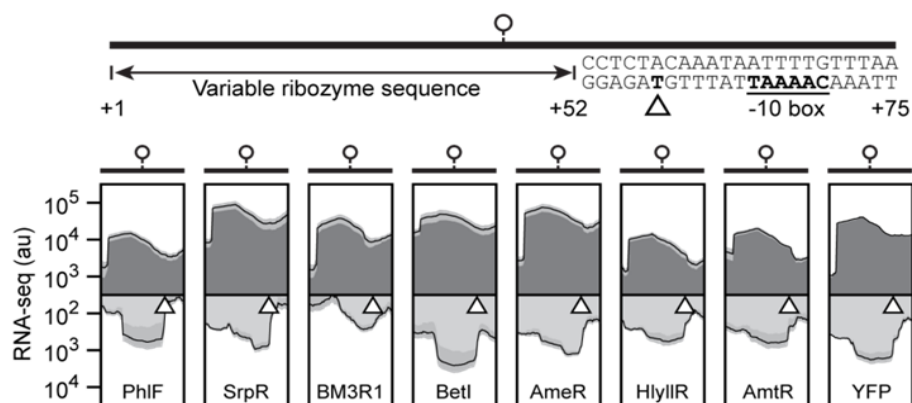
Figure 7. Cryptic antisense promoter inside ribozymes. A cryptic antisense promoter is hidden in all ribozyme sequences in the circuit, which causes about 5-fold reduction in sense transcription.
