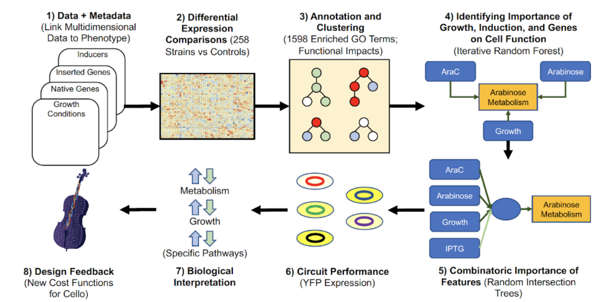
Figure 70. RNASeq pipeline for identifying functional impacts of circuits on cell hosts
