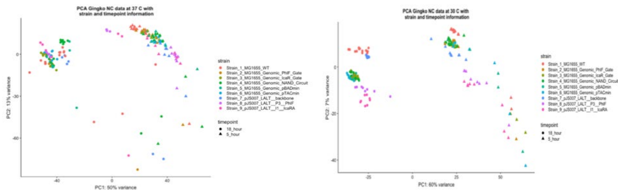
Figure 65. Comparing Gingko generated data across 37°C and 30°C
