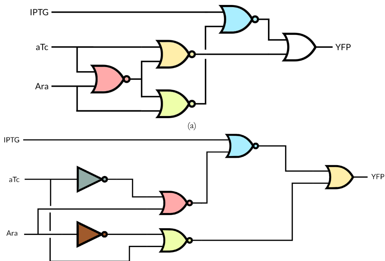
Figure 122. Original and Alternative Circuit Designs (a) Original Cello design of the circuit 0x8E. (b) Alternative design of circuit 0x8E that is free of logic hazards.
