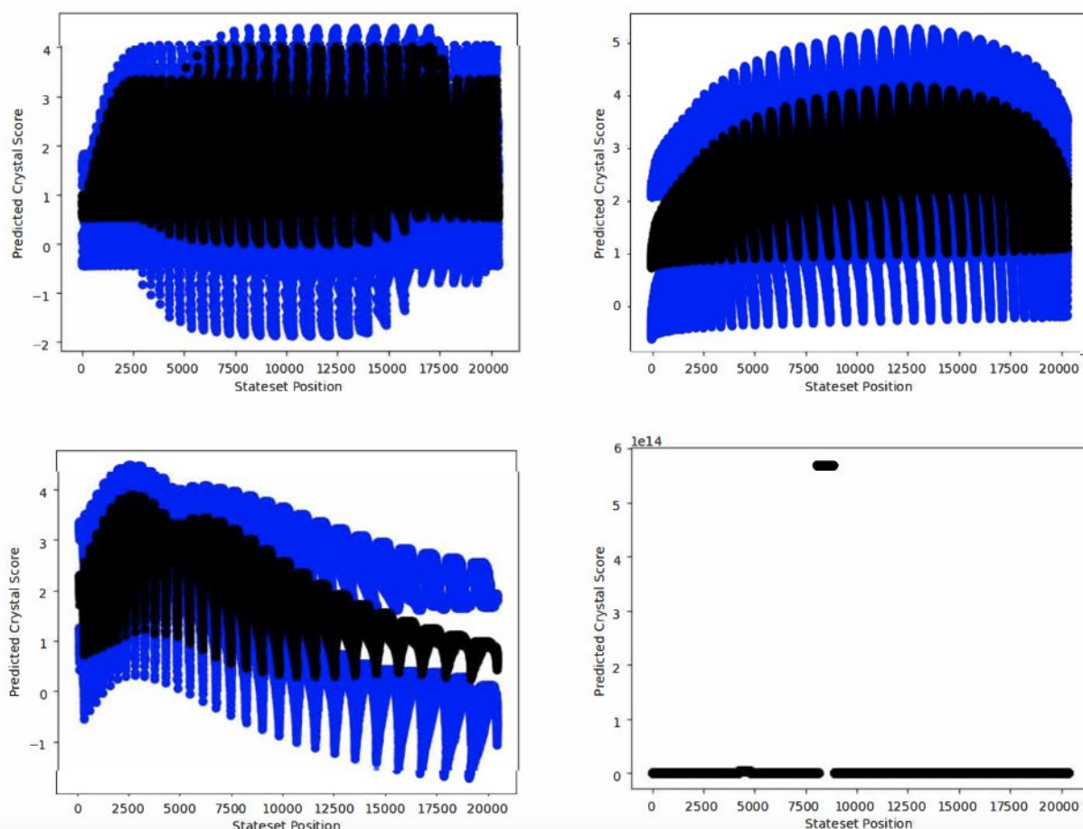
Figure 88. 2d representation of four different models after the last active learning stage. Black represents the predicted crystal score for the set of acid, organic, and inorganic concentrations at a given stateset point, while blue represents the standard deviation of that score. Higher values tend to have lower standard deviations due to the model intentionally over exploring areas that are likely to produce crystals. The model representing the underlying space is not necessary to accurately identify areas that are likely to produce crystals as maxima are explored rather than raw values. However, this is not the case for serendipity where more of the space is explored.
