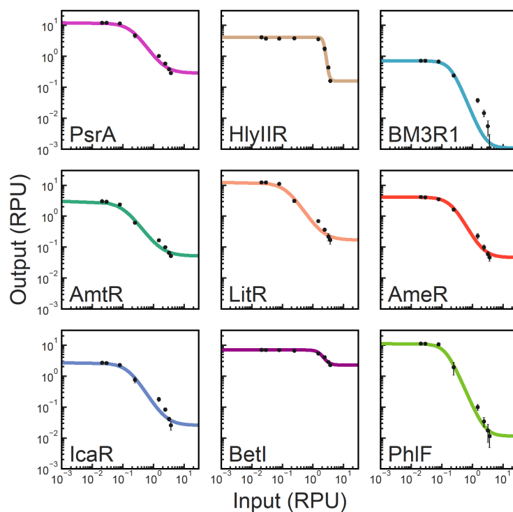
Figure 60. Response function of genomic-integrated NOT gates in E. coli Nissle. Lines are best fits to a Hill function.
