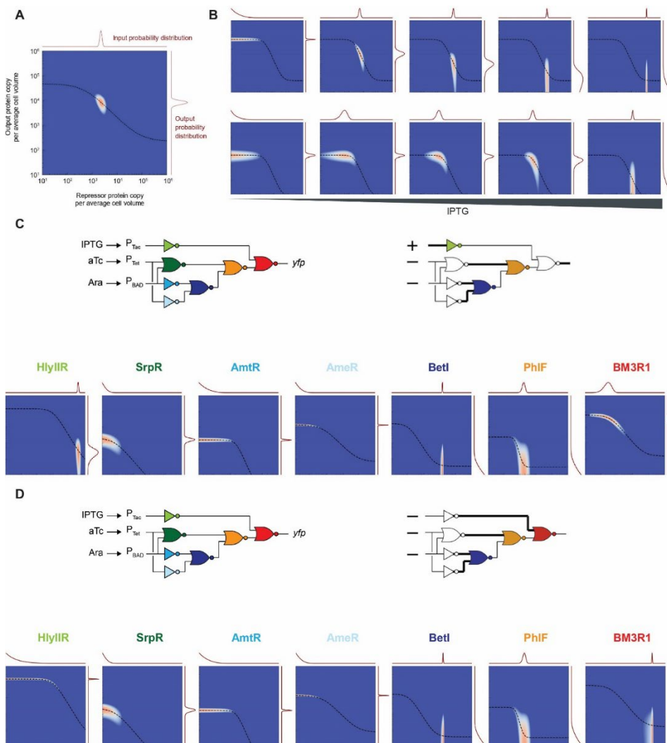
Figure 18. Simulations of noise propagation using stochastic gene expression model (A) Noise propagation through an example gate; x-axis is the repressor protein copy normalized for cell volume, y-axis is the output protein copy also normalized, the dashed black line shows the expected deterministic response function, the heat map shows the predicted distribution of cells within a population (blue to white to orange showing increasing fraction – the blue-white boundary can be thought of as likelihood equivalent to a single cell in 1ml culture at OD=1.0). The normalized probability distributions of expression level of the repressor is shown at the top and the output protein at the right. (B) Noise propagation plots for the AmeR gate on a plasmid (top row) and on the genome (bottom row). (C,D) Noise propagation plots for the 0x41 Circuit in an on state and off state
