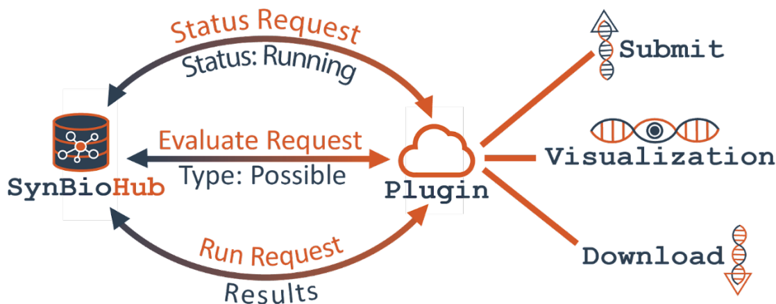
Figure 113. SynBioHub Plugin Architecture.
