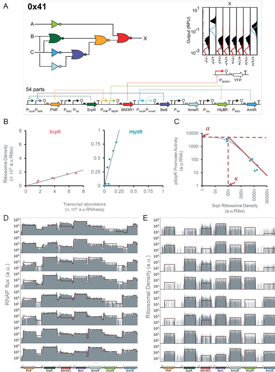
Figure 14. Part characterization using genetic circuit analyzer and steady state simulations (A) Cello designed circuit 0x41 showing the logic representation (top left), the genetic parts representation (bottom), and the predicted and experimental YFP output (top right).
