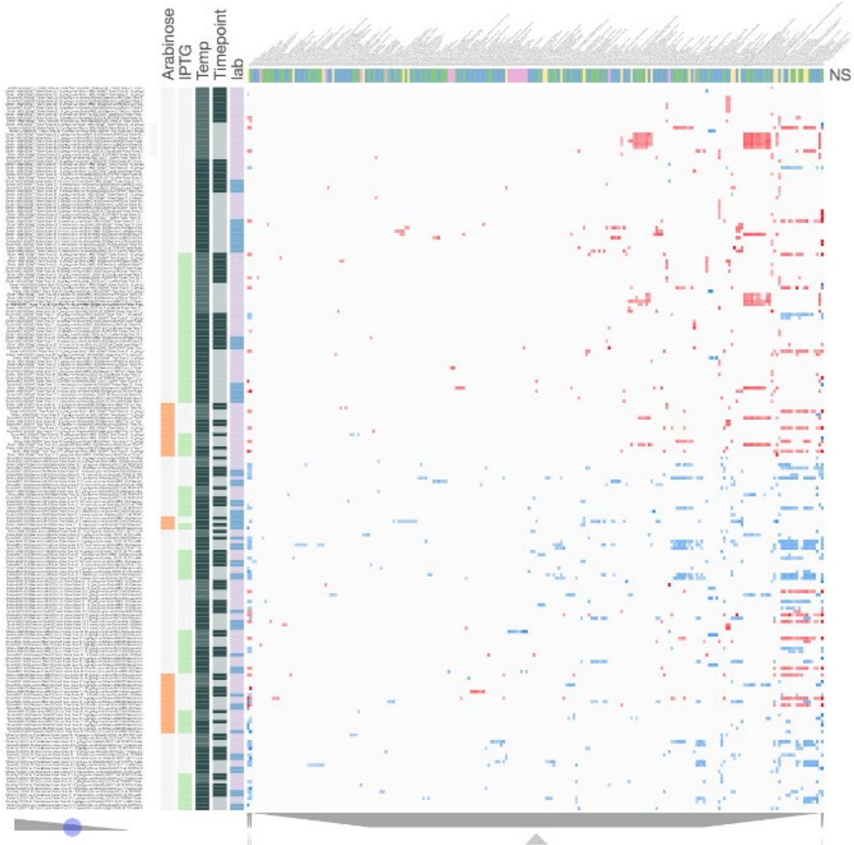
Figure 68. A matrix visualization of all annotated up-regulated and down-regulated GO and KEGG terms for differential tests using factors Arabinose, IPTG, Temp, Timepoint, and lab. The GO and KEGG terms are on the top as columns and the differential tests are displayed as rows. The column and row information is displayed when hovering over a specific cell in the matrix for quick look-up. Categories on the rows and columns can be re-sorted by double-clicking the corresponding category term. The visualization can be cropped to zoom in on an interesting region. A slider (below row names) offers the ability to change which depth of the clustering dendrogram is displayed beneath the x-axis, used to quickly crop the matrix to a cluster.
