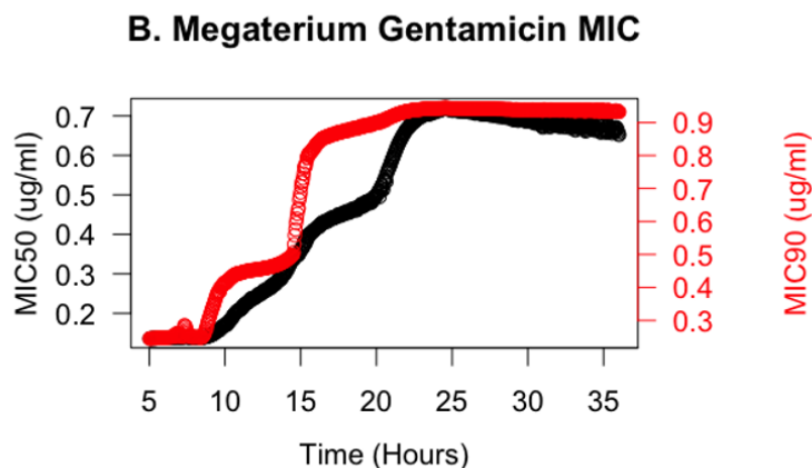
Figure 79. MIC50 (shown in black) and MIC90 (shown in red) are consistent (less and a 2x difference in MIC) for most of the times measured. Gentamicin would be one of the preferential drugs for synthetic selection in B. megaterium .
