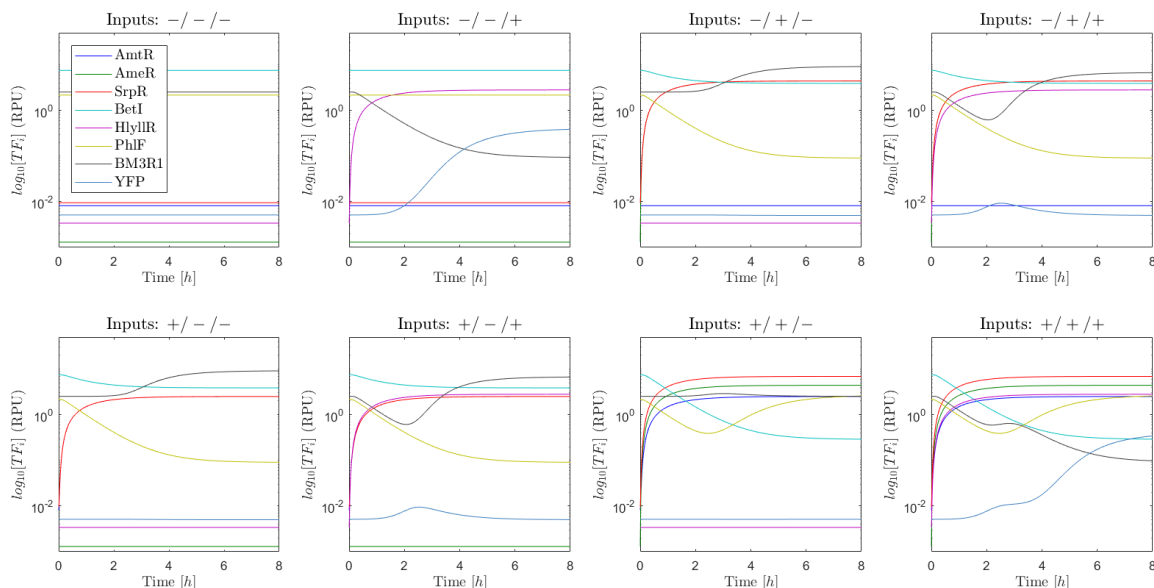
Figure 15. Predicted temporal profile of gene expression
