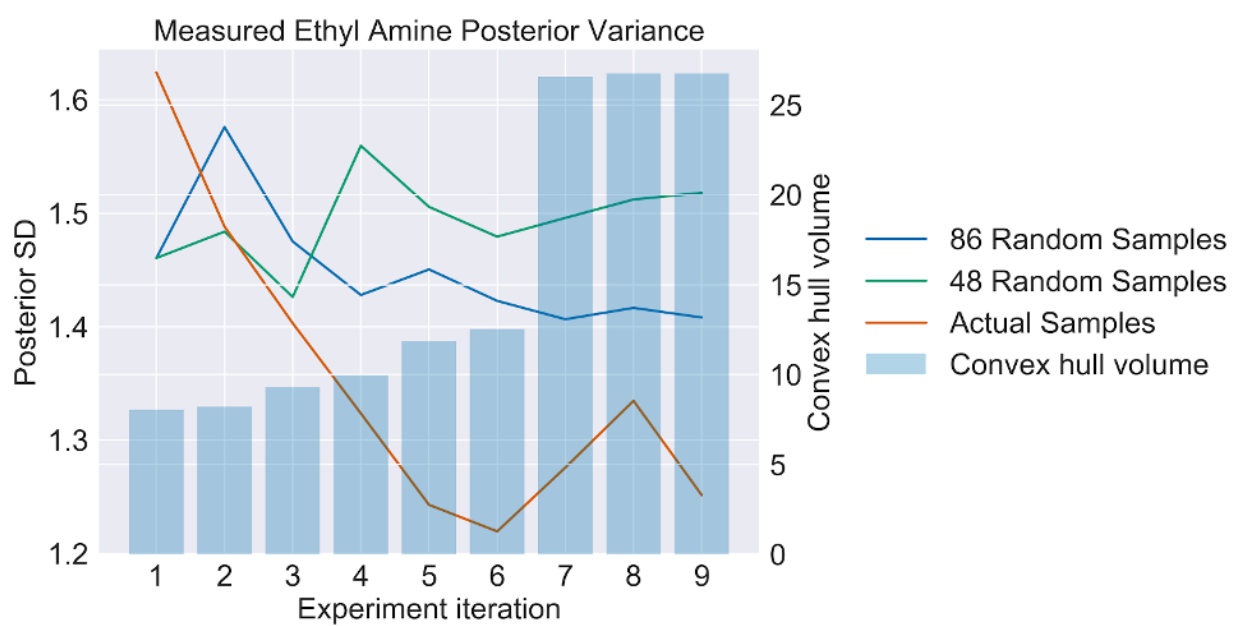
Figure 84. Rate of change in the convex hull volume explored based on the number of additional experimental points seen
