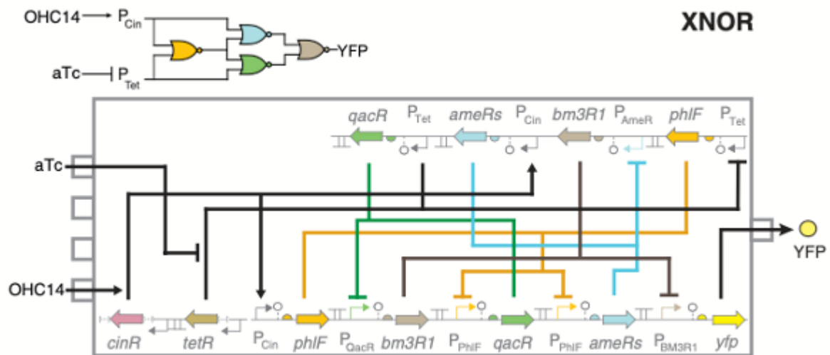
Genetic Circuit Schematic (from Park et al., 2020)
