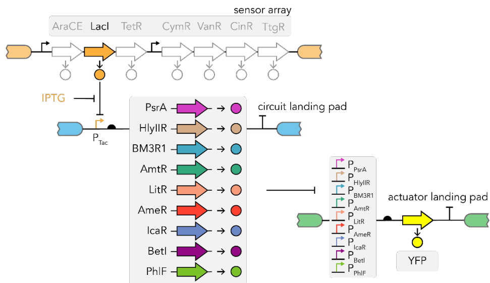
Figure 59. 9 separate genome-integrated NOT gates in E. coli Nissle.
