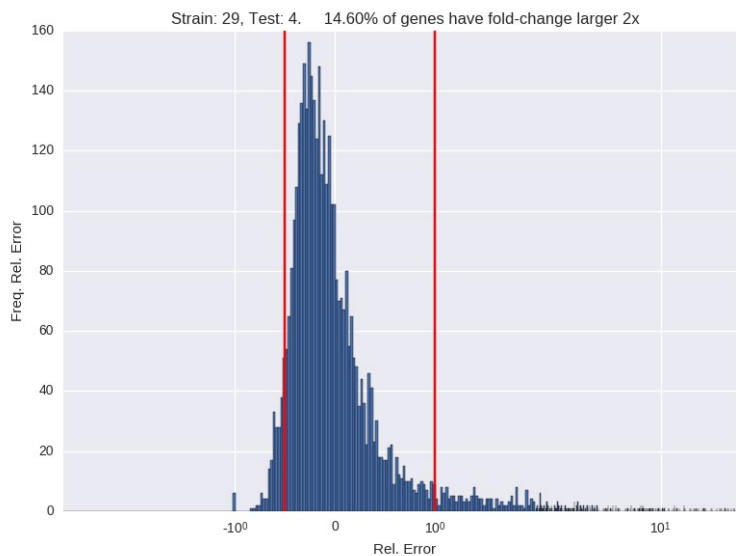
Figure 46. Accuracy of whole genome simulator for a NAND circuit in exponential growth. The distribution of relative errors for predicted expression of all native genes in strain 29 when both IPTG and arabinose are present and growth is at exponential log phase. Red lines depict the 2-fold error thresholds.
