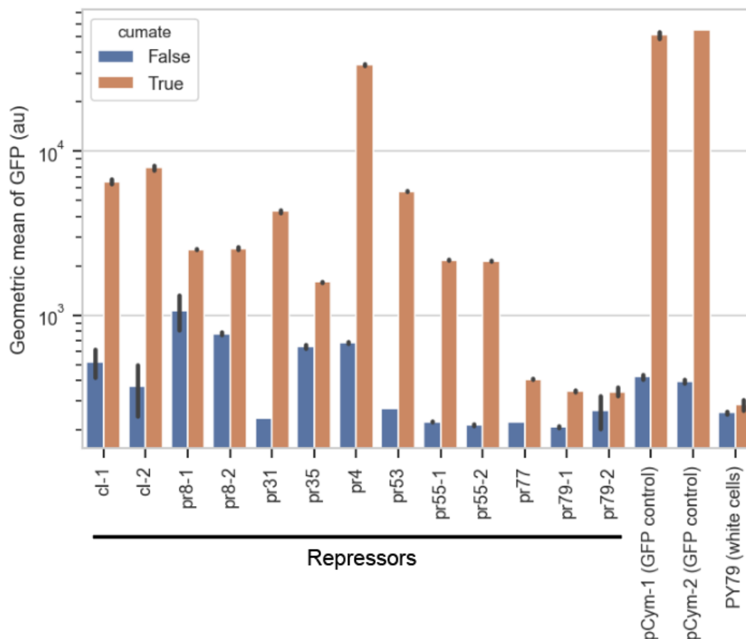
Figure 52. Characterization of Phage-based gates in B. subtilis . The measured fluorescence of sensor and phage-based gates in B. subtilis in the presence and absence of cumate inducer.
