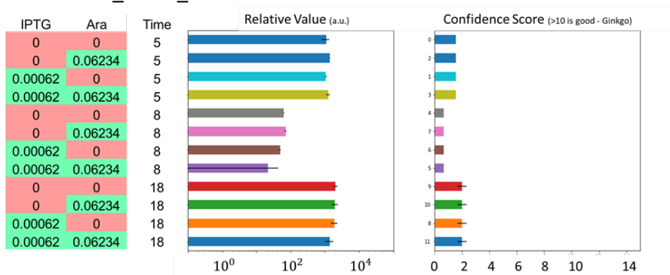
Figure 13. IcaR expression for three strains
