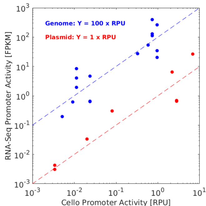
Figure 25. Comparison of promoter activities using RNA-seq and Cello, values derived from flow cytometry
