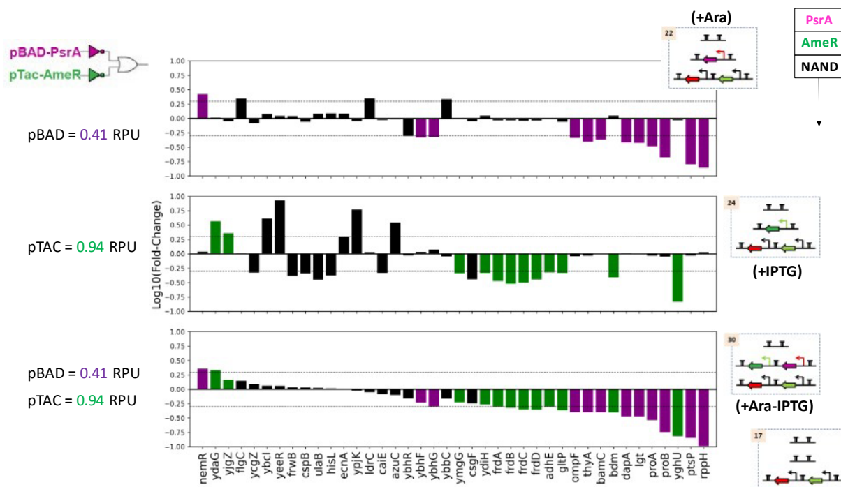
Figure 35. List of regulated genes in PsrA-AmeR NAND circuit.
