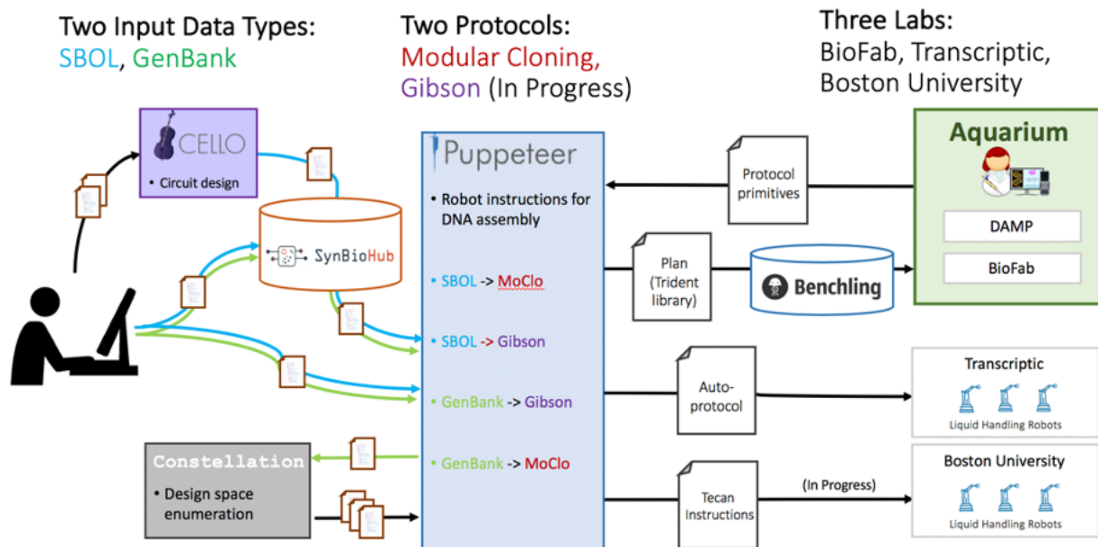
Figure 107. An architecture diagram shows Puppeteer's workflow and integrations with other software tools. The design process starts with a user creating a circuit design in Cello and uploading the SBOL output to SynBioHub. Puppeteer retrieves and parses the SBOL. Then, a user can select from a list of available cloning methods, including Modular Cloning and Gibson, and an output type, which can be Aquarium operations (BU DampLab or UW Biofab) or liquid handling robot instructions (Autoprotocol or Tecan). DNA sequence data is also uploaded to Benchling for Aquarium operations.
