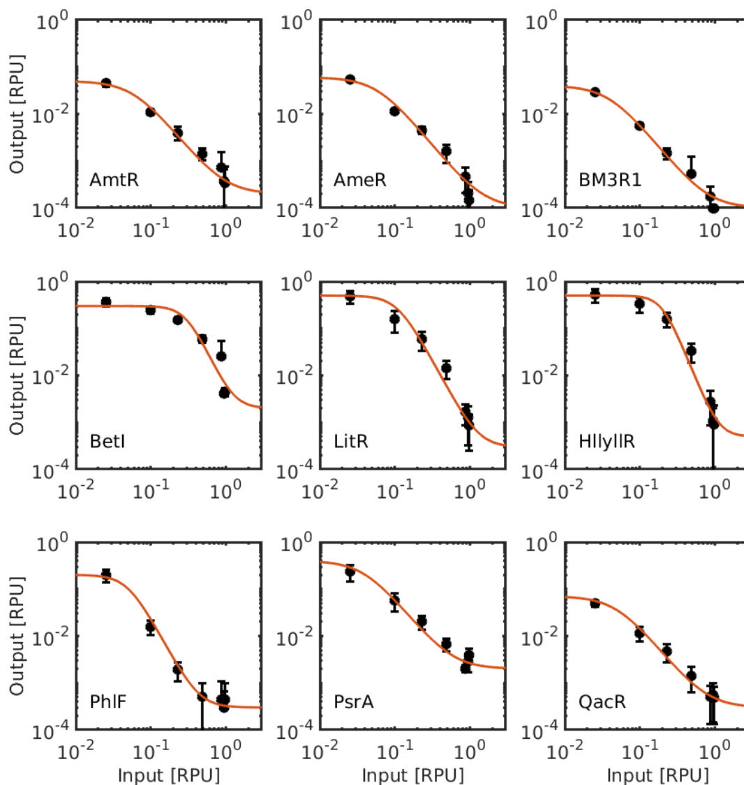
Figure 28. Response function of 9 genomically-integrated gates. Data is the average of 3 measurements in separate days. Red line is the best fit using a Hill equation.
