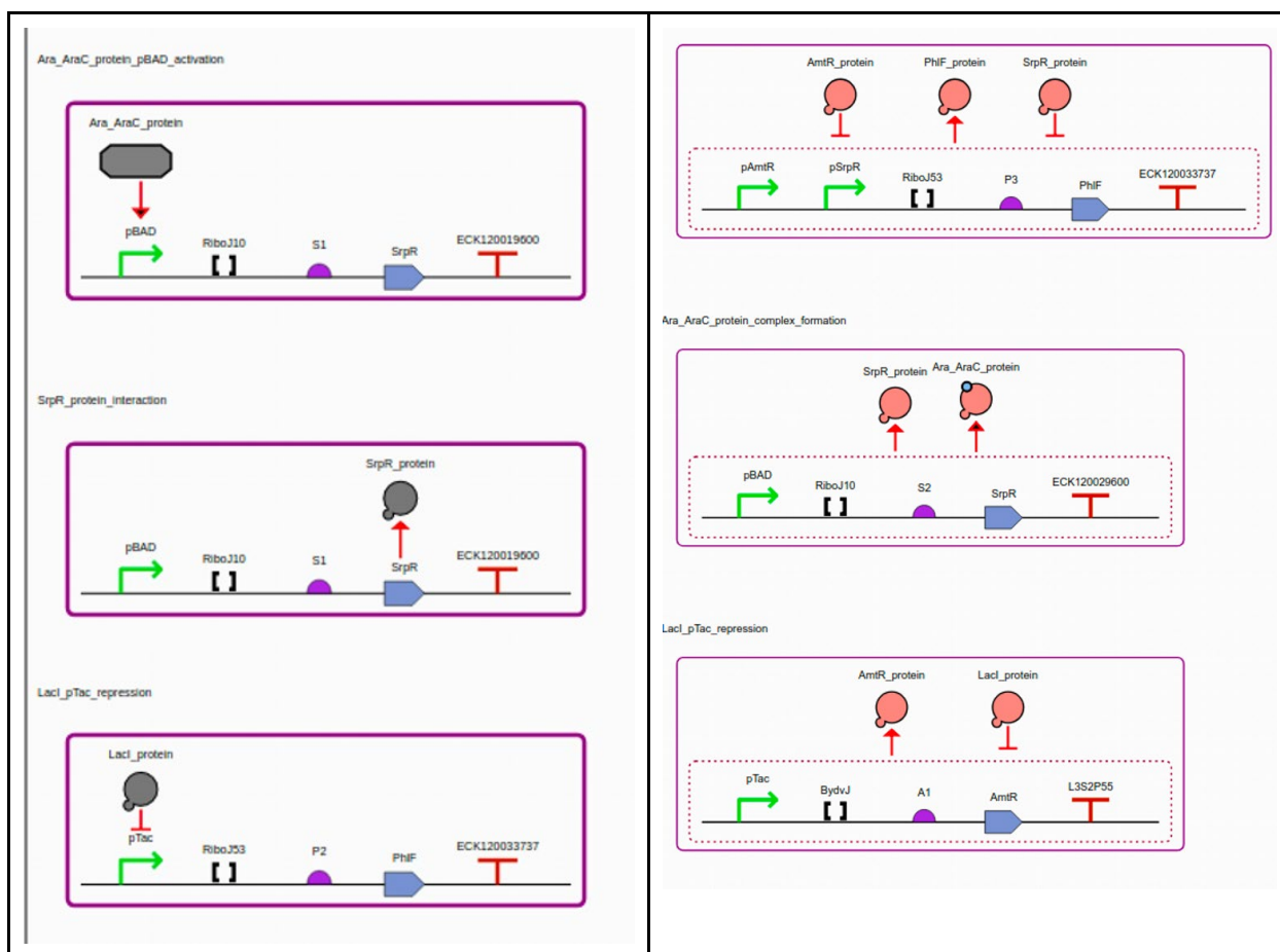
Figure 110. Previous vs. a current rendering of interactions in VisBOL. On the left is the previous implementation, where the non-DNA component sat directly on top of the part of the DNA where the interaction occurred. Unfortunately, the assumptions made in this approach often led to erroneous renderings and cannot currently be fixed due to SBOL limitations. On the right is the current implementation, where the non-DNA components are shown above the entire circuit.
