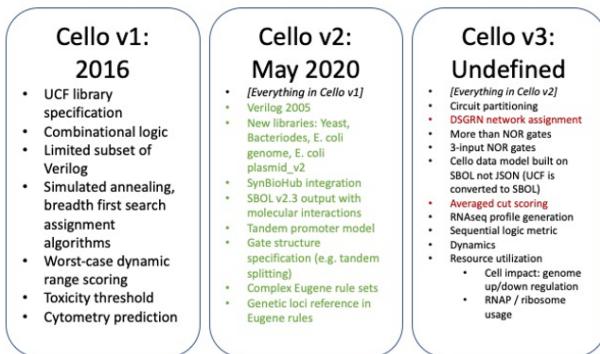
Figure 89. Roadmap of Cello releases.
