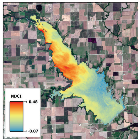
Normalized Difference Chlorophyll Index (NDCI) for July 8, 2021
