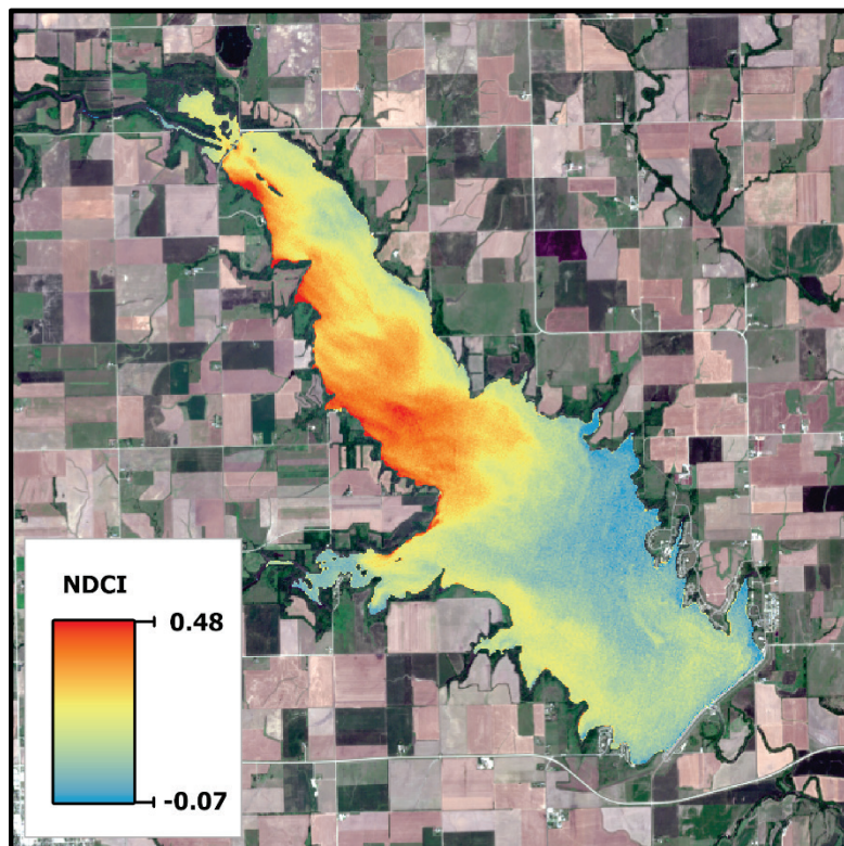
Figure 12. NDCI output for Marion Reservoir, Kansas for 8 July 2021.
