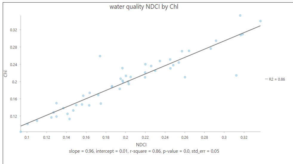
Figure 15. Linear regression graph comparing NDCI relative index values to hypothetical (synthetic) chlorophyll-a sample values (in situ); sample .svg graph output.
