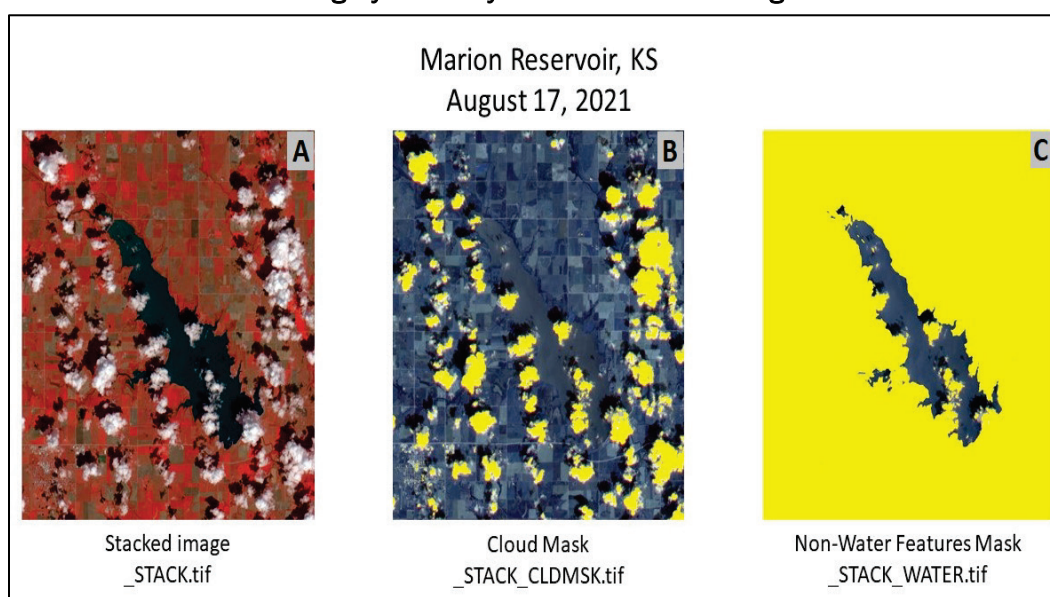
Figure 10. Sentinel-2 imagery of Marion Reservoir, Kansas for August 17, 2021. A.) Sentinel-2 stacked image -bands 1-8A with no mask applied, B.) Cloud Mask – yellow areas represent the removal of clouds from the imagery, C.) Non-Water Features Mask – yellow areas represent all features (including clouds) removed from the imagery with only water areas remaining.
