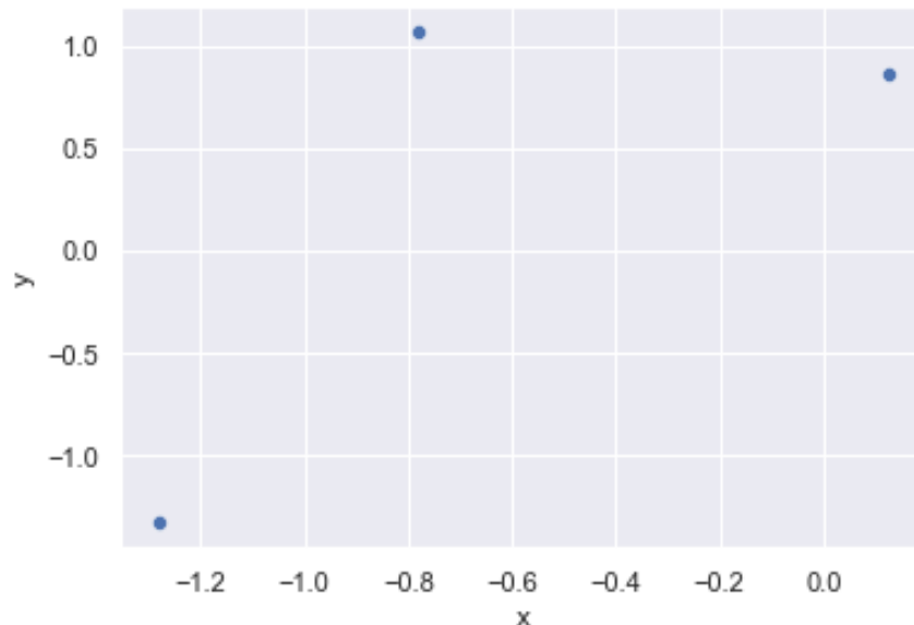
Figure 3.4: 1S 2D KS Test Data Example
