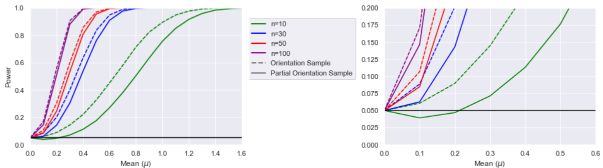
Figure 3.35: 1S 2D KS Test Sample Methods Mean Power \alpha = 0.05
