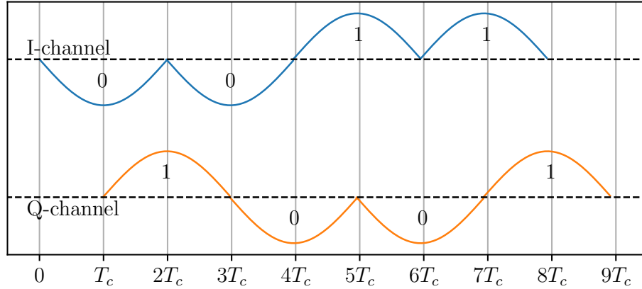
Figure A.2. Example of O-QPSK half-sine pulse shaping with I- and Q-channels for bit sequence [0,1,0,0,1,0,1,1] . Note that bits are transmitted on alternating channels, where the quadrature component is delayed by T_c .
