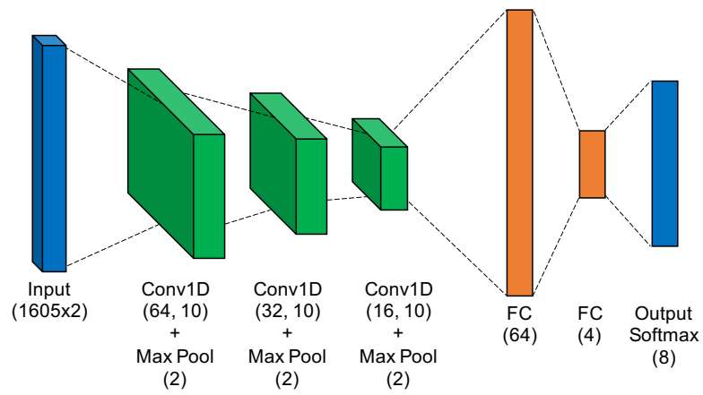
Figure 7. Low-Capacity Convolutional Neural Network.
