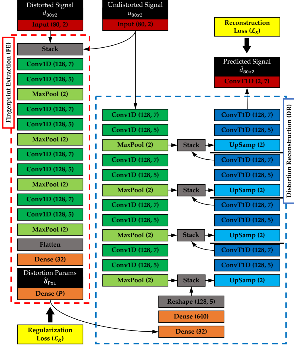
Figure 20. FEDR Network Architecture. The only information passed from the Fingerprint Extractor (FE) to Distortion Reconstructor (DR) are the undistorted signal and the parameters. Model is trained end-to-end to minimize \mathcal{L}_S and \mathcal{L}_R .
