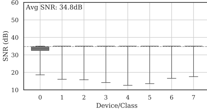
Figure 17. Summary of estimated collection SNRs for all classes across all channels after adjusting SNR to 35 dB. The mean SNR dropped to 34.8 dB, as denoted by the dotted line.
