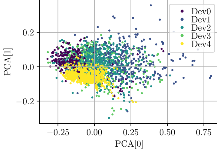
Figure 29. First and second PCA elements of FEDR-16 parameter space for 5-class RFF. Minor clustering is visible for some of the classes, but most of the hyperspace separability is nonlinear.
