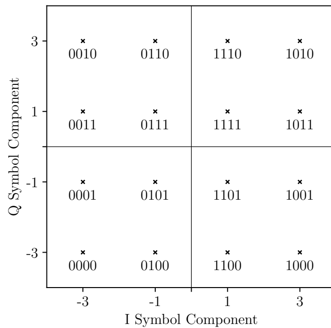
Figure A.5. 16-QAM symbols with corresponding bit sequences.
