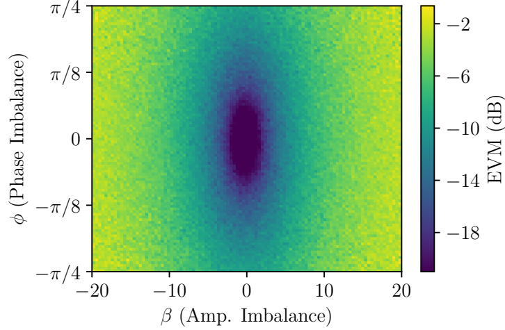
Figure 23. EVM for OFDM+16-QAM with amplitude ( \beta ) and phase ( \phi ) imbalance. The dark region in the middle is the target zone for the synthetic distortion, where EVM less than -16 dB, within the operational parameters specified by IEEE 802.11a/g.
