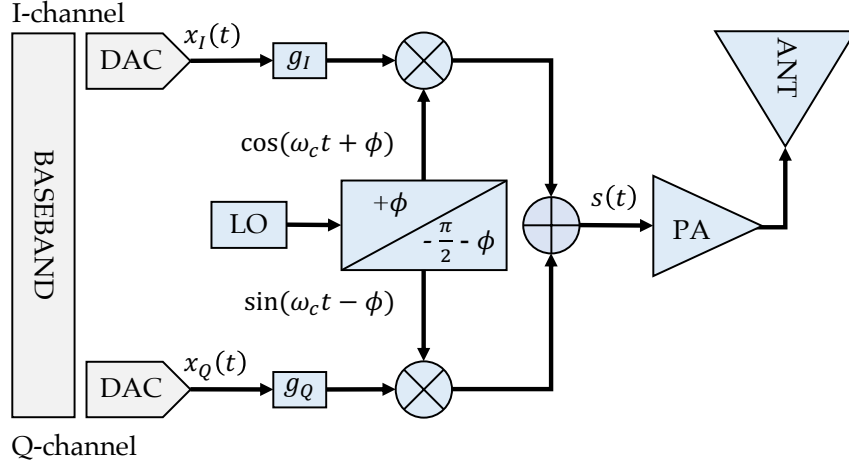
Figure 22. Typical Transmitter Architecture. IQ imbalance comprises amplitude and phase imbalances between the in-phase (I) and quadrature (Q) channels. These imbalances have been shown in recent research to contribute significantly to RFF [50].
