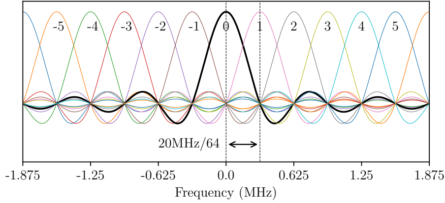
Figure A.4. OFDM subcarriers in frequency domain. Subcarriers -5 to 5 are shown, with 0.3125 MHz spacing between them, enabled by a 3.4 \mu s burst length.
