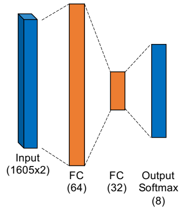
Figure 6. Fully-Connected Artificial Neural Network.
