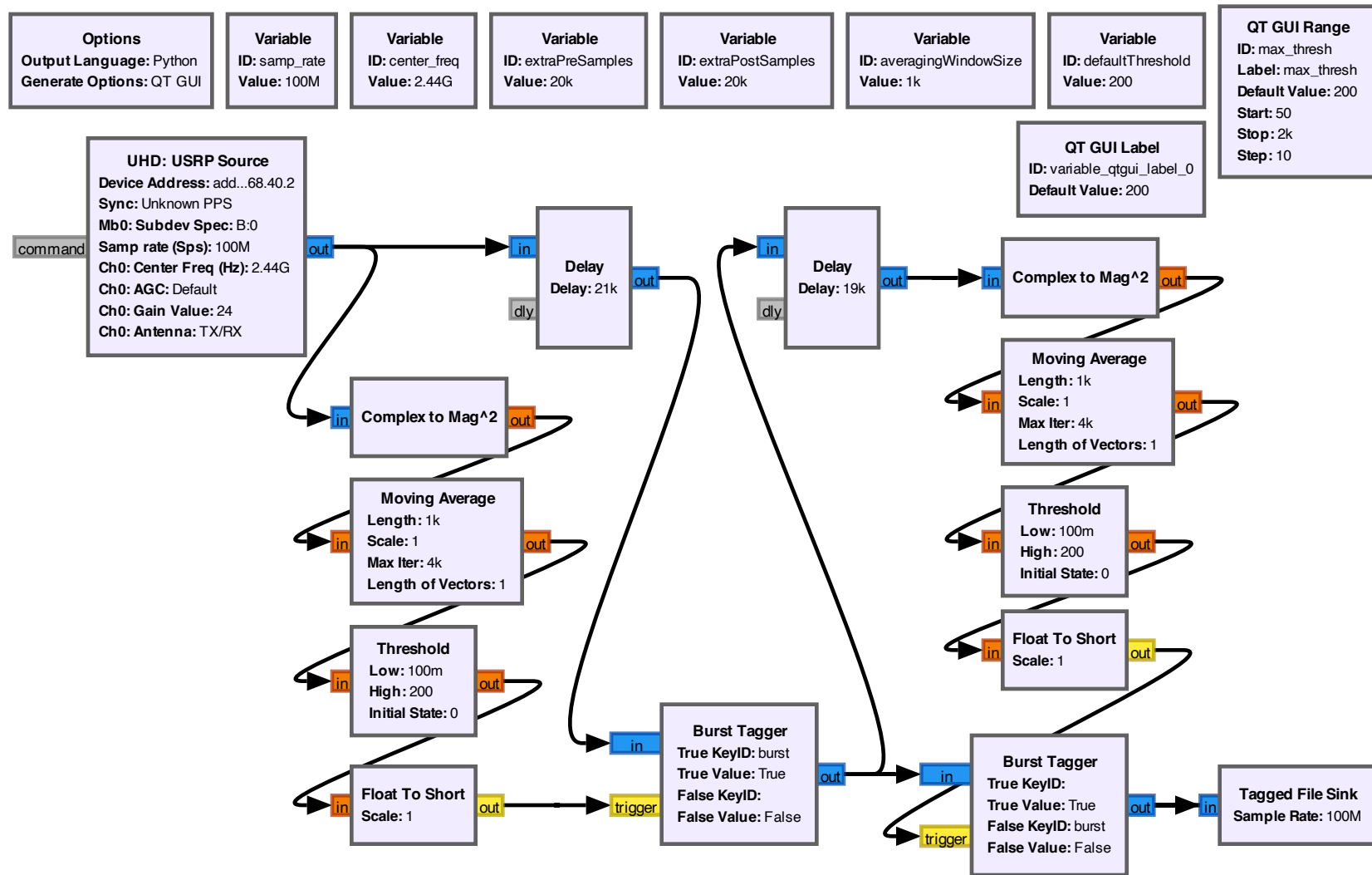
Figure C.1. GNU Radio Companion visualization of on-the-fly data collection and burst detection technique. The technique works by delaying the primary signal path to detect bursts, tagging a burst start and burst end position, and saving the information between the tags to hard drive.
