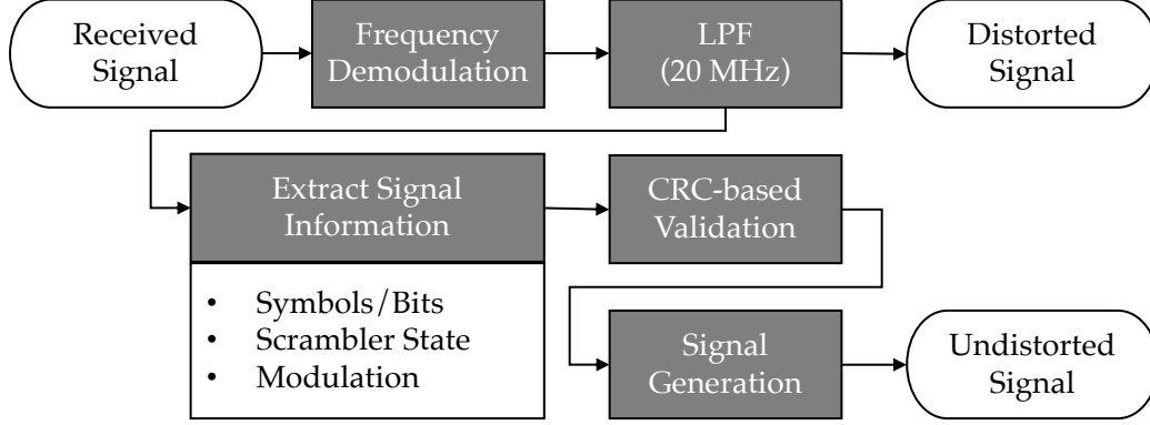
Figure 26. Overview of real-world signal pre-processing in preparation for machine learning. Parameters required for signal generation are the original symbols/bits, the initial scrambler state, and the OFDM symbol modulation type [2].
