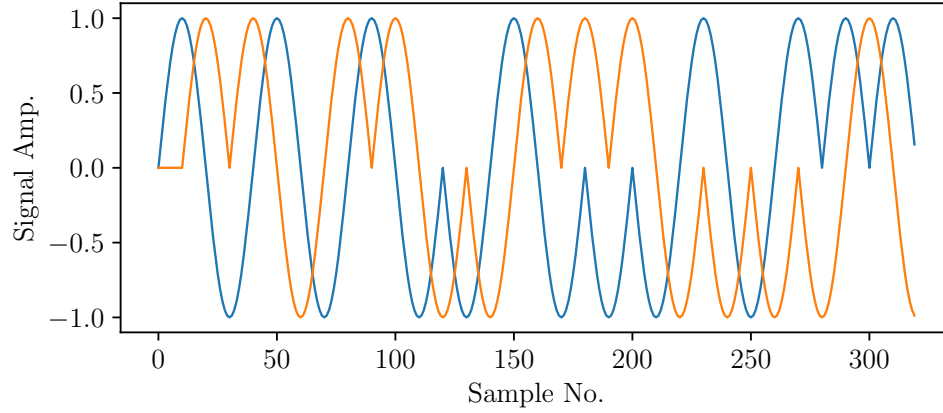
Figure A.3. First “0” symbol of an O-QPSK preamble.
