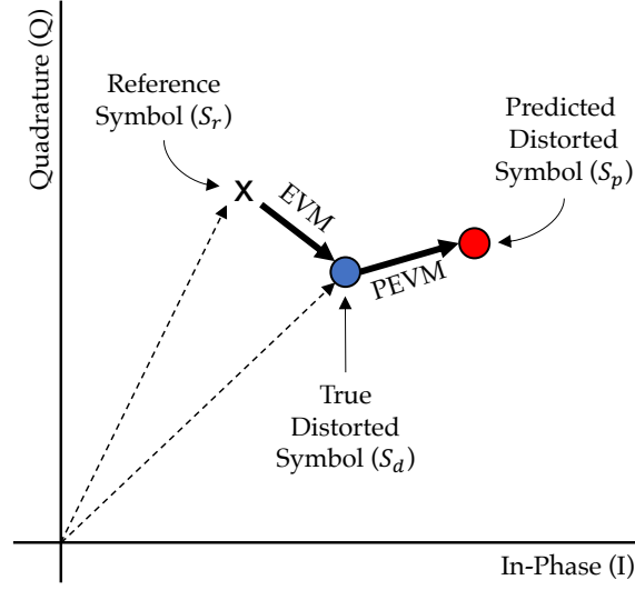
Figure 21. EVM and PEVM. Typically error is measured between the distorted symbol and the undistorted symbol (EVM), but the important error for this application is the distance between the distorted symbol and the prediction of the distorted symbol (PEVM).
