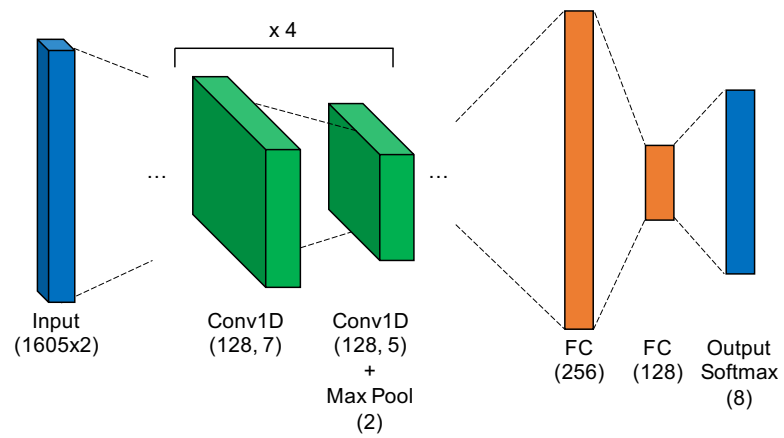
Figure 8. High-Capacity Convolutional Neural Network.
