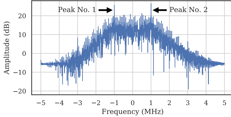
Figure 2. FFT of the square of a WirelessHART burst with yielded peaks. Centering the peaks about 0 MHz center-aligns the carrier and corrects the frequency offset.
