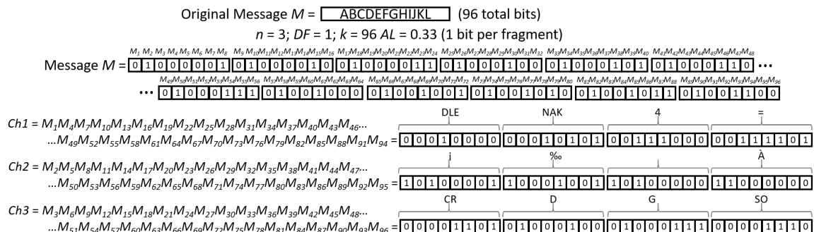
Figure 11. 1-Bit Fragmentation of Original Message Across Three Channels.
