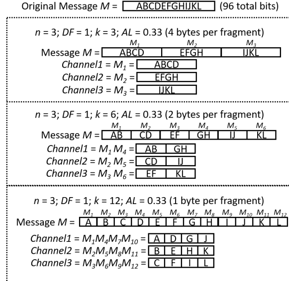
Figure 9. Byte-wise Fragmentation of Original Message Across Three Channels.
