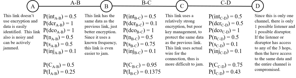
Figure 14. A Single-Channel, Three-Hop Network and QoSS Metrics.
