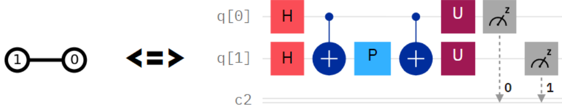
Figure 54: The QAOA circuit associated with the K_2 graph.
