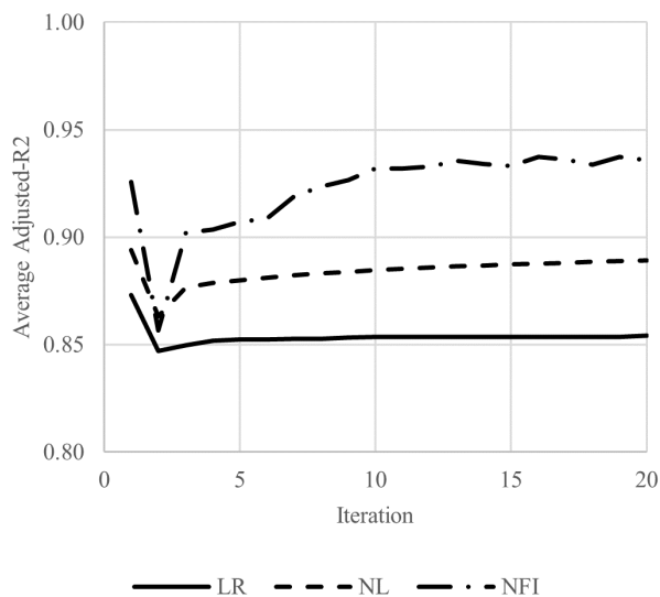
Figure 5: Model average adjusted-R 2
