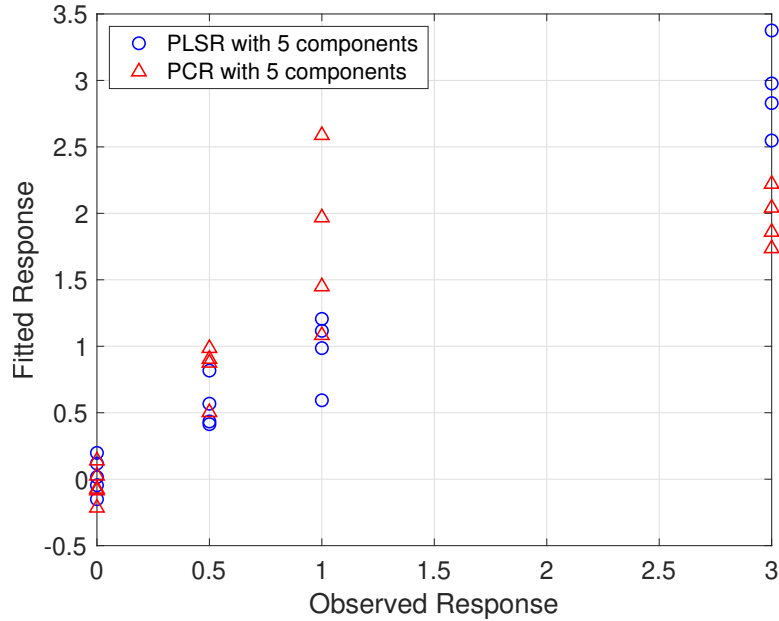
Figure 25. Comparison of measured and predicted Ga concentration using PCR and PLSR models.
