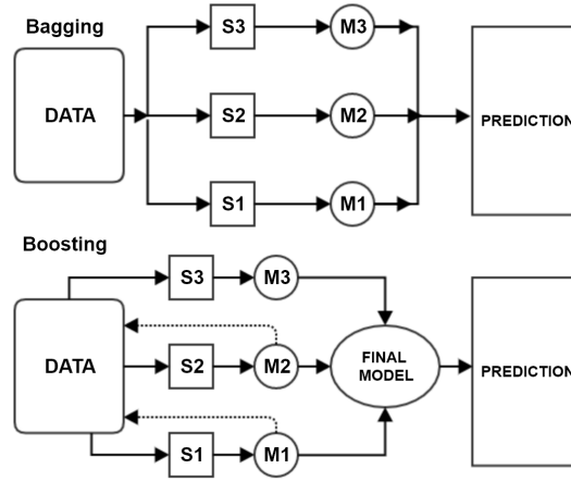
Figure 28. Comparison of bagging and boosting ensemble methods. Squares denoted by 'S' and 'M' represent data subsets and individual learner models trained on those subsets, respectively.
