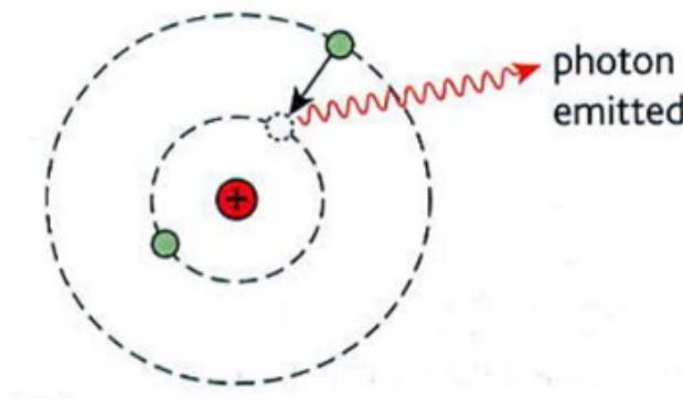
Figure 3. Basic rendering of the atomic de-excitation process [27].
