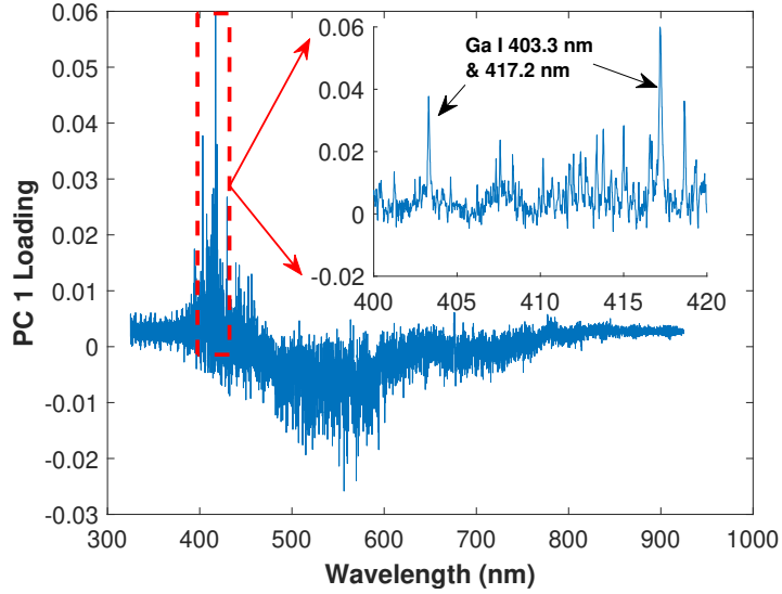
Figure 68. PC 1 loadings of each wavelength in the data. The two wavelengths corresponding to the strongest Ga I emissions load the highest, and therefore contribute to most of the total variance of the data.
