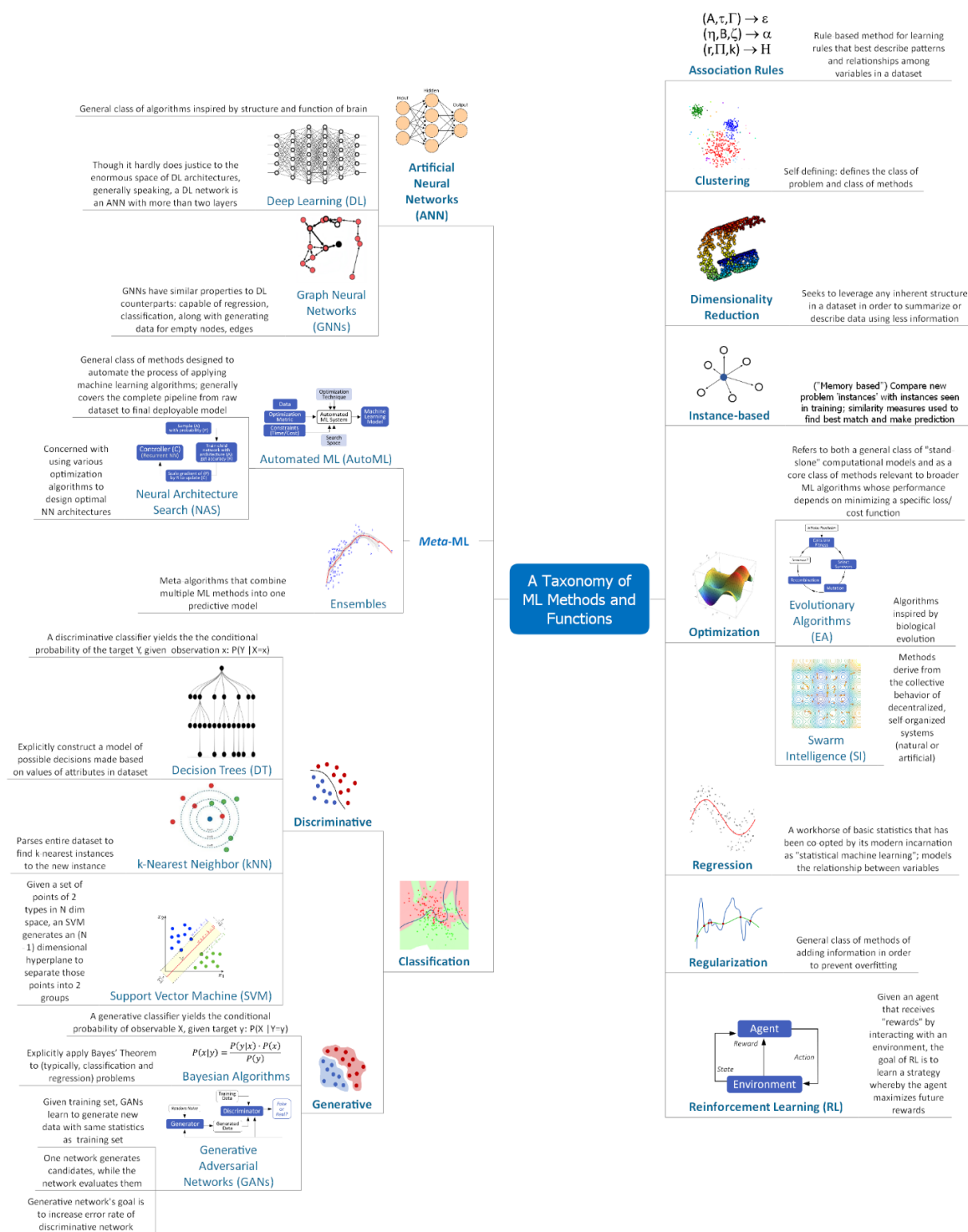
Figure 9. High level taxonomy of ML methods
