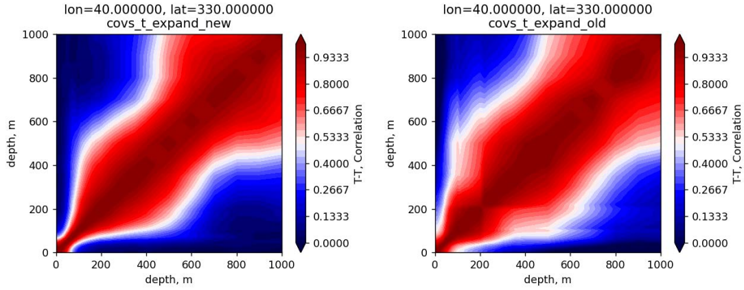
Figure B4. The temperature-temperature vertical covariance in the North Atlantic at 40^\circ , 30^\circ W, computed (left plot) using the smooth time search profile given in equation (B24). The plot on the right is from using the original, step function methods of equations (B23). The details of the covariance calculation are described in the next section.
