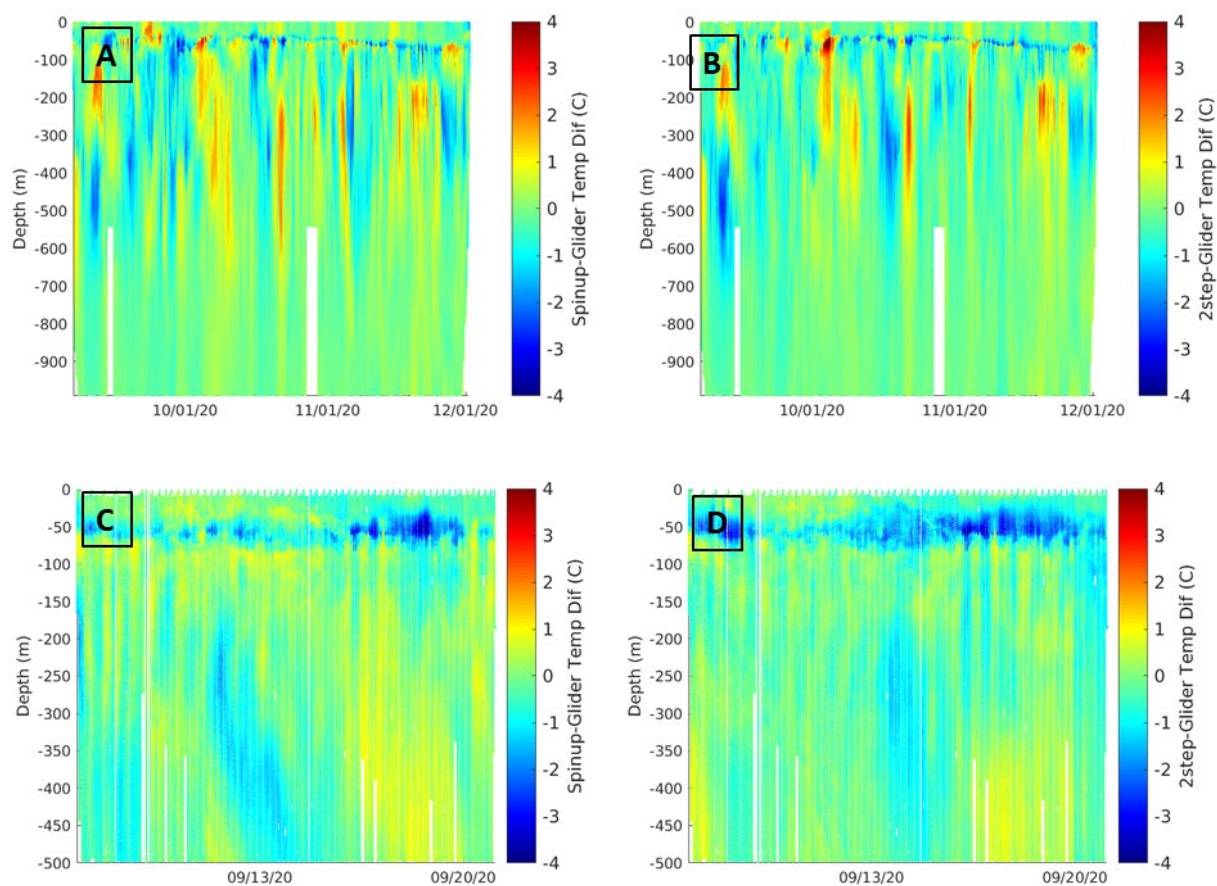
Figure 30. Temperature errors of Exp1 relative to gliders SG601 (A) and NG357 (C). Likewise for Exp2, the errors relative to gliders SG601 (B) and NG357 (D).
