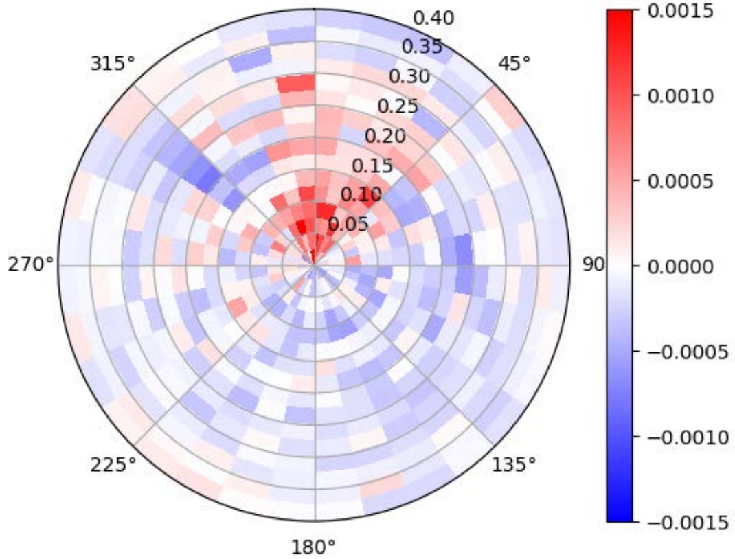
Figure 14. The probability density of the difference between the TWO-STEP minus the CNTRL test cases of the velocity magnitude (m/s) and direction ( ^{\circ} ) errors. 14-hour forecasts from both cases are compared over the same set of 130,188 observations.
