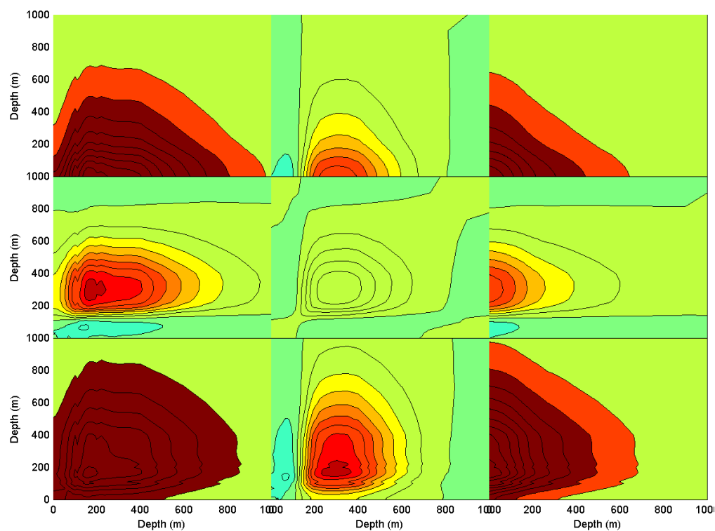
Figure C6. Cross covariance of T, S and \phi at 275°E, 24°N for January. This matrix is computed from the eigenvector and eigenvalue information stored in data files. Each month of the year is a separate file, and the eigen information is stored on a 0.5° grid covering the globe.
