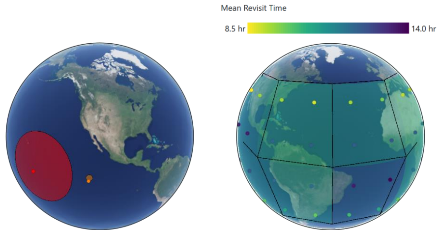
Figure 10 TAT-C simulation on satellite constellation observations (left) and computation on coverage statistics for regions of interest (right)
