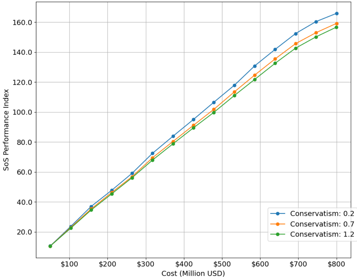
Figure 16 Initial results: cost vs. SoS performance
