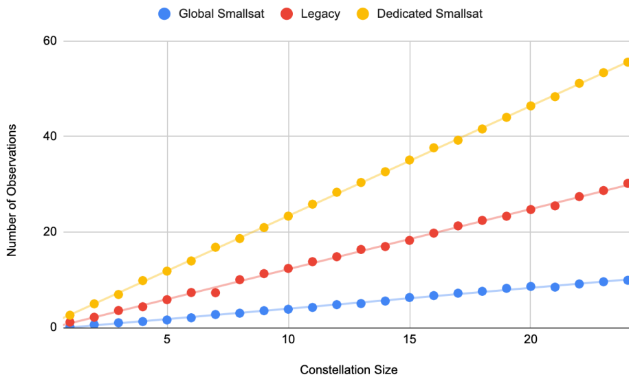
Figure 11 Coverage statistics for all three constellation types.
