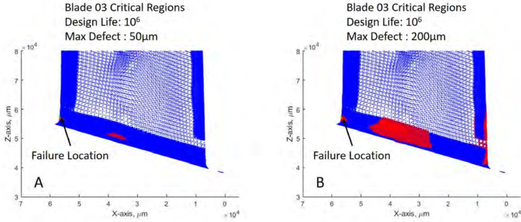
Figure 43. Critical failure locations for Turbine Blade 03 assuming A) A defect \leq 50\mu\text{m} causes failure and B) A defect \leq 200\mu\text{m} causes failure
