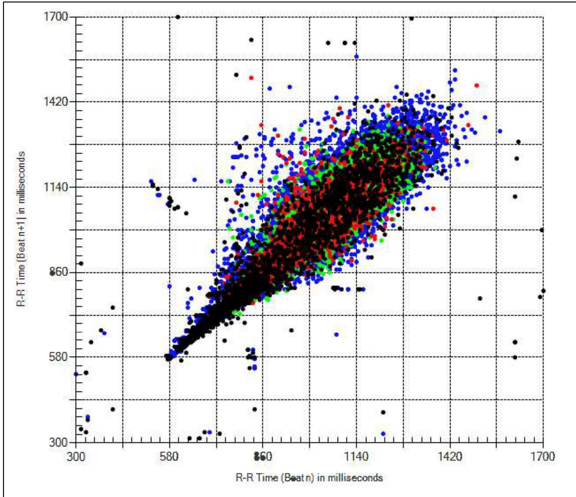
Figure 1. Poincaré plot example. Poincaré plot displaying heart rate variability over time. The RR interval, RR(n) is plotted over time as a function of the subsequent RR interval RR(n+1) .
