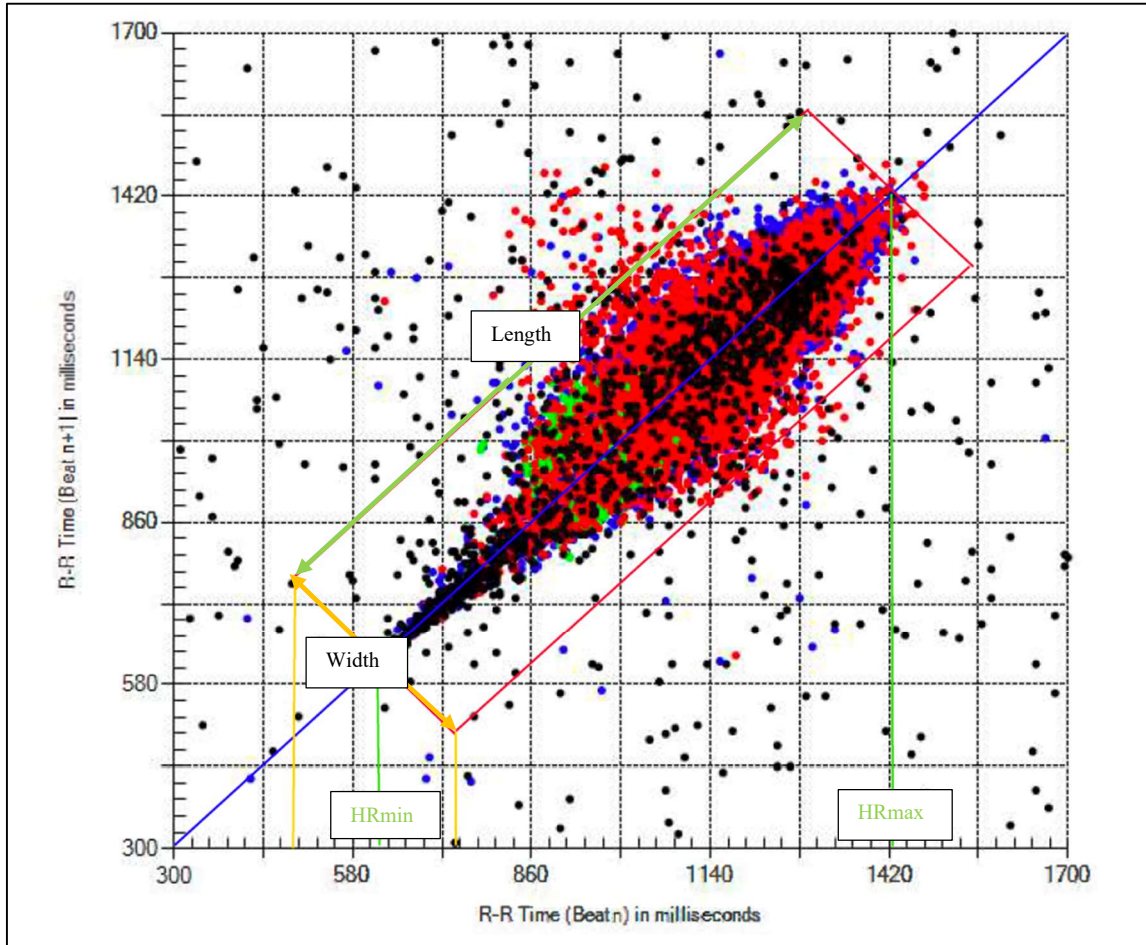
Figure 2. Poincaré plot analysis example. Example shown is a typical plot seen in the control group. Line of identity (blue). Length of the plot is measured along the line of identity (green) and width of the plot is measured from the perpendicular line crossing the line of identity (yellow). Square of the plot (red). Method adapted from (Chaidas et al., 2014; Mermigkis et al., 2009)
