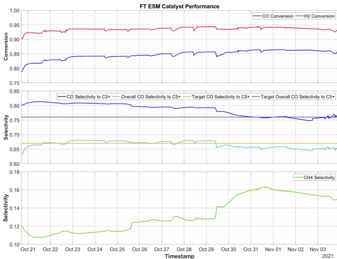
Figure 5. FT Catalyst Performance from October 21, 2021 to November 3, 2021
