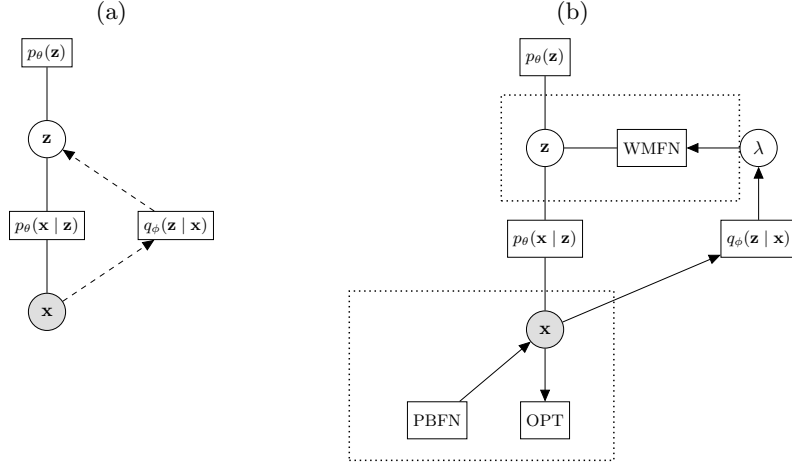
Fig. 2: Left (a): Latent variable model with conditional recognition factor. Note that the two unidirectional dashed arrows indicate that this model uses PySigma’s augmented factor graph semantics. Right (b): Compiled PySigma model of the Variational Autoencoder. The nodes grouped by a dashed rectangle together construct a predicate subgraph.
