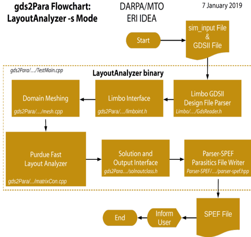
Figure 3: Flowchart of the gds2Para Tool
