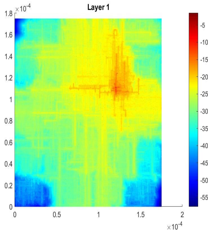
Figure 5: Voltage Distribution across the Chip of an ASAP 7 nm Design
