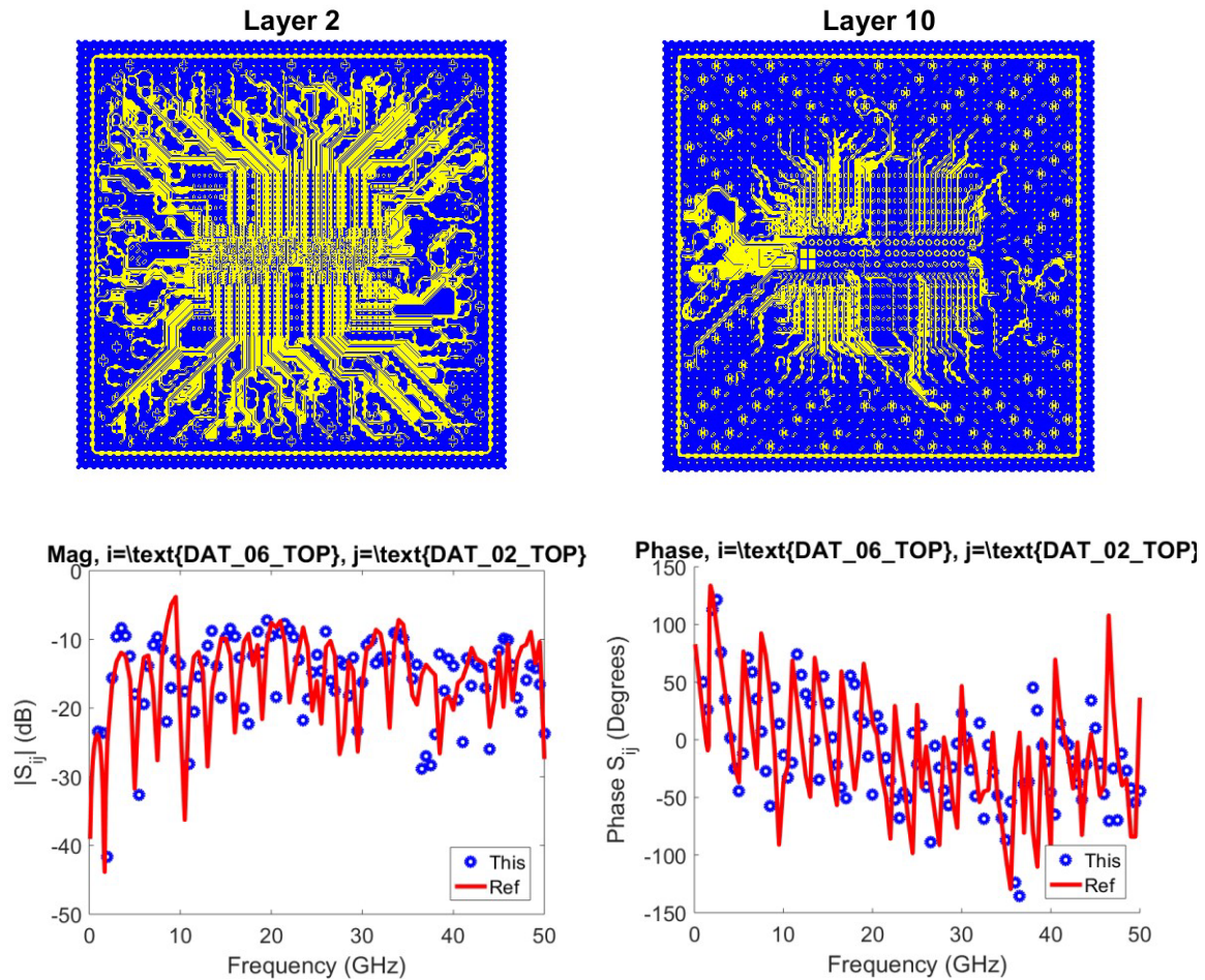
Figure 6: S-parameters Extracted from an IBM Package
