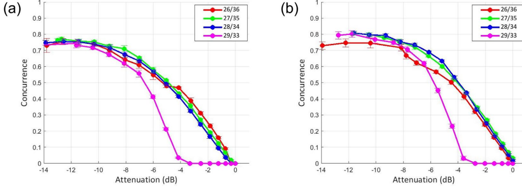
Fig. 2 Concurrence as a function of pump attenuation when the DSF is stored at (a) +20 °C and (b) -86 °C. The decrease in concurrence is seemingly due to spectral broadening of the pump caused by SPM. This decrease in concurrence is greatest for the inner-most channel pair (29/33) since that channel pair has the smallest detuning from the pump (Channel 31).
