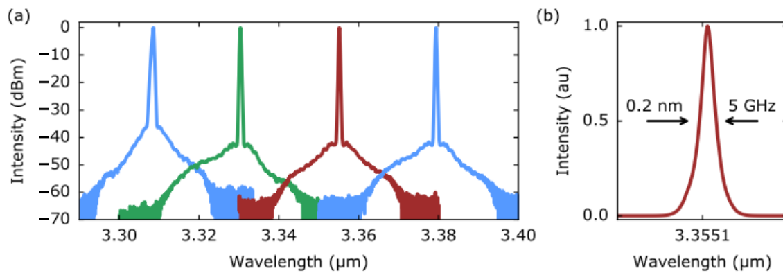
Figure 2 - Idler spectral tuning - note that the full tuning range is not shown due to the optical spectrum analyzers measurement range. (b) Example idler spectrum plotted on linear scale, with full-width half maximum spectral widths (wavelength and frequency) indicated, resolution limit of OSA was 0.1 nm.
