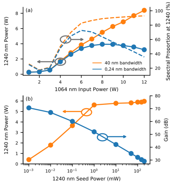
Figure 9 - (a) Calculated phosphosilicate Raman fiber amplifier output power (points) and percentage spectral content (dashed lines) as a function of input 1064 nm power for a 40 nm (orange) and 0.24 nm (blue) integration bandwidth at 1240 nm. (b) Generated 1240 nm power (orange) and phosphosilicate Raman fiber amplifier gain (blue) as a function of seed power, for an Yb: fiber MOPA power of 8 W
