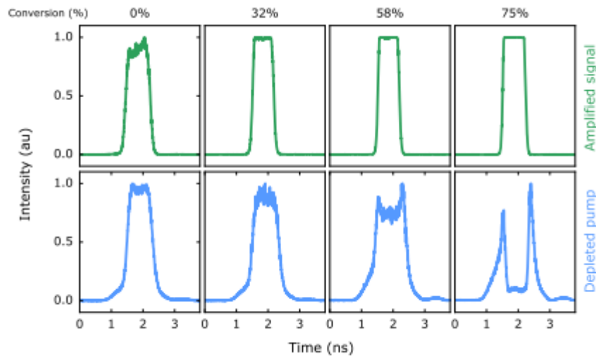
Figure 5 - Sampling optical oscilloscope traces of signal and pump for increasing levels of pump conversion, from 0% to 75%, after undergoing parametric conversion in PPLN. Signal pulses shown on top row in green, with corresponding pump pulses on the bottom row in blue. All pulse amplitudes are normalized.
