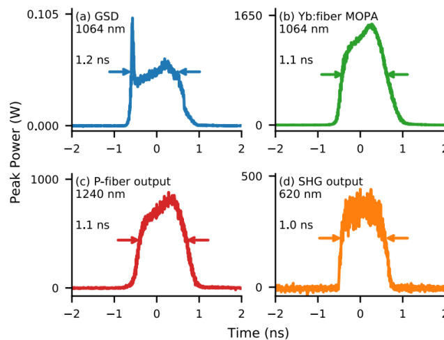
Figure 8 - Temporal profiles of the output pulses of the (a) 1064 nm gain-switched laser diode (GSD), (b) Yb: fiber MOPA, (c) phosphosilicate fiber (P-fiber) amplifier, and (d) 620 nm SHG output from the PPLT crystal. The full-width-half-maximum (FWHM) pulse duration is indicated in each case.
