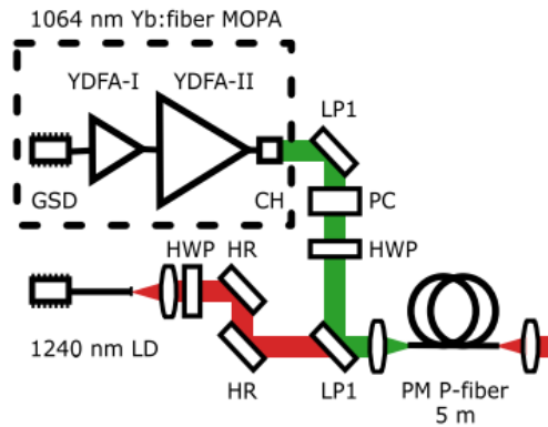
Figure 7 - 1240 nm phosphosilicate Raman fiber - GSD, gain-switched laser diode; YDFA-I, Yb-doped fiber pre-amplifier; YDFA-II, Yb-doped fiber power amplifier; CH, collimator head; LD, laser diode; P-fiber, phosphosilicate fiber; HWP, half-wave plate; PC, power control, formed of half-wave plate and polarizing beam splitter cube; HR, highly reflective mirror at 1240 nm; LP1, longpass filter (cut-on 1150 nm).
