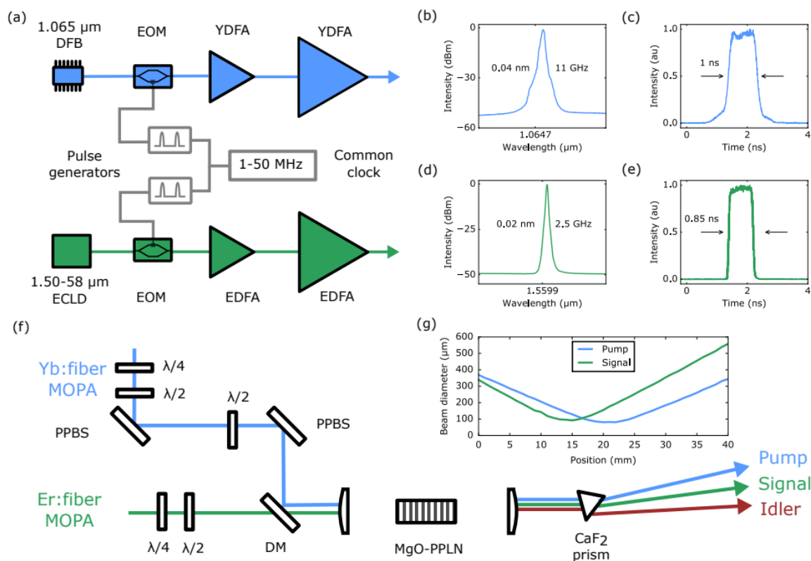
Figure 1 - Master oscillator power amplifiers (MOPAs) used for mid-infrared (mid-IR) generation, component acronyms are described in the body of the main text. (b)/(d) Example spectral and (c)/(e) temporal outputs of the Yb/Er:MOPAs. Labels show the full-width half maxima (FWHM) in wavelength, frequency and time domains respectively. MOPA output characteristics presented here represent those for optimal high average power mid-IR generation. (f) Mid-IR parametric conversion stage. The two MOPAs were combined in a 40 mm long MgO-doped periodically poled lithium niobate (MgO-PPLN) crystal. Crystal held in an insulated copper oven at temperatures from 20–230°C. (g) Measured pump and signal beam caustics in air, at the focal position of crystal.
