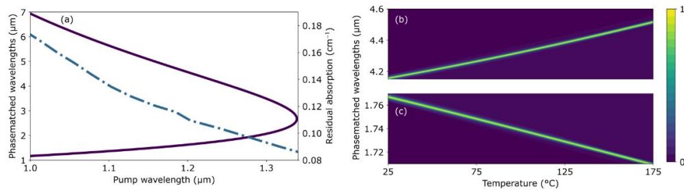
Figure 11 - (a) Phase-matched signal and idler wavelengths for non-critical 90° type-I (oo-e) in CSP, purple solid line. Residual absorption of CSP as a function of pump wavelength, dashed-dotted blue line. (b) Phase-matched idler and signal (c) wavelengths against crystal temperature, colorbar indicates the theoretical conversion efficiency.
