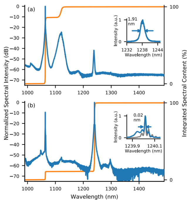
Figure 10 - Spectra of the phosphosilicate Raman fiber amplifier output for a 1064 nm input power of 8 W where (a) no seed light is present and (b) 200 mW of seed power are coupled into the phosphosilicate fiber. The orange lines show the integrated spectral content as a function of wavelength. Insets show optical spectrum of the generated 1240 nm light (blue) and 1240 nm seed diode (gray) on a linear scale.
