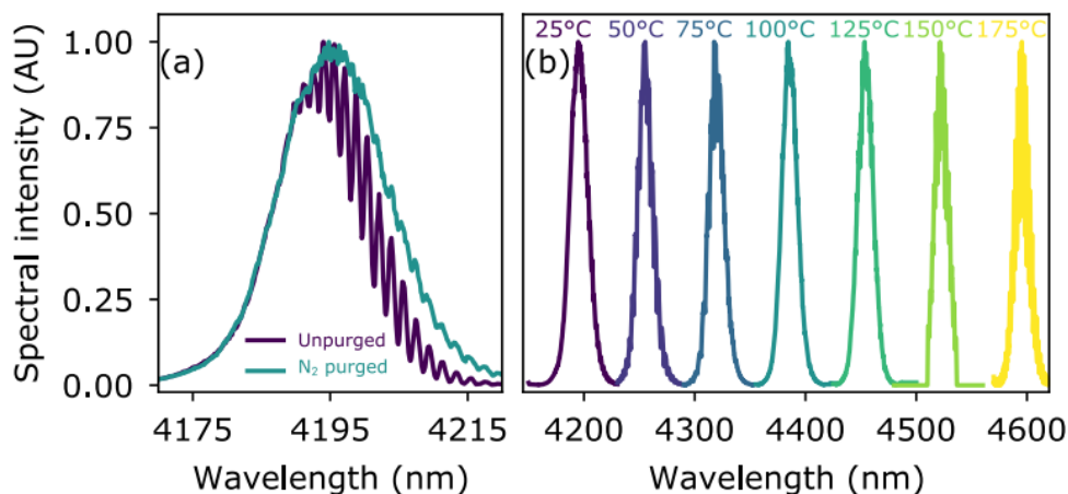
Figure 16 - (a) Example MIR idler spectrum at 25°C, in both the unpurged and N 2 purged case. (b) Wide idler wavelength tuning possible through temperature tuning the CSP crystal.
