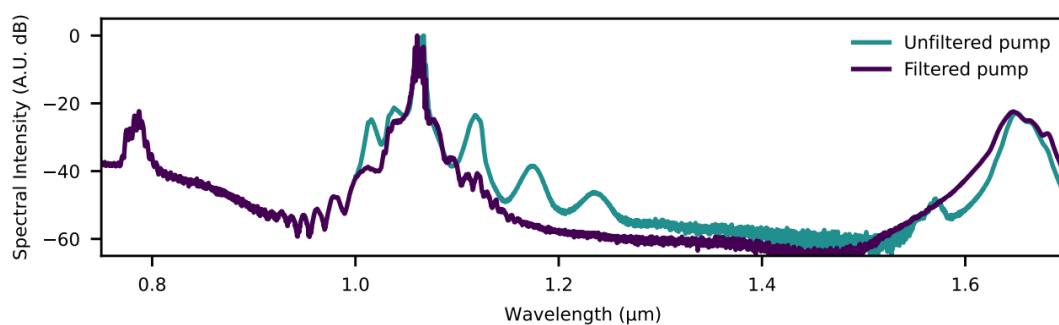
Figure 20 - Spectrum at output of PCF. With and without long pass 1100 nm filtering of the pump source to remove Raman scattered light.
