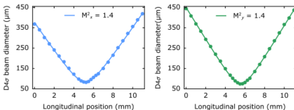
Figure 4 - Measured beam diameter ( D4\sigma widths) of the idler in the horizontal and vertical beam axis through the focus of a lens, with a Gaussian fit to the beam caustic. Taken at full power and measured using a pyroelectric scanning slit beam profiler.
