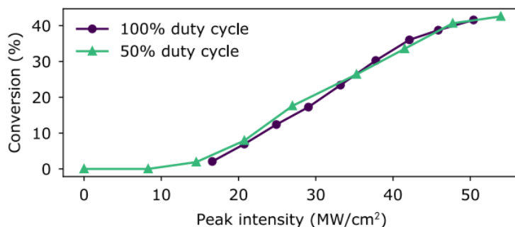
Figure 15 - Total pump conversion (combined signal plus idler) at different duty cycles. \lambda_s = 1.76 \mu\text{m} and \lambda_i = 4.20 \mu\text{m} .
