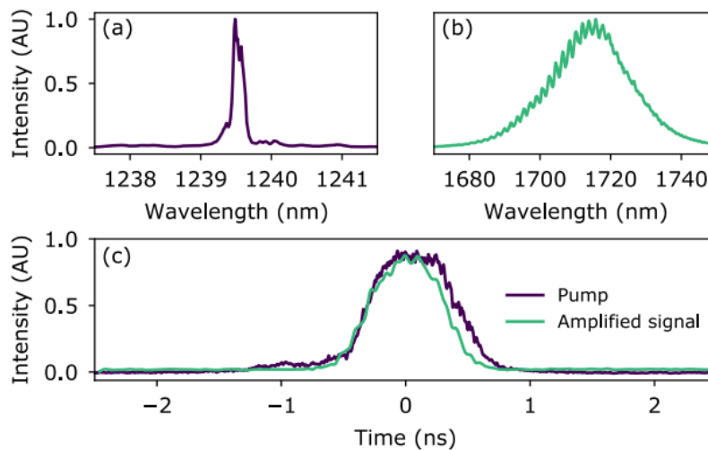
Figure 13 - a) Optical spectrum of Raman fiber amplifier pump pulses, and (b) continuous-wave filtered fiber supercontinuum signal seed. (c) Temporal profiles of pump and amplified signal pulses.
