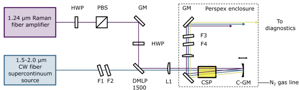
Figure 12 - Experimental setup for seeded optical parametric in CSP. The 1.24 \mu\text{m} Raman fiber amplifier acts as the pump with a continuous wave fiber supercontinuum source providing the seed signal, pumping the CSP crystal in a double pass configuration to generate idler radiation in the 4.2–4.6 \mu\text{m} band.
