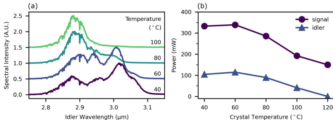
Figure 22 - (a) Idler wavelength tuning with temperature. (b) Generated idler and amplified signal power tuning with temperature.
