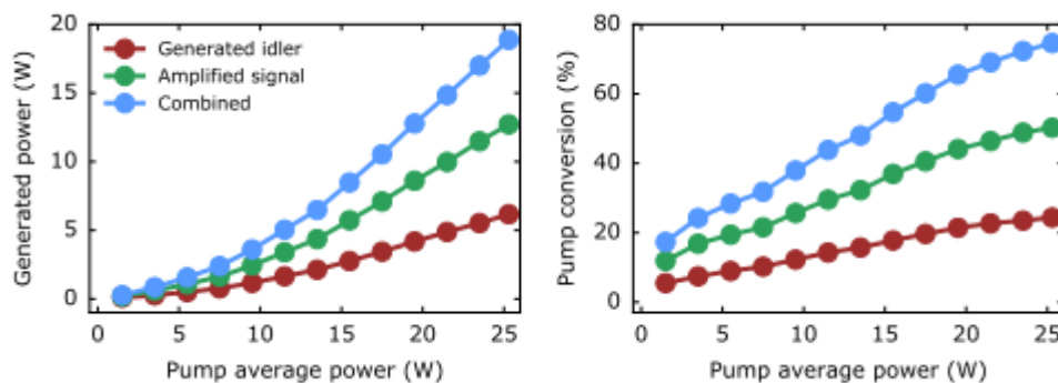
Figure 3 - (a) Example amplified signal (green), generated idler (red) and combined (blue) powers produced during parametric conversion. (b) Typical pump conversion to the signal, idler and combined wavelengths.
