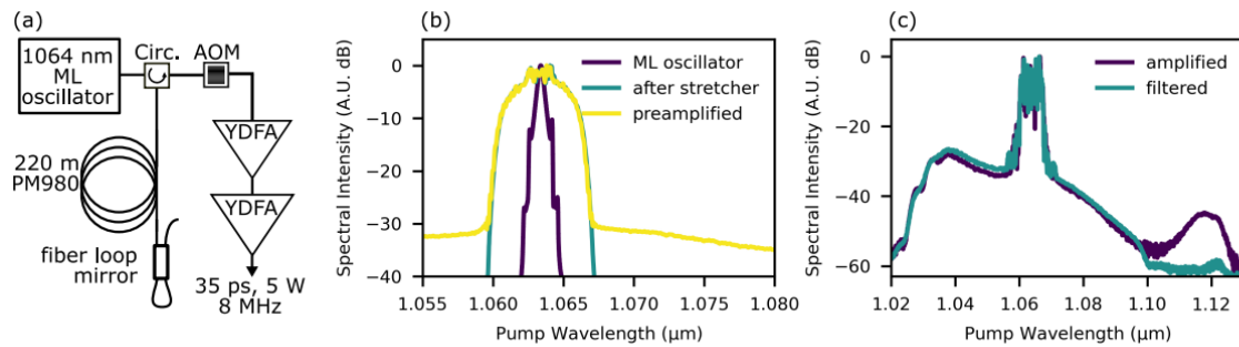
Figure 19 - Ytterbium fiber master oscillator power amplifier (MOPA) system. ML, mode-locked; Circ., Fiber circulator; AOM, acousto-optic modulator; YDFA, ytterbium-doped fiber amplifier. (b, c) Pump laser spectra at different positions along the MOPA chain.
