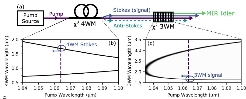
Figure 18 - (a) Schematic of MIR generation via cascaded \chi^{(3)} four wave mixing (4WM) and \chi^{(2)} three wave mixing (3WM). (b) Phase matching diagrams for the 4WM in PCF and (c) 3WM in PPLN (at 60°C).
