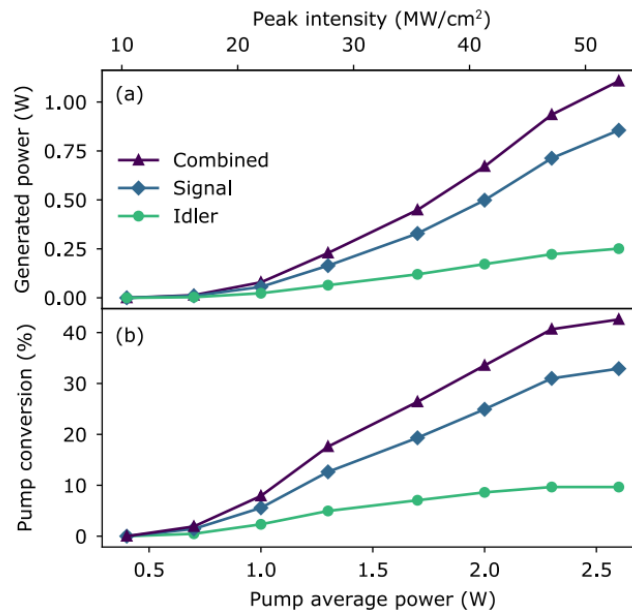
Figure 14 - (a) Signal, idler, and combined (signal plus idler) average powers against pump average power (bottom axis)/pump peak intensity in the crystal (top axis). (b) The corresponding pump conversion into the signal, idler, and combined (signal plus idler). \lambda_s = 1.76 \mu\text{m} and \lambda_i = 4.20 \mu\text{m} .
