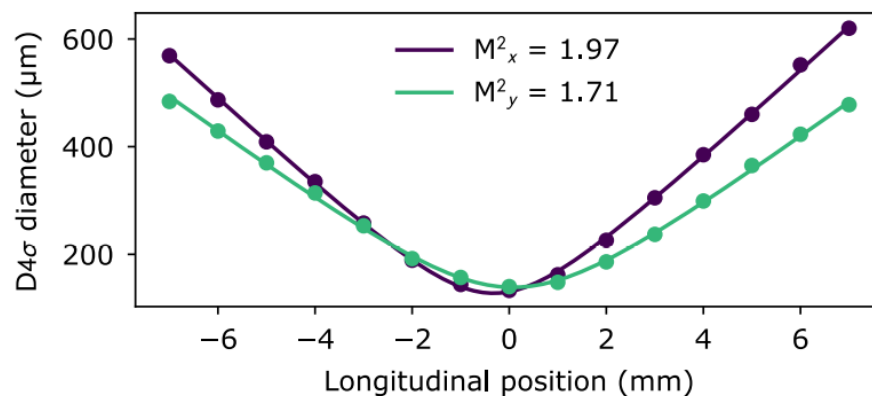
Figure 17 - Measured beam diameter ( D4\sigma widths) of the idler in the horizontal ( x ) and vertical ( y ) beam axis through the focus of a lens measured using a pyroelectric scanning slit beam profiler, with a Gaussian fit to the beam caustic.
