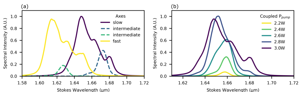
Figure 21 - (a) Generated Stokes sidebands on the fast and slow axes, and at intermediate positions between the principle axes. (b) Generated Stokes sidebands variation with coupled pump power on the fast axes.
