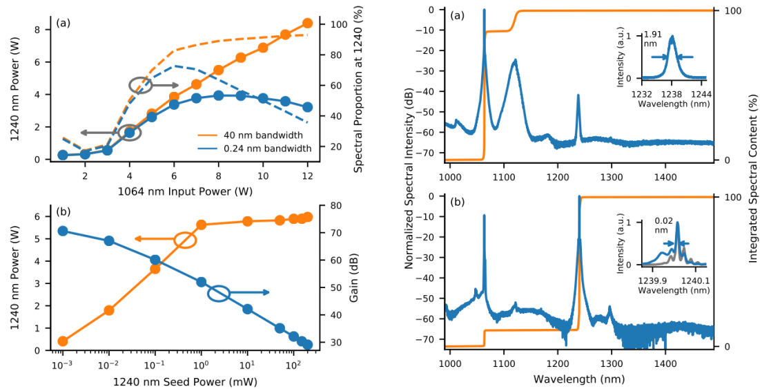
Figure 6 - (a) Calculated phosphosilicate Raman fiber amplifier output power (points) and percentage spectral content (dashed lines) as a function of input 1064 nm power for a 40 nm (orange) and 0.24 nm (blue) integration bandwidth at 1240 nm. (b) Generated 1240 nm power (orange) and phosphosilicate Raman fiber amplifier gain (blue) as a function of seed power, for an Yb: fiber MOPA power of 8W. Spectra of the phosphosilicate Raman fiber amplifier output for a 1064nm input power of 8W where (a) no seed light is present and (b) 200 mW of seed power are coupled into the phosphosilicate fiber. The orange lines show the integrated spectral content as a function of wavelength. Insets show optical spectrum of the generated 1240 nm light (blue) and 1240nm seed diode (gray) on a linear scale.
