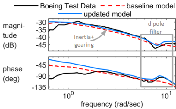
Figure 7.2.3-1: Boeing Flight-Test Data and CAE Simulation Pitch Responses.
