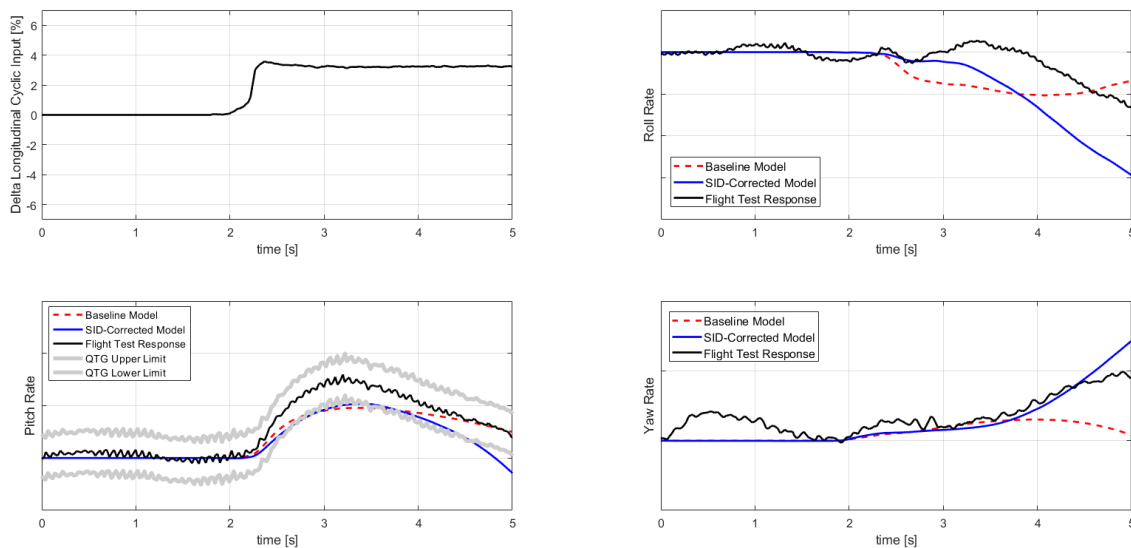
Figure 7.3.3-9: Response to Aft Longitudinal Step Input in Hover.
