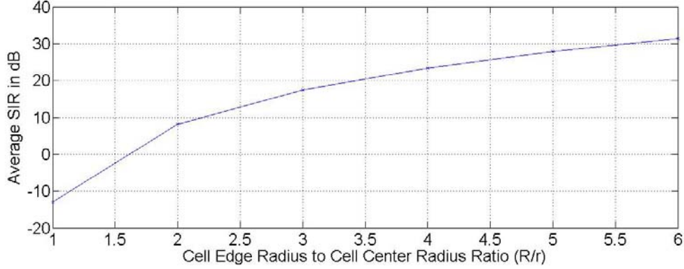
Figure 38. Reverse channel average SIR as a function of the ratio of R/r (120°-sectoring).
