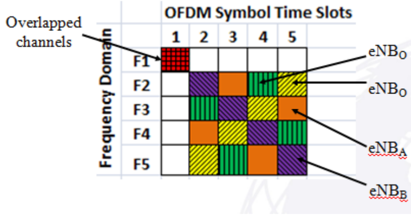
Figure 33. Mapped matrices.
