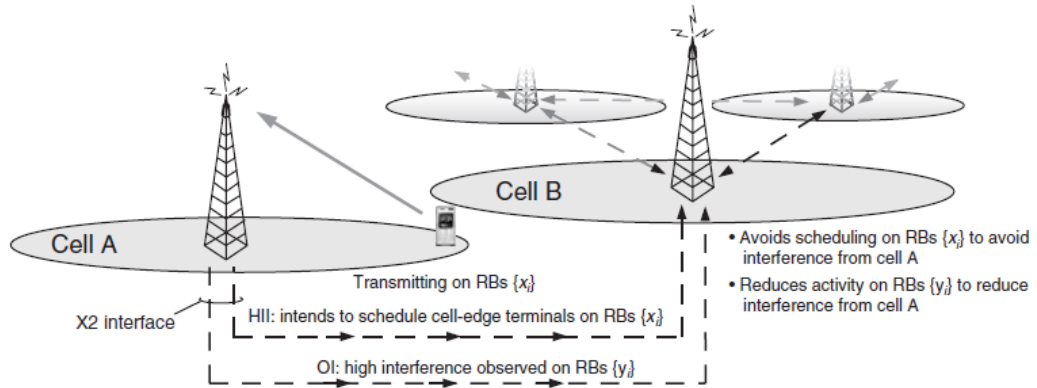
Figure 6. Example of uplink co-channel interference coordination. From [19].
