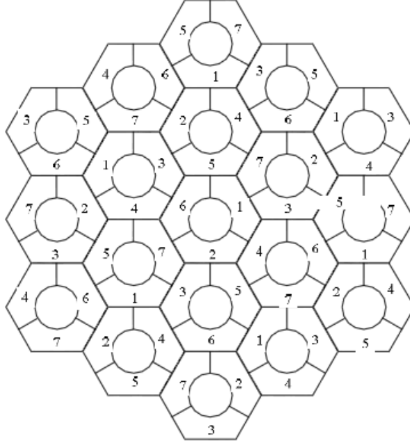
Figure 5. Frequency reuse scheme of Network Power Planning scheme. From [2].
