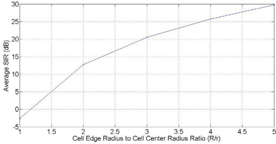
Figure 37. Forward channel average SIR as a function of the ratio of R/r (120°-sectoring).
