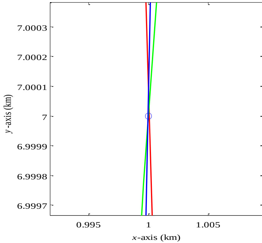
Figure 3. Three sensors obtain an error of 0.1 meters when attempting to geolocate an emitter.
