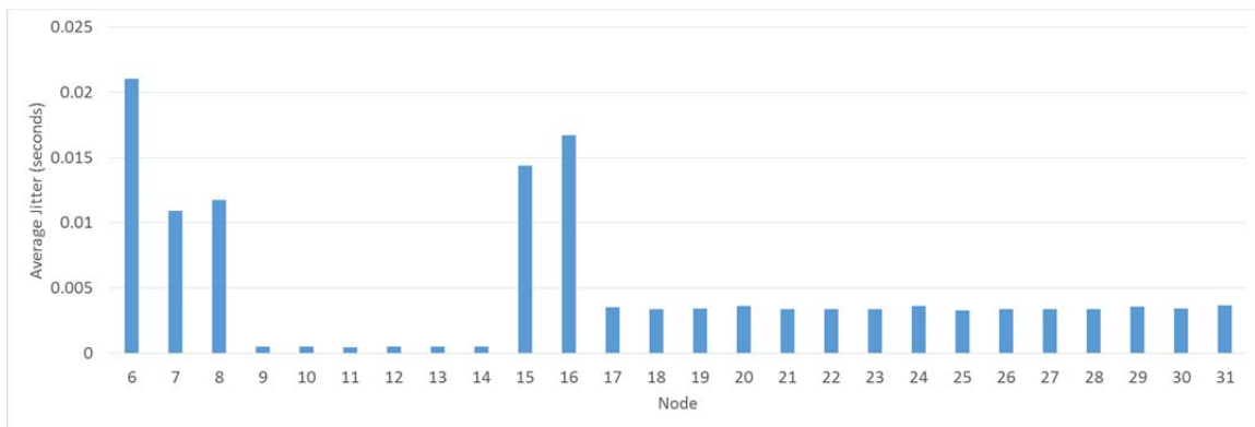
Figure 107. Average Jitter for 5.5-Mbps Data Rate in Scenario I
