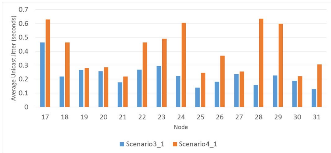
Figure 72. Average Jitter Time Comparison for Scenario III and IV
