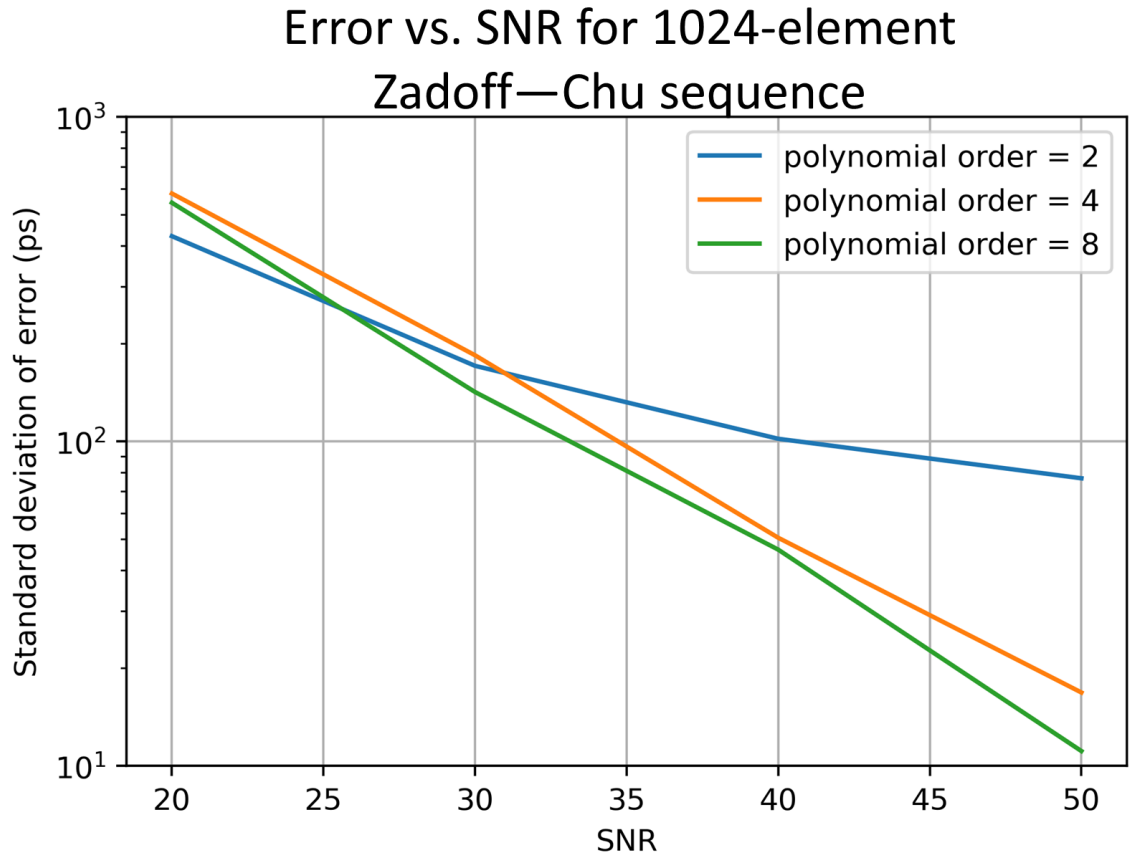
Fig. 3 Standard deviation of arrival time error vs. signal-to-noise in decibel ratio for 1024-element Zadoff—Chu sequence. The three traces show computational results with different orders of polynomial interpolation.
