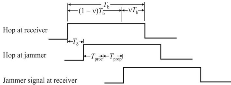
Figure 3.3. Frequency Hopping Follower Jamming. Source: [58].
