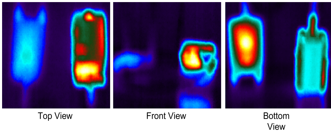
Figure 7.7. Thermal Test Two: Mode ON, During Operations (5 Minutes Active).
