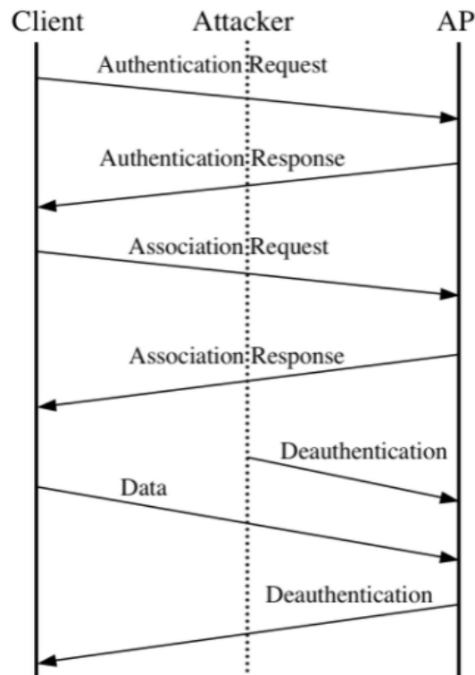
Figure 4.7. Deauthentication Attack. Source: [102].
