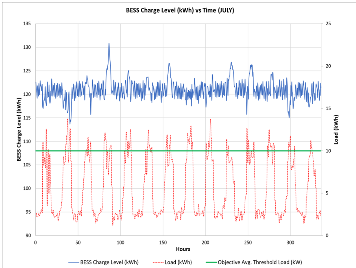
Figure 2.9. This figure shows a snapshot of a single run of the system over the 14 day period of analysis using July GHI input data. The green line represents the design objective threshold load. As seen, the load often exceeds this during peak work hours. The BESS is able to handle the load and the PV and EDG are able to recharge sufficiently to avoid load shed (BESS reaches zero). The difference from Figure 2.8 is that the BESS is maintaining a higher charge level throughout the period of analysis due to the increased PV output from the increased solar irradiance in July.
