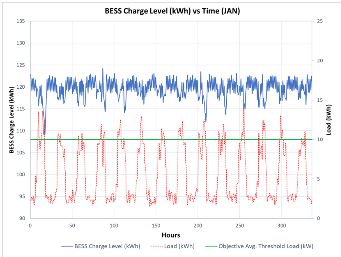
Figure 2.8. This figure shows a snapshot of a single run of the system for the 14 day period of analysis using January GHI input data. The green line represents the design objective threshold load. As seen, the load often exceeds this during peak work hours due to the stochastic nature of the model. The BESS is able to handle the load and the PV and EDG are able to recharge sufficiently to avoid load shed (BESS reaches zero).
