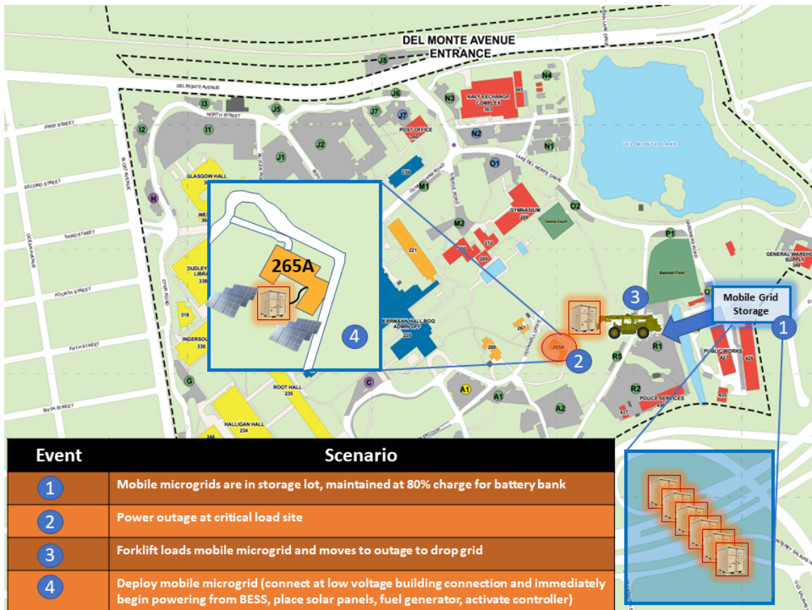
Figure 2.3. Mobile Microgrid CONOPS for NSA Monterey Backup Power: This CONOPS for installation critical load backup power shows a simple step by step process for employing the mobile microgrid to restore power to a critical load. Power can be restored very quickly after the mobile microgrid is co-located with the critical load because the system provides power from the BESS. Workers can then position the PV array while the load is powered with the BESS, within safety requirements, because the mobile microgrid is a low voltage (48V) system.
