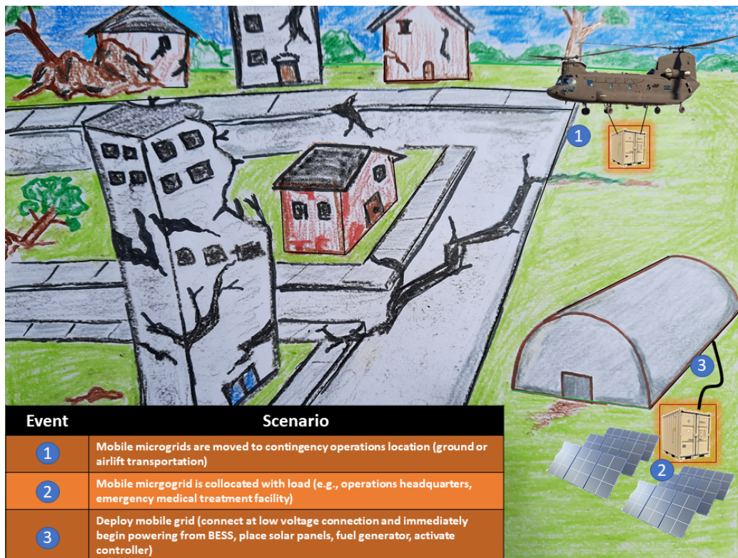
Figure 2.4. Mobile Microgrid CONOPS for Contingency Operations: This CONOPS for contingency operations shows a mobile microgrid being airlifted to the contingency environment and collocated with an operations headquarters. The load can be powered from the BESS immediately after the mobile microgrid is dropped at the site. Workers can then position the PV array while the load is powered with the BESS, within safety requirements, because the mobile microgrid is a low voltage (48V) system.
