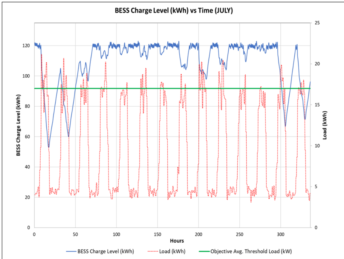
Figure 2.11. This figure shows a snapshot of a single run of the system over the 14 day period of analysis using July GHI input data but a much larger load than was designed for. The green line represents the increased average load of 17 kW. As seen, the load often exceeds this during peak work hours. The difference between this figure and Figure 2.10 is that the PV is now able to recharge at a sufficient rate to prevent a slow draw down of the BESS and prevent load shed.
