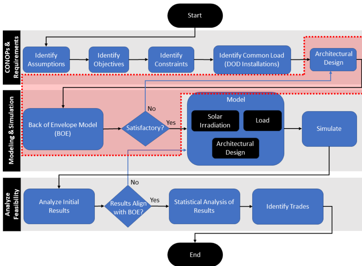
Figure 2.7. Mobile Microgrid SE Process Model that highlights the iterative process to develop the architectural design. Shown in red is the design loop that was used to refine the architectural design using COTS products for use in modeling and simulation.
