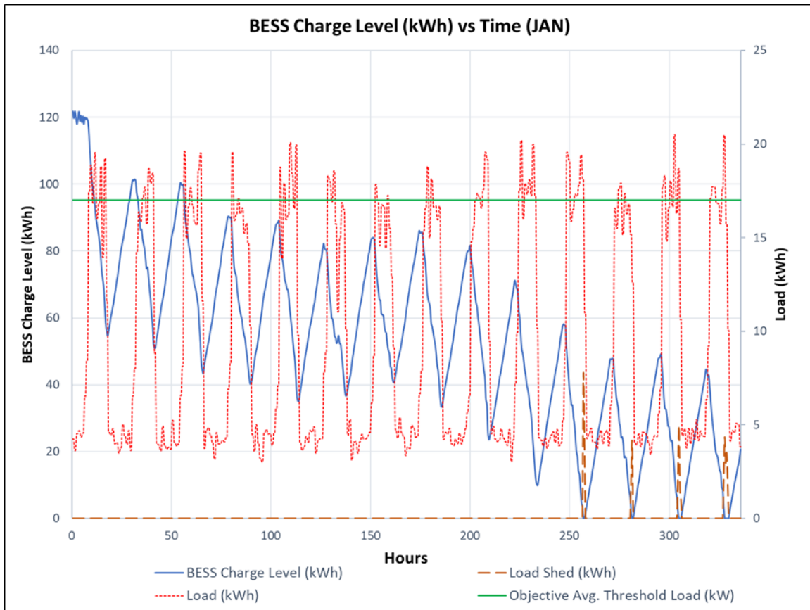
Figure 2.10. This figure shows a snapshot of a single run of the system over the 14 day period of analysis using January GHI input data but a much larger load than was designed for. The green line represents the increased average load of 17 kW. As seen, the load often exceeds this during peak work hours. Because the BESS capacity was designed to provide 1.5 days of storage for an average 10 kW load, it is able to meet the load for the majority of the period of analysis. However, the PV and EDG are not able to recharge sufficiently to avoid load shed as seen by the dotted dark red line spikes representing load shed at the far right of the graph.
