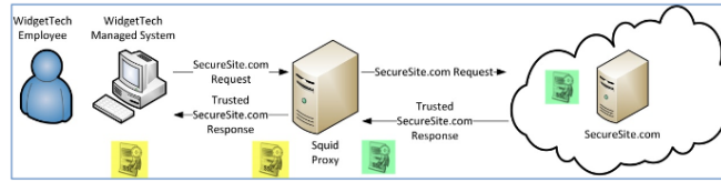
Figure 2.5. Traffic Inspection at Squid Proxy Server. Source: [6]
