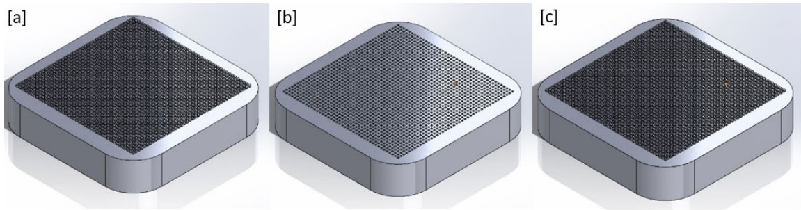
Figure 15. Flat plate sample with 100 \mu m cubic pillar surface finish (a), flat plate sample with 100 \mu m cubic indentations on surface (b), and flat plate sample with alternating 100 \mu m cubic pillar and indentations along surface (c)
