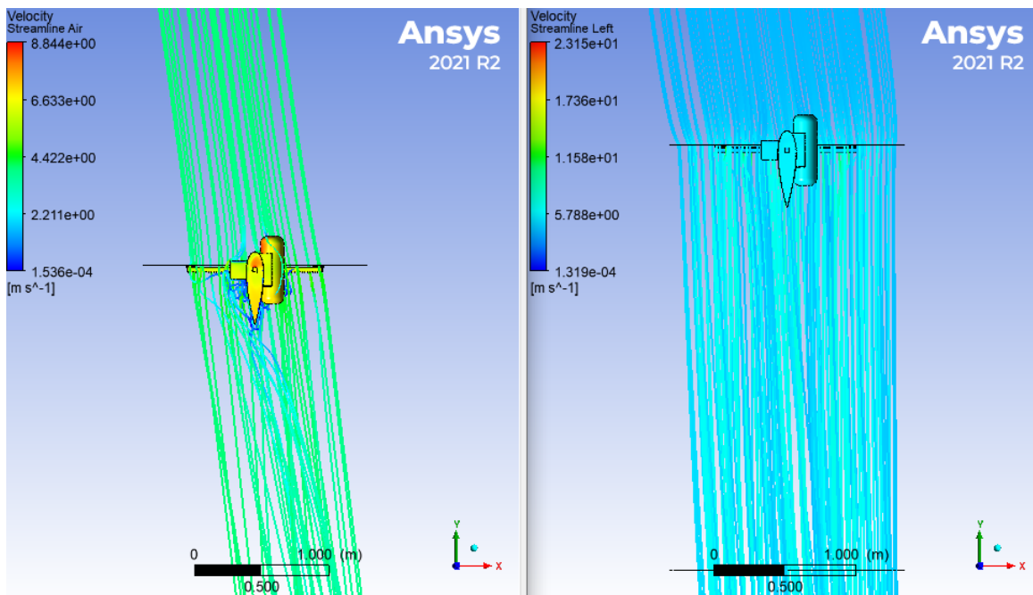
Figure 61. Flying Wing in 4 m/s 8^\circ \epsilon Streamlines
