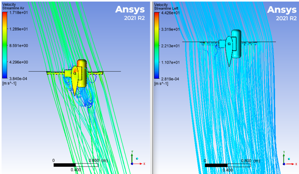
Figure 62. Flying Wing in 8 m/s 16^\circ \epsilon Streamlines
