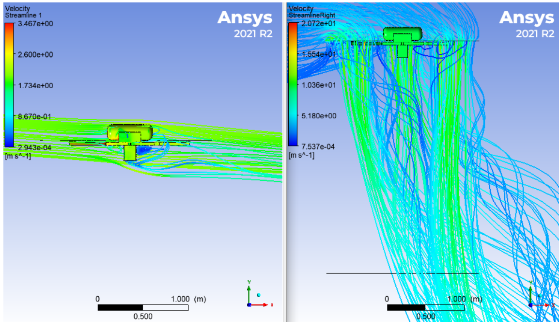
Figure 48. COTS 2 m/s 4° \epsilon Streamlines
