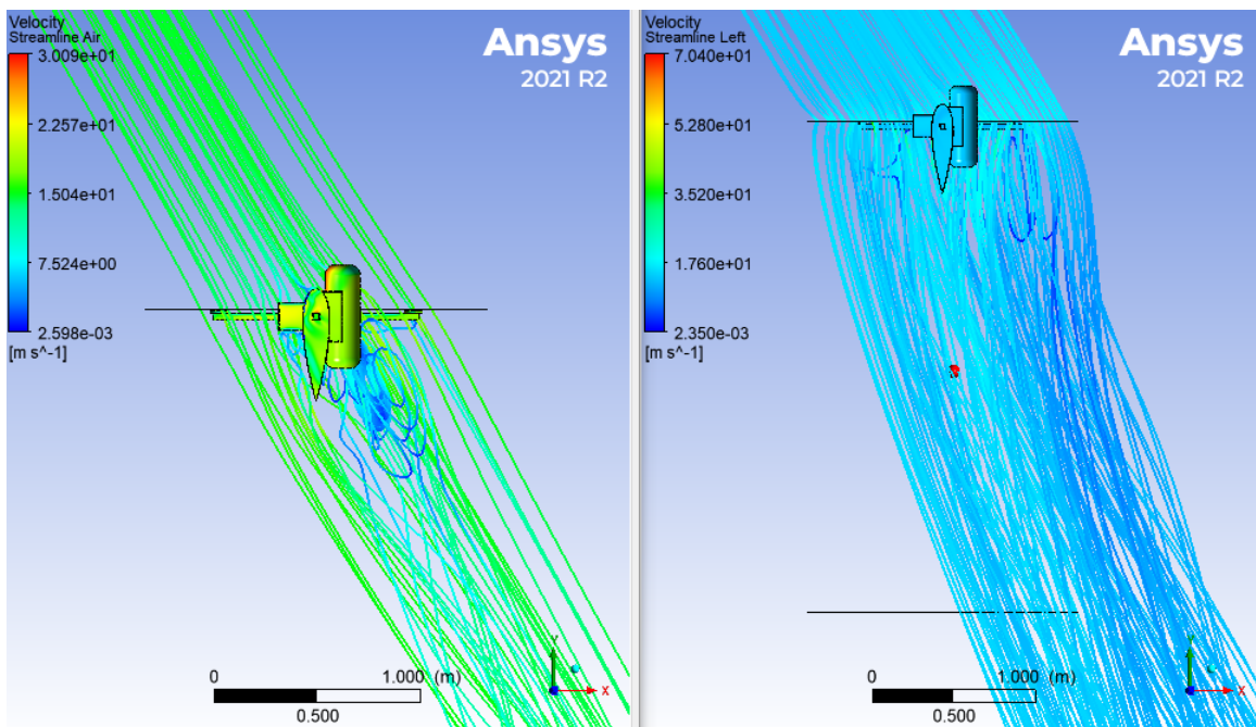
Figure 63. Flying Wing in 15 m/s 30^\circ \epsilon Streamlines
