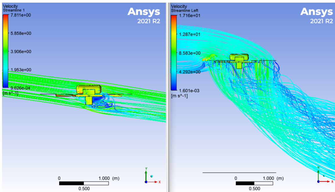
Figure 49. COTS 4 m/s 8° \epsilon Streamlines
