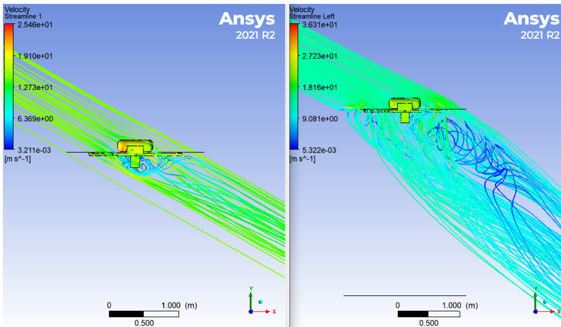
Figure 51. COTS 15 m/s 30^\circ \epsilon Streamlines
