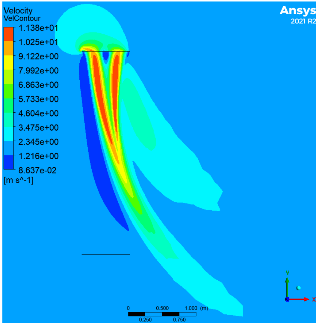
Figure 26. 2 m/s 4° \alpha Velocity Contour Plot
