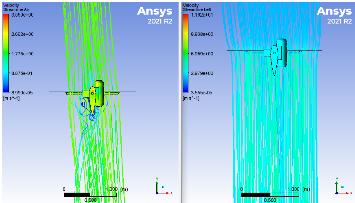
Figure 60. Flying Wing in 2 m/s 4^\circ \epsilon Streamlines
