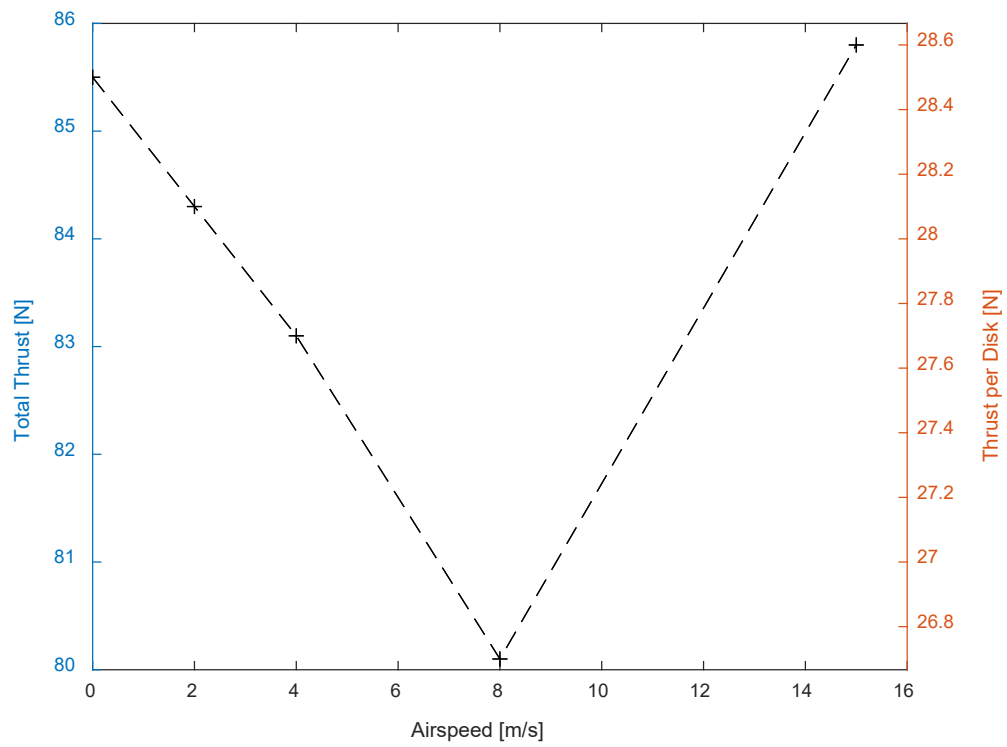
Figure 46. COTS CFD Predicted Thrust Results
