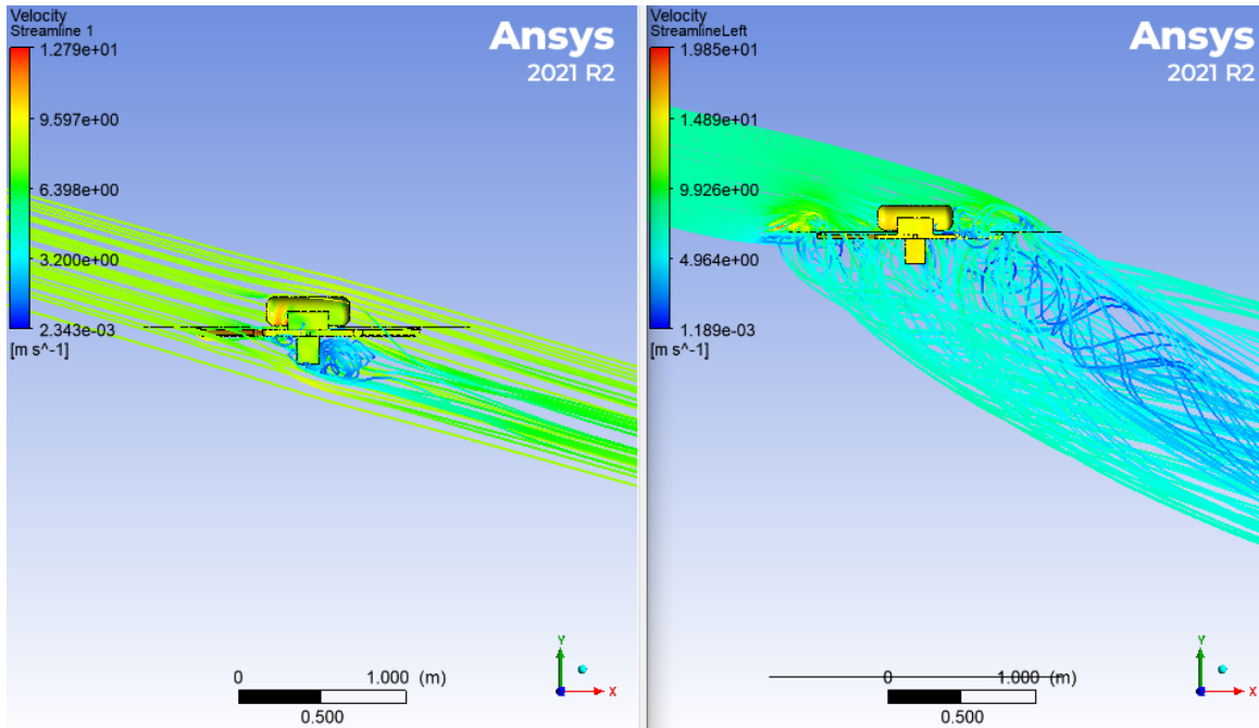
Figure 50. COTS 8 m/s 16^\circ \epsilon Streamlines
