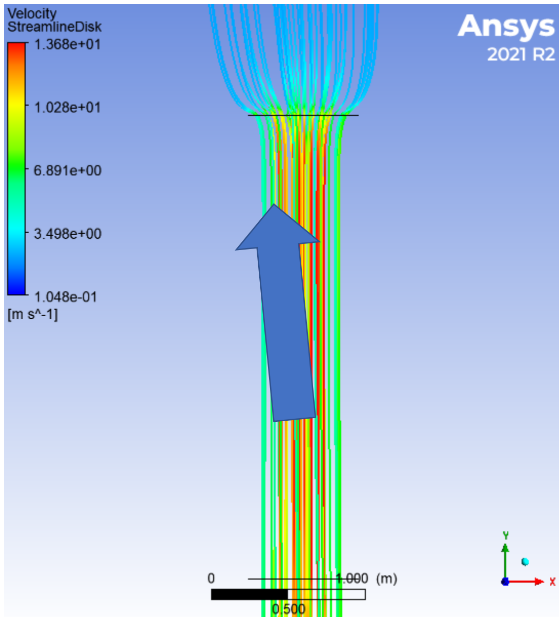
Figure 29. 2 m/s 86^\circ \alpha Streamlines
