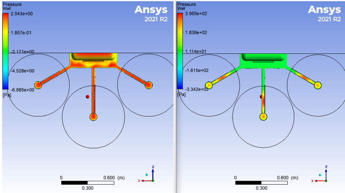
Figure 42. COTS 2 m/s Vertical Climb Pressure Distributions
