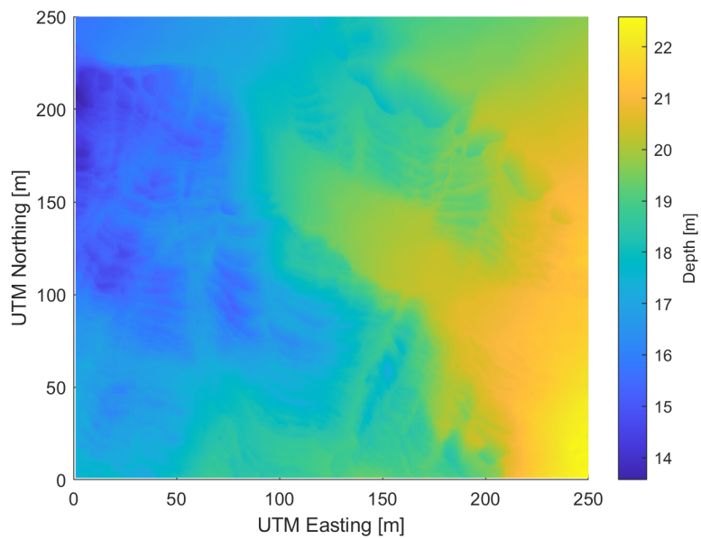
Figure 5.3. Monterey Bay Bathymetry Map
