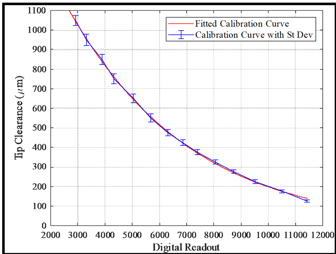
Figure 82. Calibration Curve, BCTR (Tip Gap Casing), Mid-Chord Probe 4.
