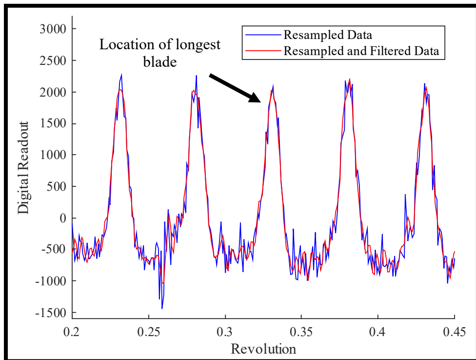
Figure 42. Filtered Data Comparison for 1050 μm (0.0413").
