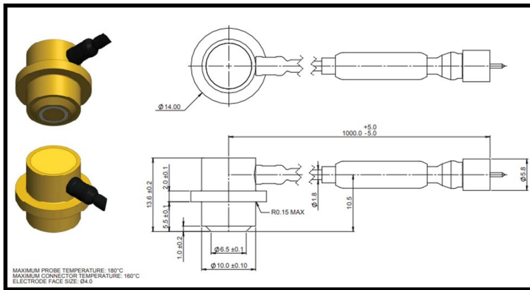
Figure 89. Capacitive Probe Dimensions (Units in mm). Source: [29].
