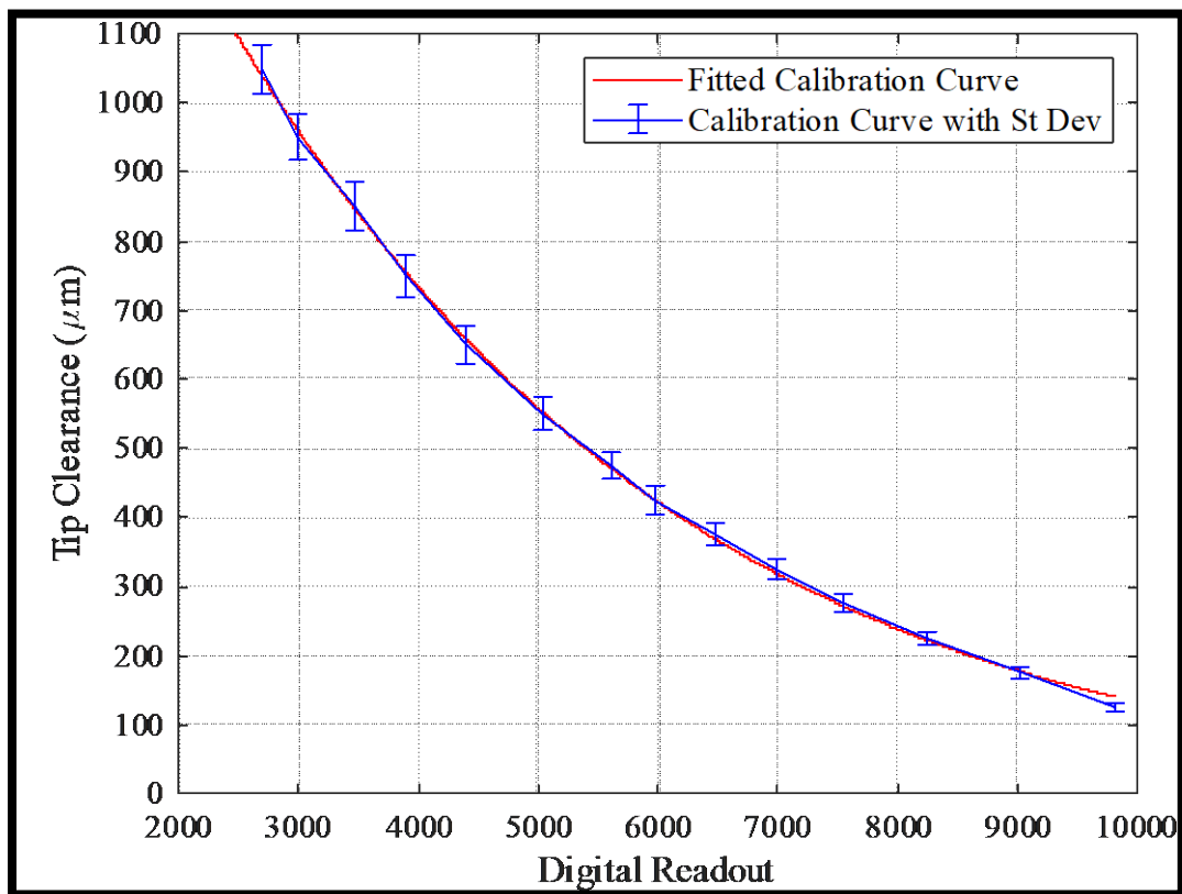
Figure 86. Calibration Curve, BCTR (Tip Gap Casing), Trailing Edge Probe
