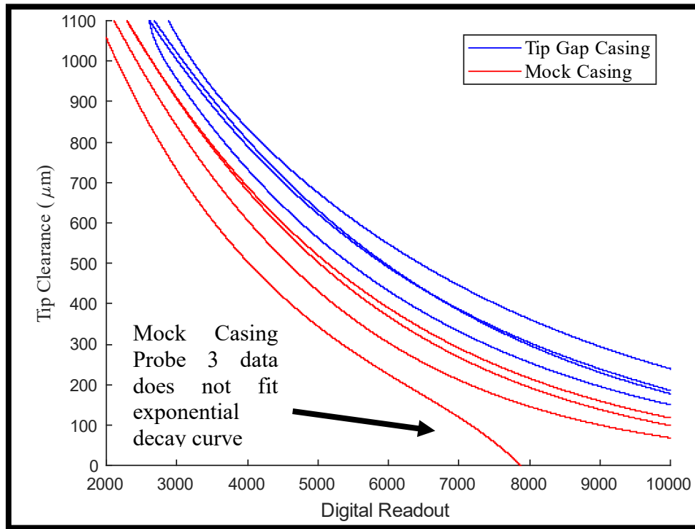
Figure 54. Mock Casing to Tip Gap Casing Comparison, Leading Edge.
