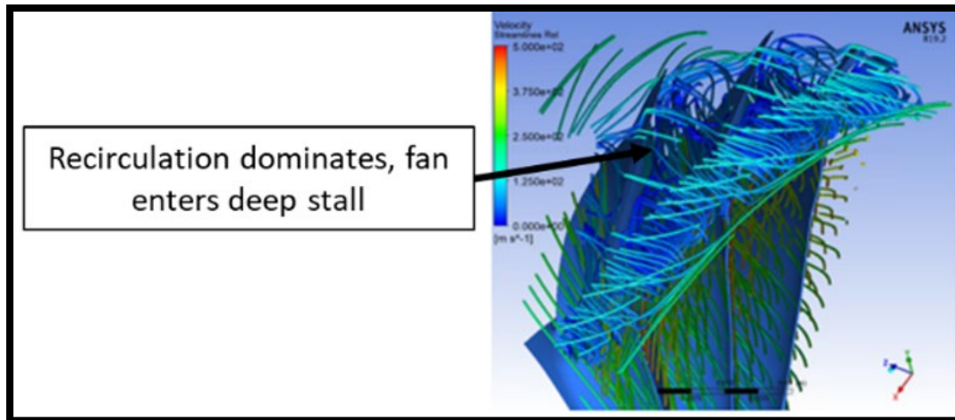
Figure 9. Simulated Tip Vortex from a Wide Tip Clearance for the NPSMF. Source: [20].
