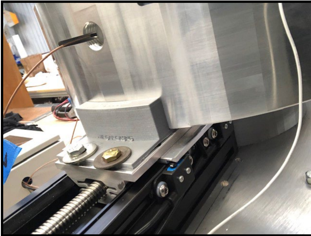
Figure 108. BCTR (Tip Gap Casing) Front Casing Grip Mount.
