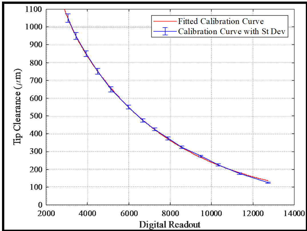
Figure 77. Calibration Curve, BCTR (Tip Gap Casing), Leading Edge Probe 3.
