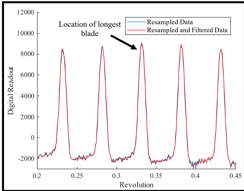
Figure 41. Filtered Data Comparison for 125 μm (0.00492").
