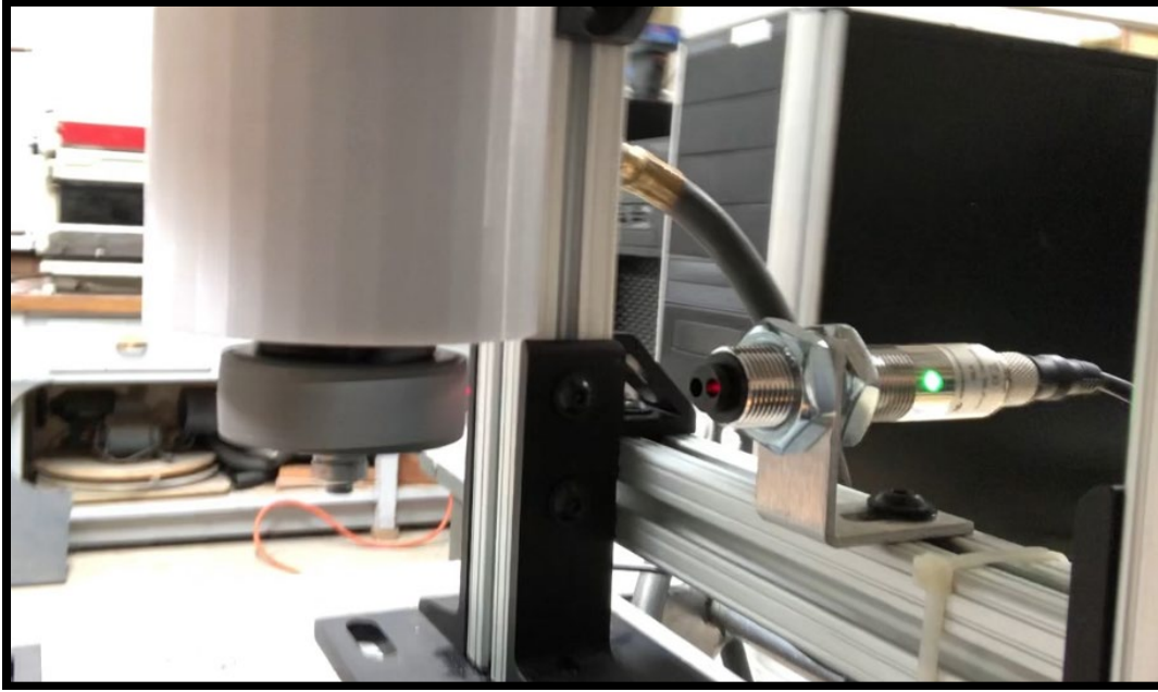
Figure 19. RLS Tachometer.
