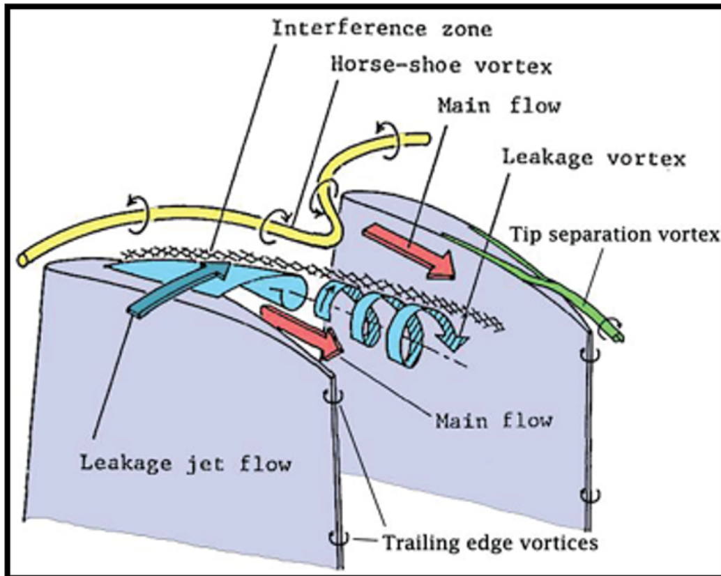
Figure 3. Secondary Flows Occurring in a Compressor Stage. Source: [6].
