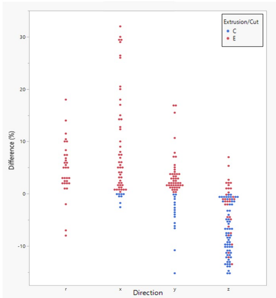
Figure 23. Directionality Based Errors. Extrusion/Cut is also Shown. Source: [20].
