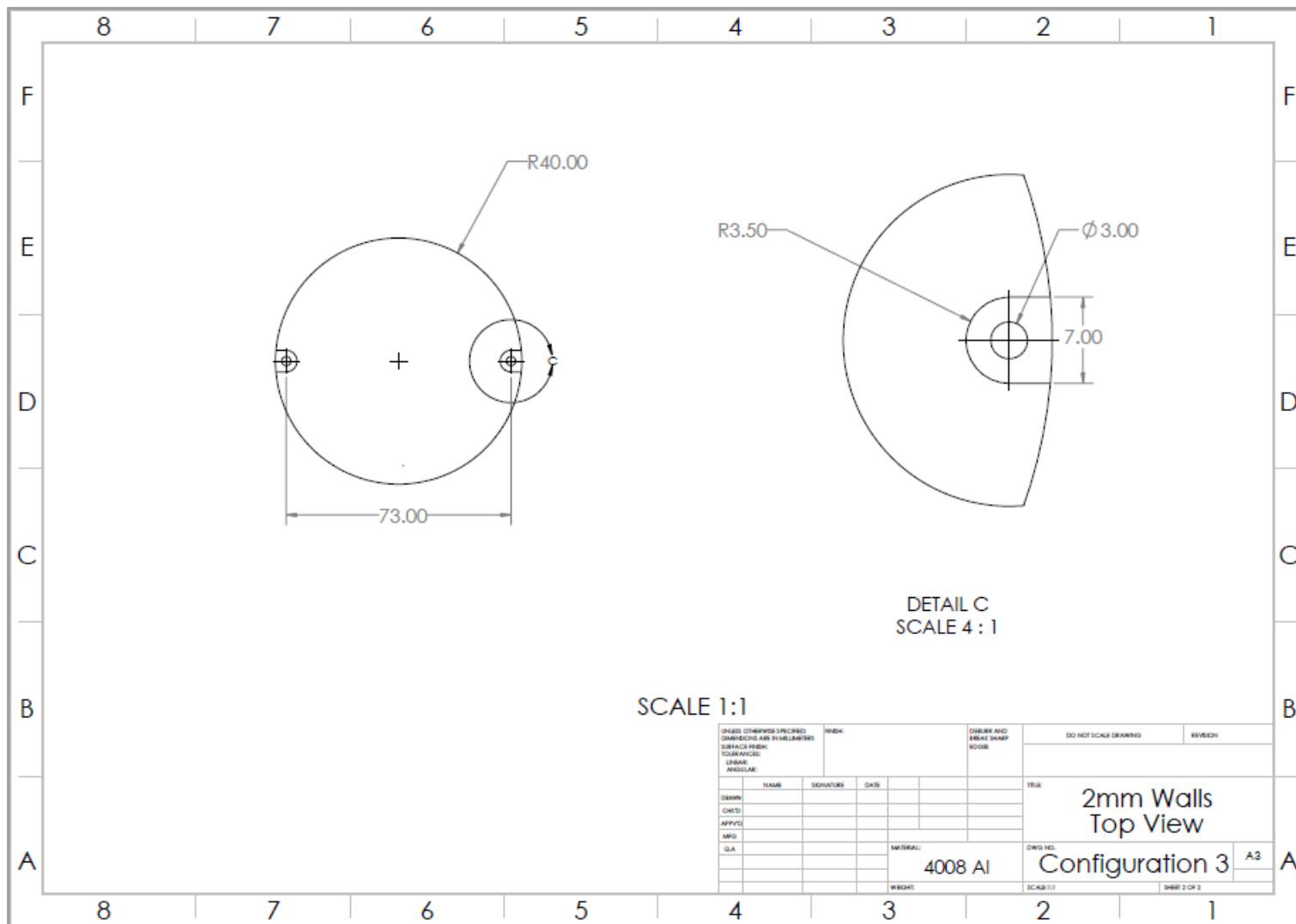
Figure 63. Configuration 3 Top View
