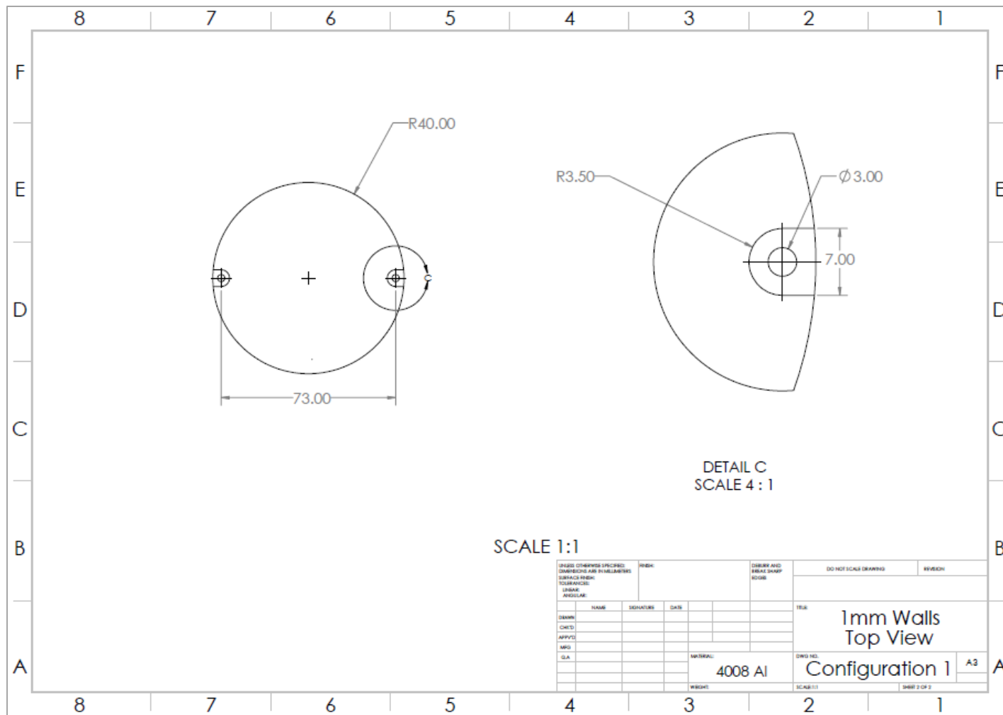
Figure 59. Configuration 1 Top View
