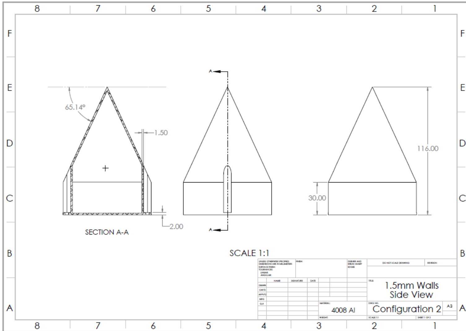
Figure 60. Configuration 2 Side View
